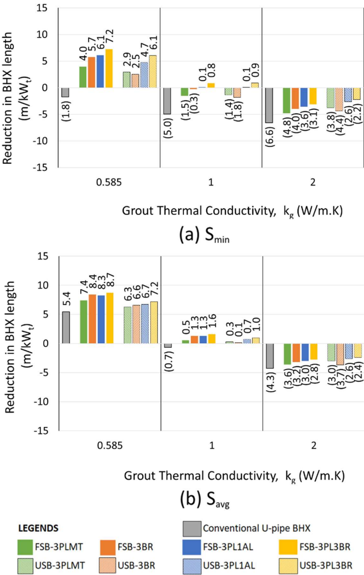
Figure 26. Reduction in length for various arrangements of U-tube BHx compared to coaxial pipes; k_s : 1 W/m.K, (a) S_{min} (b) S_{avg} .
