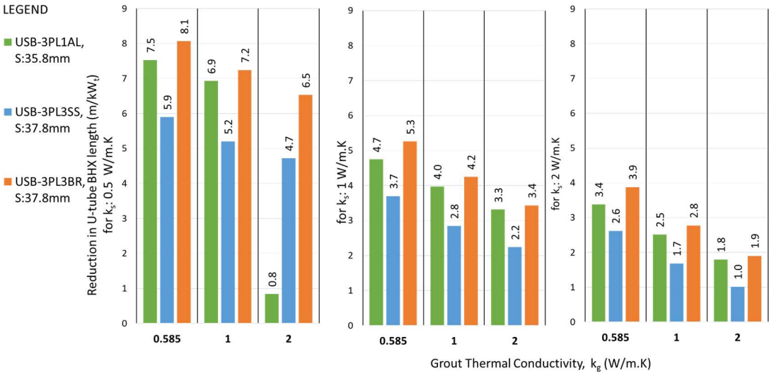
Figure 23. Reduction in the BHx length for various U- barriers; k_s: 0.5 \text{ W/m.K} .
