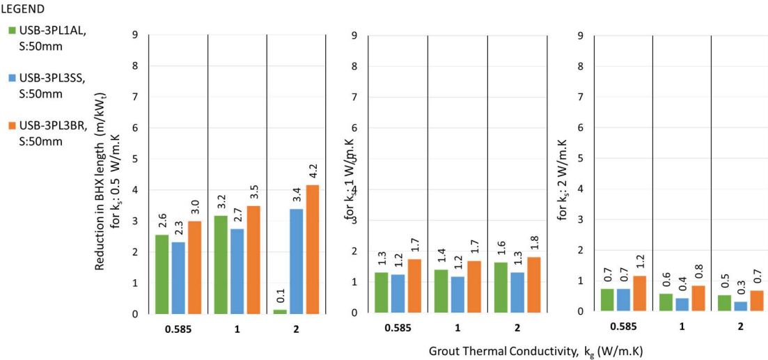
Figure 24. Reduction in the BHx length for various U- barriers; k_s: 2 \text{ W/m.K} .
