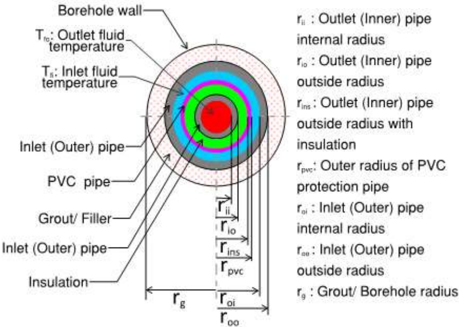
Figure 6. Insulated Coaxial pipes model geometry.
