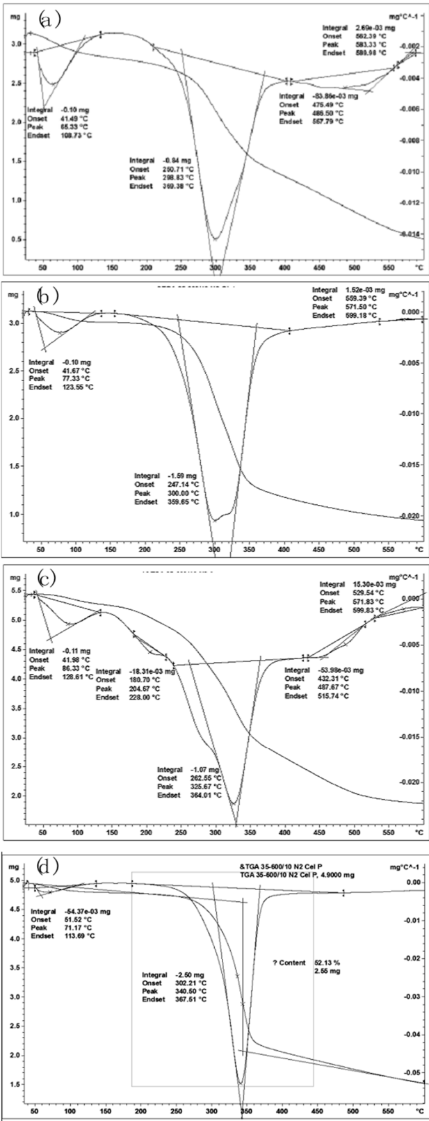
Fig. 2 Thermogravimetric analysis of (a) barley husk, (b) corn cob, (c) agave leaves, and (d) cellulose
