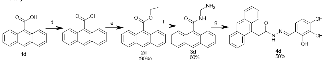
Scheme 1. Preparation of benitrobenzazide derivatives. Reagent and conditions: (A) a : \text{SOCl}_2 (1.2 equiv.), MeOH, 0^\circ\text{C} \rightarrow \text{RT} , 24h; b : \text{N}_2\text{H}_4 \cdot \text{H}_2\text{O} (98%, 4 equiv.), MeOH, RT/reflux 24/72h.; c : (\text{HO})_3\text{C}_6\text{H}_2\text{CHO} ; (1.0 equiv.), MeOH, RT/reflux, 24h. (B) d : \text{SOCl}_2 , (53.6 equiv.), DMF, RT, Ar, 4h; e : EtOH, TEA (1.2 equiv.), RT, 24h; f : \text{N}_2\text{H}_4 \cdot \text{H}_2\text{O} (98%, 100 equiv.), reflux, 72h; g : (\text{HO})_3\text{C}_6\text{H}_2\text{CHO} ; (1.1 equiv.), MeOH, reflux; 24h.
