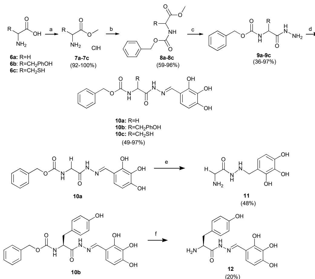
Scheme 4. Preparation of Benserazide analogues. Reagent and conditions: a: MeOH, SOCl 2 (1.2 equiv.), 0°C→RT, 24h; b: CbzCl (1,2 equiv.), TEA (2,5 equiv.), DCM, RT, 24h; c: 98% N 2 H 4 ·H 2 O (4.0 equiv.), MeOH, RT, 24h; d: (HO) 3 C 6 H 2 CHO, (1.2 equiv.), MeOH, RT, 24h/(HO) 3 C 6 H 2 CHO; (1.2 equiv.), THF, reflux, 72h; e: HCOONH 4 , 25% Pd(OH) 2 /C, MeOH, 50°C, Ar, 12h; f: H 2 , 25% mixture Pd(OH) 2 /C and Pd/C, 2.5 bar, MeOH, RT, 6h.
