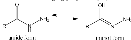
Figure 1. Tautomerism in a hydrazide molecule.
