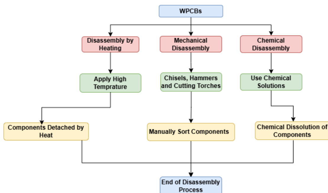
Figure 2. Traditional Disassembly Methods.
