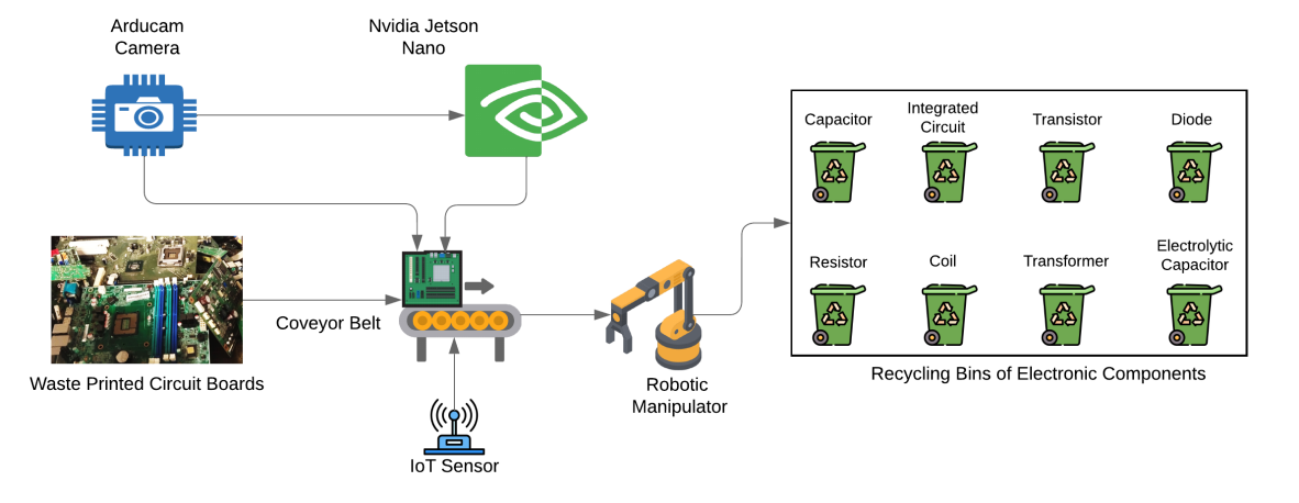
Figure 4. Industrial Realization of automatic disassembly of WPCBs.
