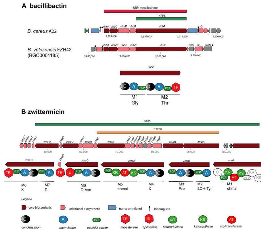
Figure 5. Gene clusters involved in non-ribosomal synthesis of bacillibactin and zwittermixin. A: The siderophore gene cluster in the B. cereus A22 chromosome, Comparison with the corresponding B. velezensis FZB42 gene cluster revealed the presence of the sfp gene downstream of the ballibactin transcription unit as unique feature. B: The gene cluster for synthesis of the PK/NRP hybrid zwittermixin in B. cereus SN4-3.
