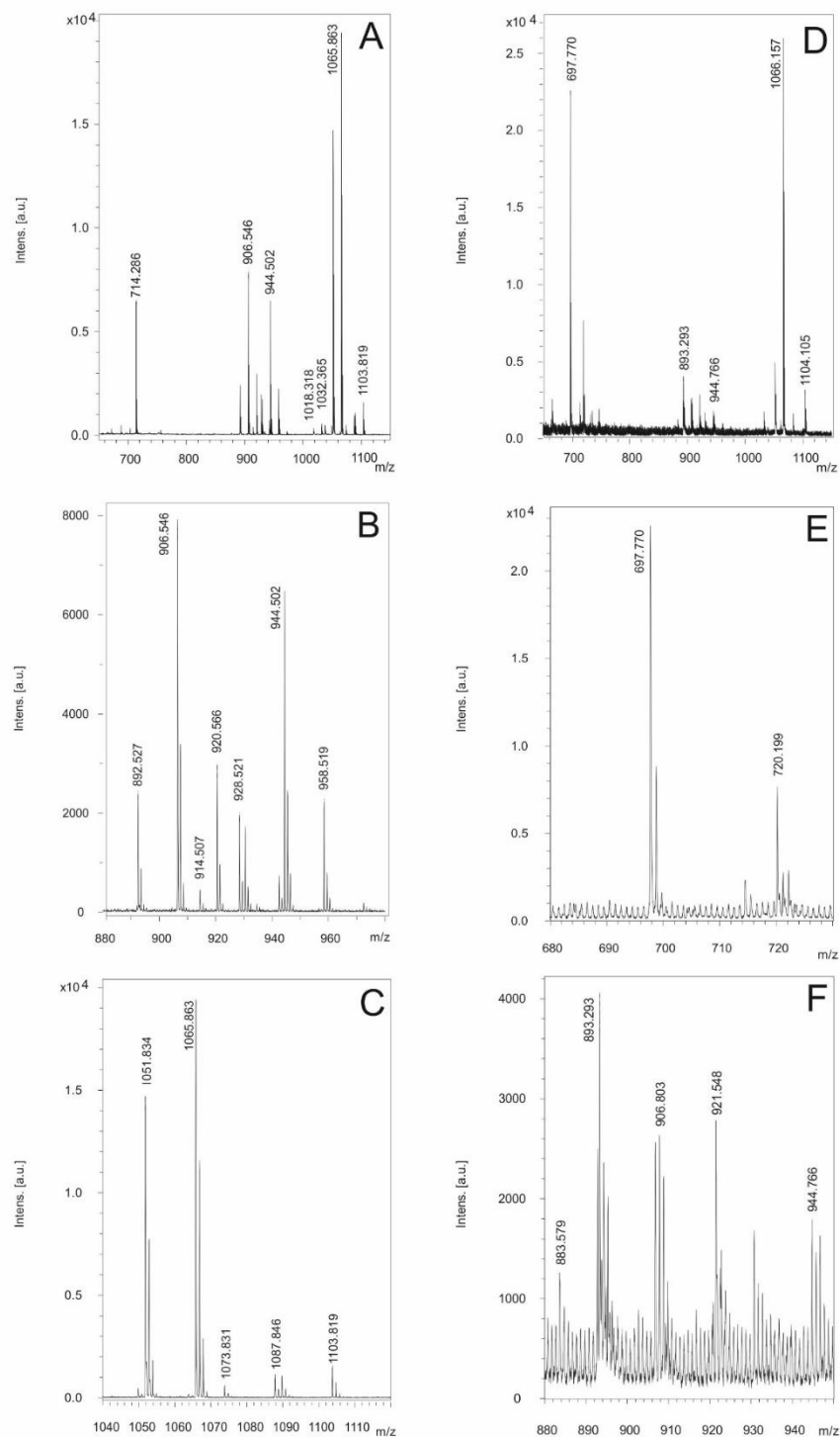
Figure 6. Bioactive compounds produced by B. cereus A22. A-C: Compounds detected in surface extracts of this strain. A: MALDI-TOF mass spectrum of a surface extract of strain A22 grown on agar plates in the Landy medium in the mass range from m/z = 650-1150. B: Kurstakins observed between m/z = 880-980. C: Detection of a yet unknown prominent product with mass numbers of 1051.83 and 1065.86 Da. D-F: Compounds found in the culture filtrate of strain A22 grown in the Landy medium for 48 h. D: MALDI-TOF mass spectrum of a culture filtrate of strain A22 grown in the Landy medium for 48 h in the mass range from m/z = 690 - 1120. E: Detection of the arylpolyene-lipopeptide thumolycin and the siderophore
