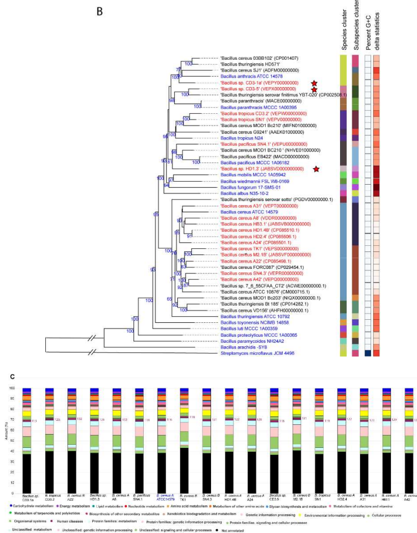
Figure 1. A: Approximately-maximum likelihood phylogenetic tree for 128 Bacillus cereus group genomes, calculated by EDGAR using the Fast tree software ( http://www.microbesonline.org/fasttree/ ). The unrooted tree was built out of a core of 1054 genes per genome. The core has 280,349 AA residues/bp per genome, 35,884,672 in total. Bacillus_A is a term used from GTDB ( https://gtdb.ecogenomic.org ) for genomospecies belonging to the B. cereus group. The tree is divided into three main branches (1-3). Cluster 3 is further divided into the subclusters 3A and 3B. The 21 type strains are labelled in blue letters. The isolates, investigated in this study, are indicated by red letters and belong all to the subcluster 3B. Related subclusters containing the plant-associated Vietnamese isolates are marked by irregular colored fields. The ANI values are documented in Suppl. Fig. S3. B: Bacillus cereus tree inferred with FastMe 2.1.6.1 [34] from GBDP distances calculated from whole-proteome data using the Type (Strain) Genome Server TYGS ( https://tygs.dsmz.de ). Analysis was performed using both, Maximum Likelihood and Maximum Parsimony, with 16 type strains (blue letters) and 17 genome sequences obtained from the Bacillus cereus strains isolated from Vietnamese crop plants (red letters). In addition, 16 strains with similar proteomes obtained from the NCBI data bank, were included yielding a total of 49 proteomes. The branch lengths are scaled in terms of GBDP distance formula ds . Putative novel genomospecies were indicated by red stars. The numbers above branches are GBDP pseudo-bootstrap support values > 60% from replications, with an average branch support of 87.5 %. The first two colored columns to the right of each name refer to the genome-based species and subspecies clusters, specified by dDDH cut-off values of 70% and 79%, respectively. C: Functional KEGG category analysis of plant-associated B. cereus group isolates. Type strain B. cereus ATCC 14579 was included in the analysis. The number of genes associated with human diseases is indicated. 125216 KEGG functional categories (including not annotated sequences) were found in the selected 18 contigs.
