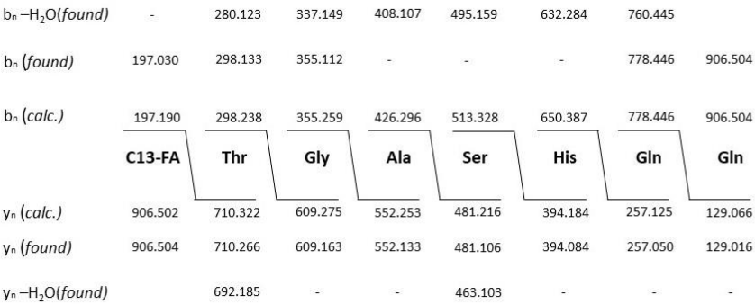
Figure 7. Mass spectrometric sequence determination of a C13-kurstakin produced by B. cereus A22 with a parent ion [M + H] + = 906.504 derived from product ion patterns obtained by LIFT-MALDI-TOF/TOF fragment ion spectra. FA: fatty acid component.
