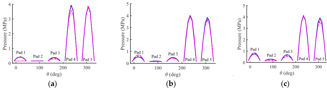
Figure 4. Hydrodynamic pressure distribution on intact and worn TPJBs. a) Shaft rotational speed is equal to 3500rpm b) Shaft rotational speed is equal to the first critical speed of the system c) Shaft rotational speed is equal to 10200rpm. (Blue solid line: Intact bearing, Red dashed line: Bearing with maximum wear depth of 10 \mu m, Magenta dashed dot line: Bearing with maximum wear depth of 20 \mu m.).
