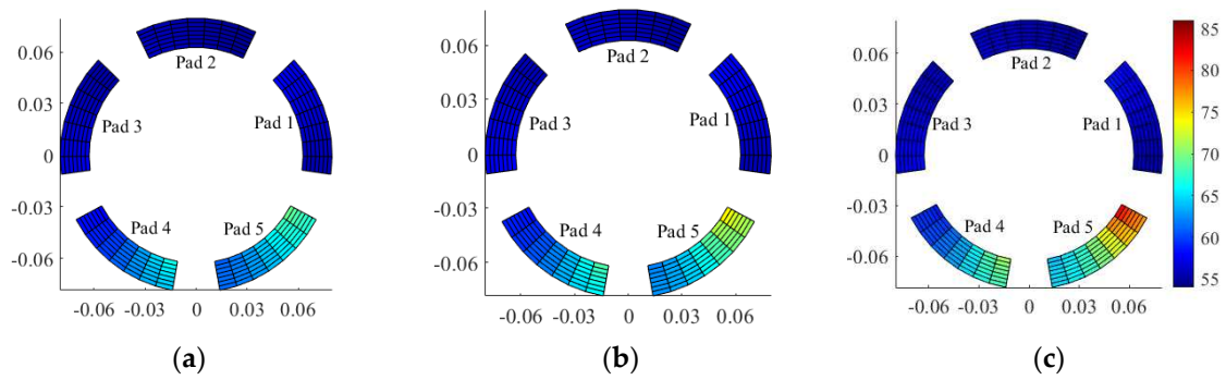
Figure 6. Pad temperature distribution at the first critical speed of the system. a) Intact bearing b) Maximum wear depth: 10μm c) Maximum wear depth: 20μm.
