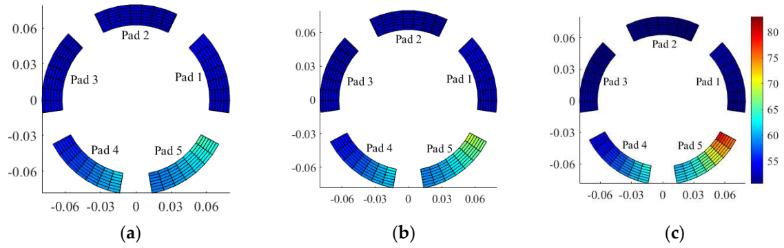
Figure 5. Pad temperature distribution at 3500rpm. a) Intact bearing b) Maximum wear depth: 10μm c) Maximum wear depth: 20μm.
