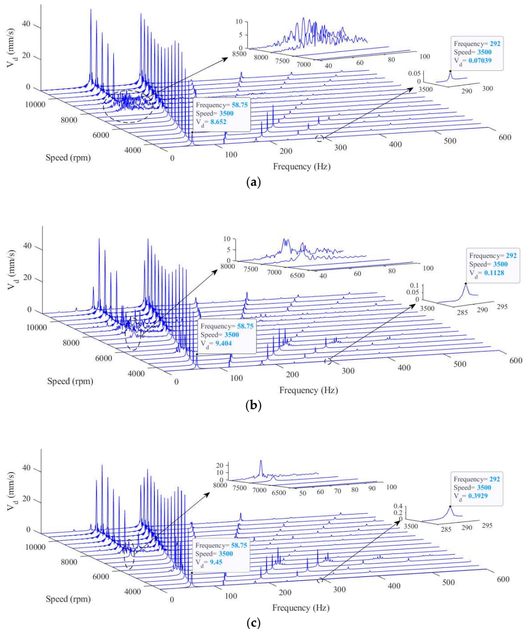
Figure 15. Waterfall diagrams for disc velocity in a range of rotor speeds and different wear severities, a) Intact bearing b) Maximum wear depth: 10μm c) Maximum wear depth: 20μm.
