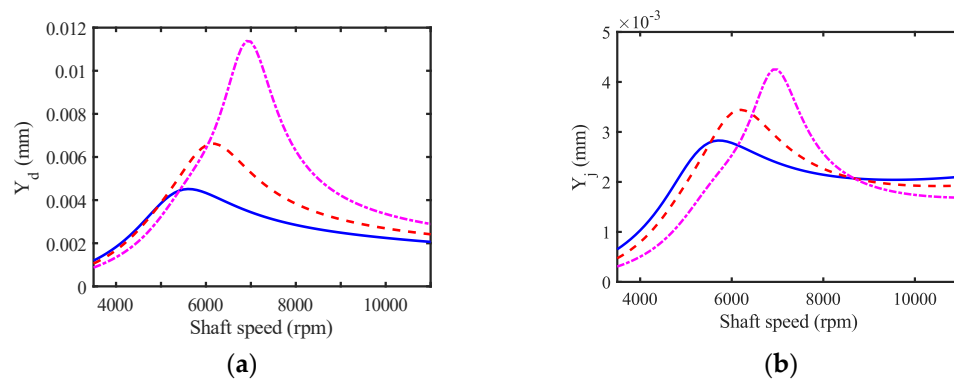
Figure 12. Rotor vibration amplitudes for intact and worn TPJBs considering 2 \times 10^{-6}\text{kg.m} mass unbalance on disc a) Disc vibration amplitude b) Journal vibration amplitude (Blue solid line: Intact bearing, Red dashed line: Bearing with maximum wear depth of 10\mu\text{m} , Magenta dashed dot line: Bearing with maximum wear depth of 20\mu\text{m} .).
