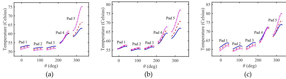
Figure 8. Pads inner surface temperature for intact and worn TPJBs a) Shaft rotational speed equals 3500rpm b) Shaft rotational speed equals to the first critical speed of the system c) Shaft rotational speed equals 10200rpm. (Blue solid line: Intact bearing, Red dashed line: Bearing with maximum wear depth of 10 \mu m, Magenta dashed dot line: Bearing with maximum wear depth of 20 \mu m.).
