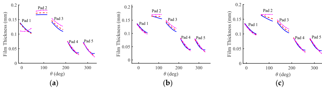
Figure 3. Oil film thickness on intact and worn TPJBs. a) Shaft rotational speed is equal to 3500rpm b) Shaft rotational speed is equal to the first critical speed of the system c) Shaft rotational speed is equal to 10200rpm. (Blue solid line: Intact bearing, Red dashed line: Bearing with maximum wear depth of 10 \mu m, Magenta dashed dot line: Bearing with maximum wear depth of 20 \mu m.).
