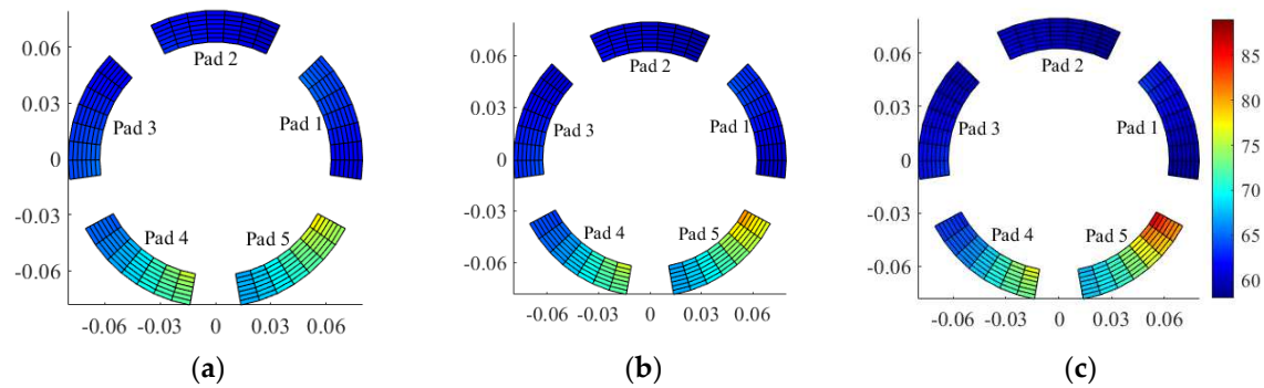
Figure 7. Pad temperature distribution at 10200rpm. a) Intact bearing b) Maximum wear depth: 10μm c) Maximum wear depth: 20μm.
