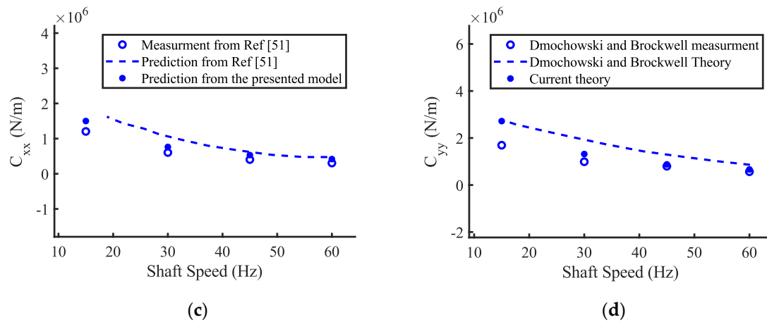
Figure A1. Comparisons of the obtained tilting pad bearing dynamic coefficients with presented experimental results in [51].
