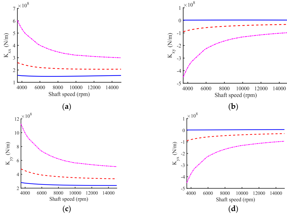
Figure 10. TPJB stiffness for intact and worn bearings cases at different speeds (Blue solid line: Intact bearing, Red dashed line: Bearing with maximum wear depth of 10\mu\text{m} , Magenta dashed dot line: Bearing with maximum wear depth of 20\mu\text{m} ).
