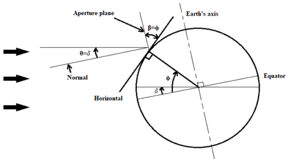
Figure 5. Solar geometry.
