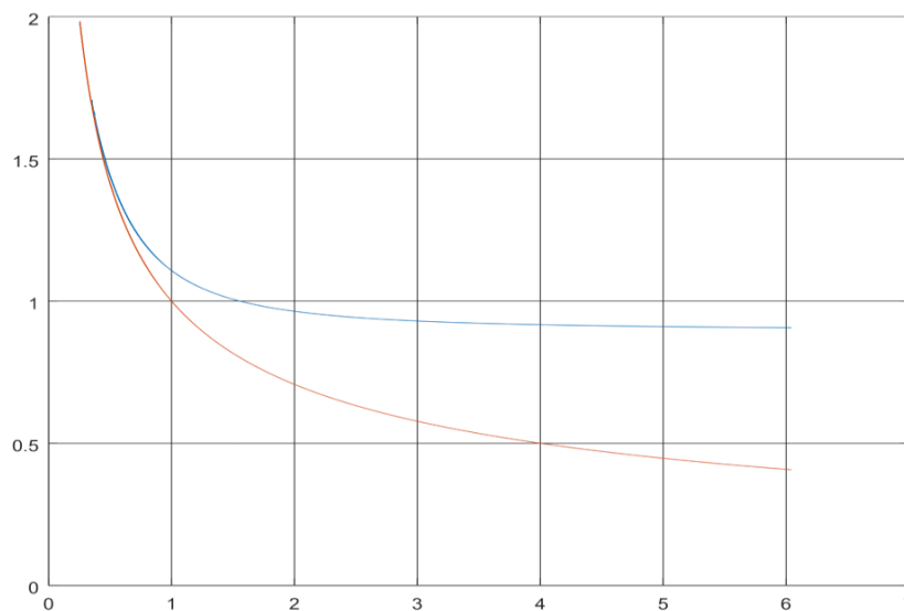
Figure 2. The rotation curve v(r) \equiv \omega(r)r|_{\lambda=1} obtained from (61) by setting \lambda = 1 (blue). The Newtonian curve for the same parameters (red).
