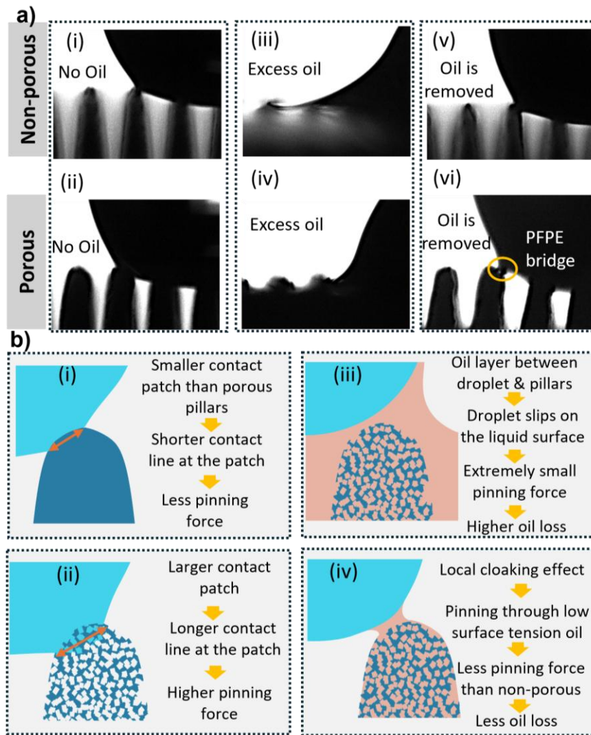
Figure 7. Depinning dynamics of water droplets on non-porous and porous PDMS micropillars under different PFPE oil-infusion conditions. (a) Side-view images showing droplet depinning on non-porous (top row) and porous (bottom row) pillars with no oil (i, ii), with excess PFPE oil (iii, iv), and after removal of excess oil (v, vi). Surfaces containing excess PFPE oil exhibit smooth and continuous recession of the contact line, whereas non-infused and oil-removed surfaces show intermittent depinning. A PFPE bridge is visible in panel (vi), indicating partial oil transfer during droplet motion. (b) Schematic interpretation of the corresponding depinning behaviour, illustrating differences in contact-patch size, pinning strength, formation of cloaking layers, and the effects of oil retention or loss on droplet mobility.
