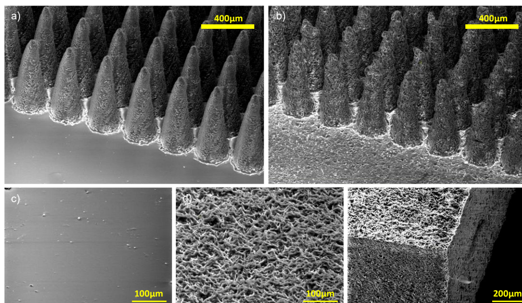
Figure 2. Scanning electron microscope images of non-porous and porous PDMS structures. a) Non-porous micropillars with laser-machined PMMA mould. b) Porous micropillars with the same mould as (a). c) Plain PDMS surface moulded from unmachined parts of the PMMA mould. d) and e). Porous PDMS plain surface and sliced porous PDMS substrate. Interconnected pores are clearly visible on the sliced sample.
