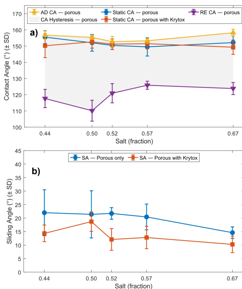
Figure 6. Wettability measurements of porous and oil-infused porous substrates. a) Contact angle-related parameters of porous micro-pillared sample and porous with PFPE oil-infused samples. b) Sliding angle (SA) of a 10 \mu\text{L} droplet on porous micropillars and the same substrates with oil infused.
