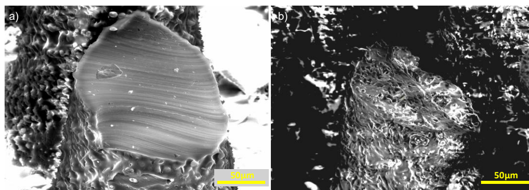
Figure 3. Magnified images of sliced micropillars. a) Nonporous micropillar b) Porous micropillar with 2:1 salt to PDMS w/w ratio. Interconnected porosity throughout the pillar surface and the pillar core is visible.
