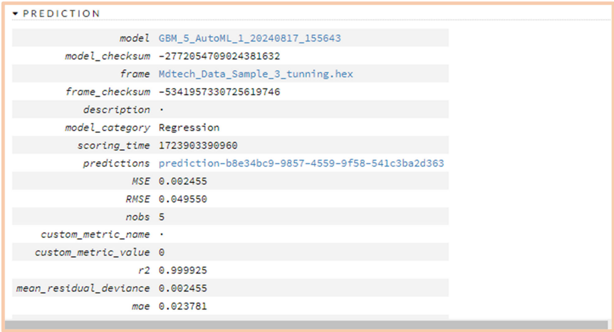
Figure 9. GBM output for MedTech Cluster.
