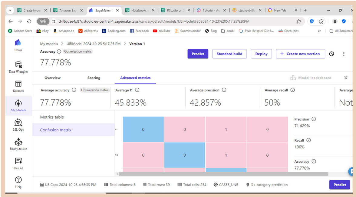
Figure 17. Prediction and Accuracy calculation from AWS SageMaker for UBI Capabilities.
