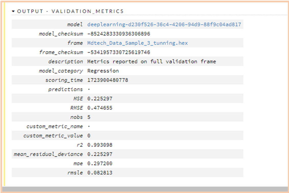
Figure 12. Deep Learning Output training for MedTech Cluster.
