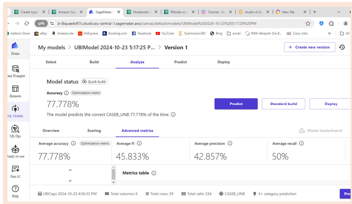
Figure 15. Data training of AWS SageMaker.
