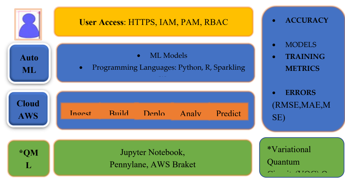
Figure 6. Architechture for Data Training.
