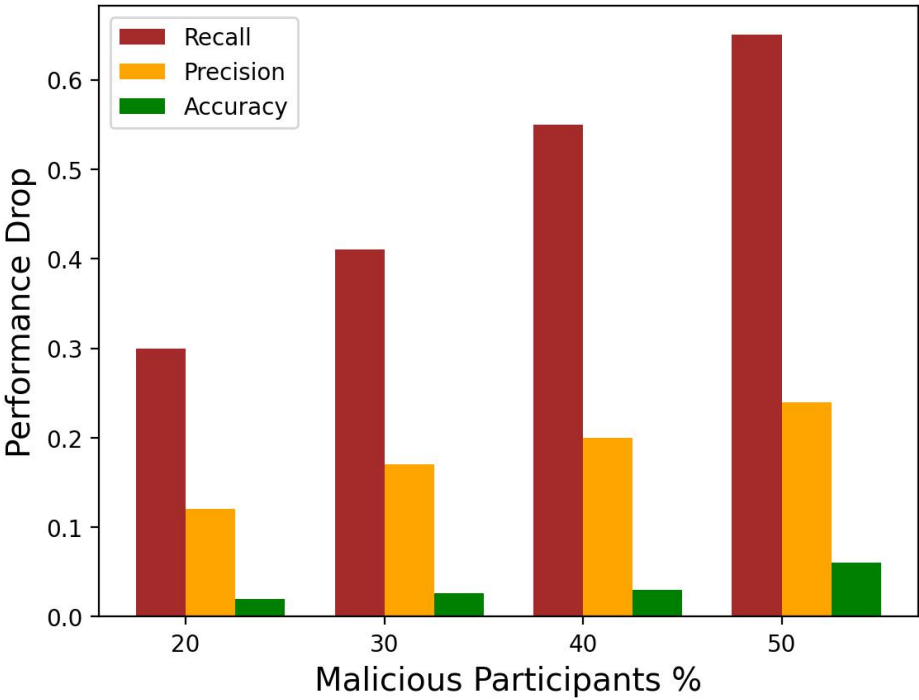
Figure 4. Impact of attacks on the performance for CIFAR-10 data.
