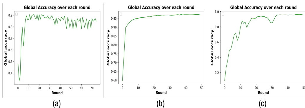
Figure 7. Effect on Convergence. (a) in presence of malicious workers, (b) all honest workers in IID setup, and (c) all honest workers in non-IID setup.
