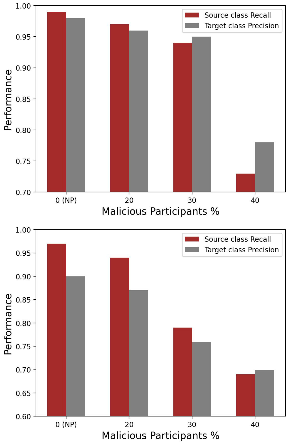
Figure 3. Impact of label-flipping attacks on targeted classes on (a) MNIST data and (b) Fashion-MNIST data.
