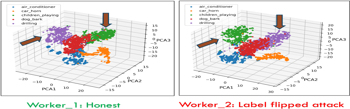
Figure 8. Class-wise cluster representation for workers. Honest worker (left) and attacked worker (right).
