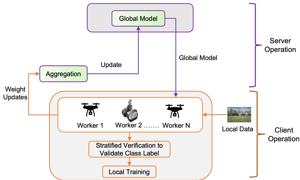
Figure 1. Proposed Confident Federated Learning.
