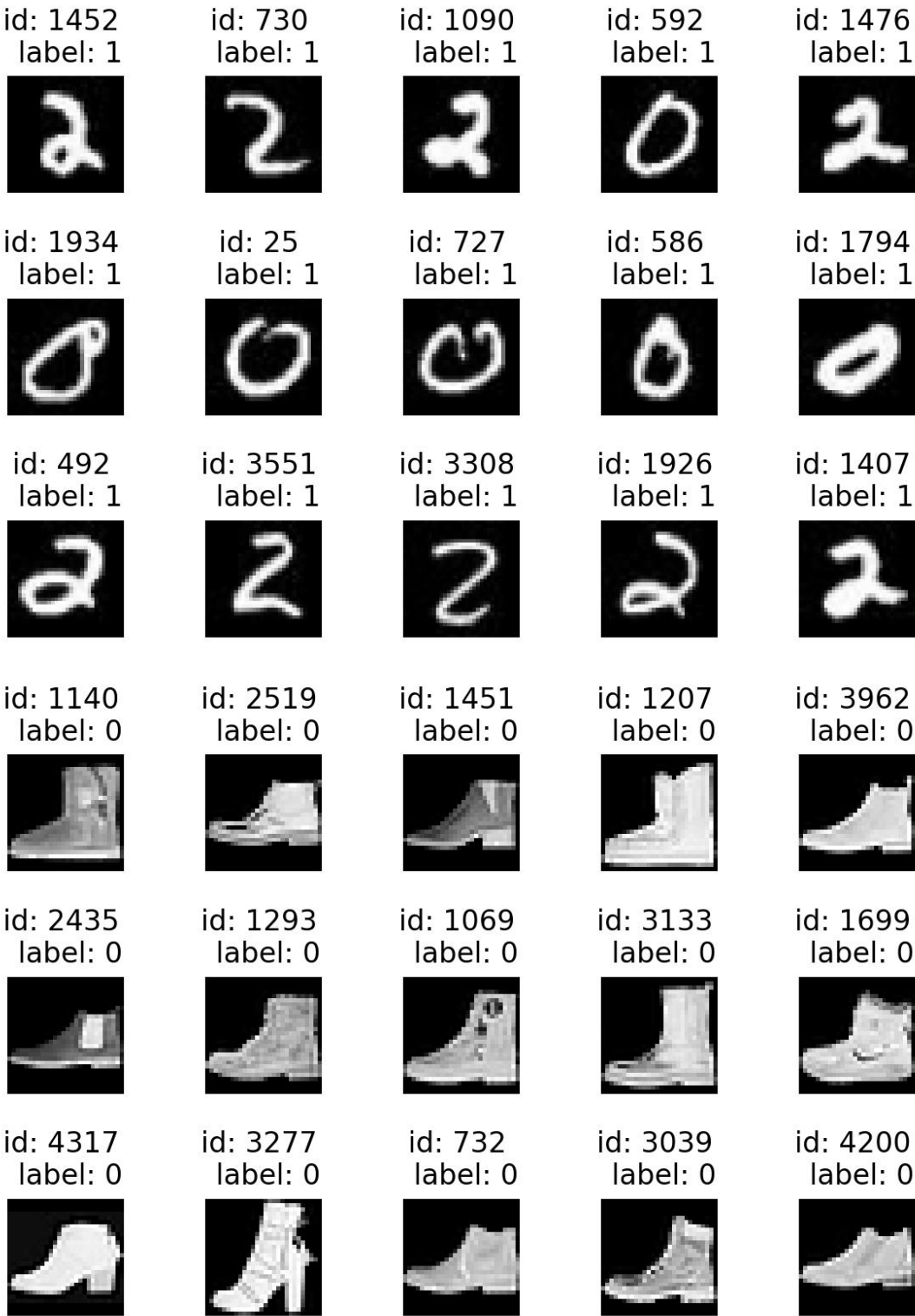
Figure 5. Detection of label flipped samples.
