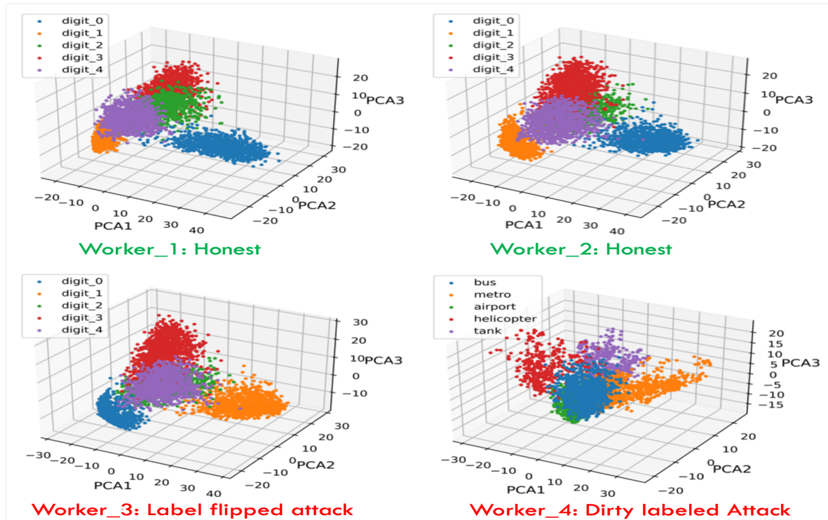
Figure 6. Clustering based approach: (a) honest worker, (b) honest worker, (c) worker attacked with label flipping among digit-0 and digit-1 class, (d) worker attacked with dirty labeling.
