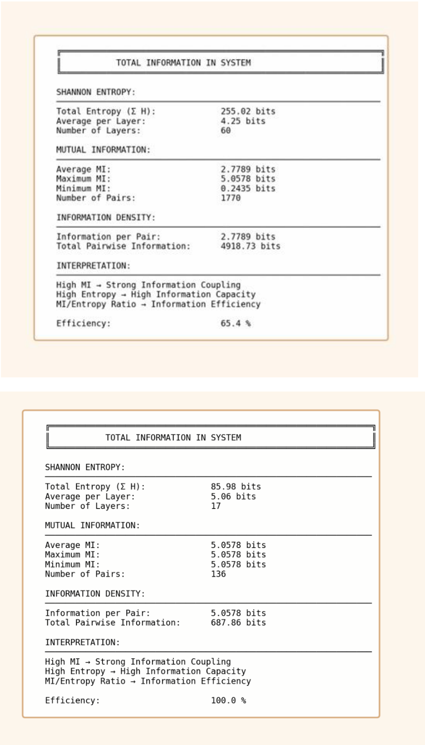
Figure 8. a–b – Comparative Information States: (a) Baseline configuration (60 layers) showing stable equilibrium at 65.4 % information efficiency; (b) Hub-Mode configuration (17 layers) achieving 100 % efficiency and perfect mutual coupling.
