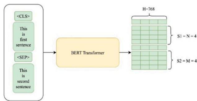
Figure 2. BERT method architecture.
