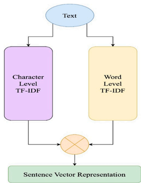
Figure 3. The architecture of the TF+IDF method.
