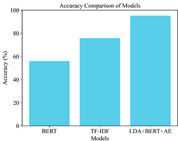
Figure 9. Result of accuracy of models.
