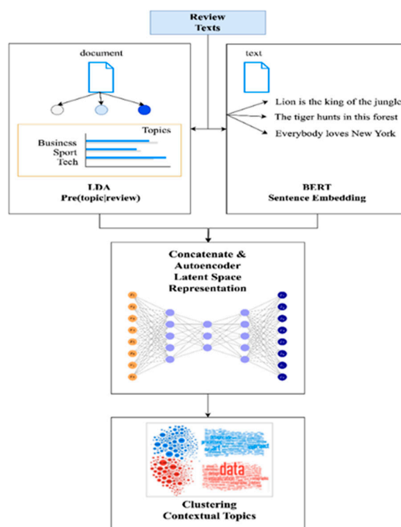
Figure 4. The architecture of the hybrid method LDA+BERT+AE.
