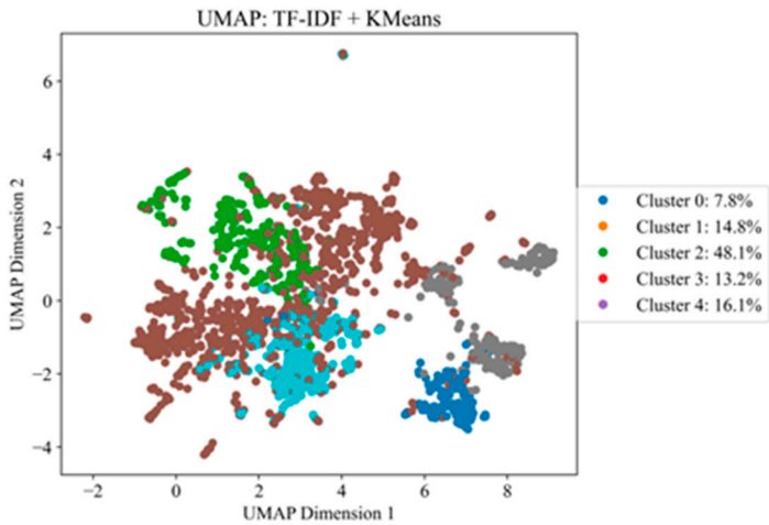
Figure 5. Result of clustering using the TF+IDF method.
