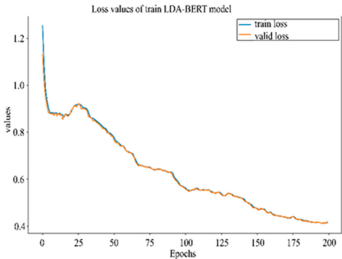
Figure 8. Change in the loss value during the training of the hybrid LDA+BERT+AE model.
