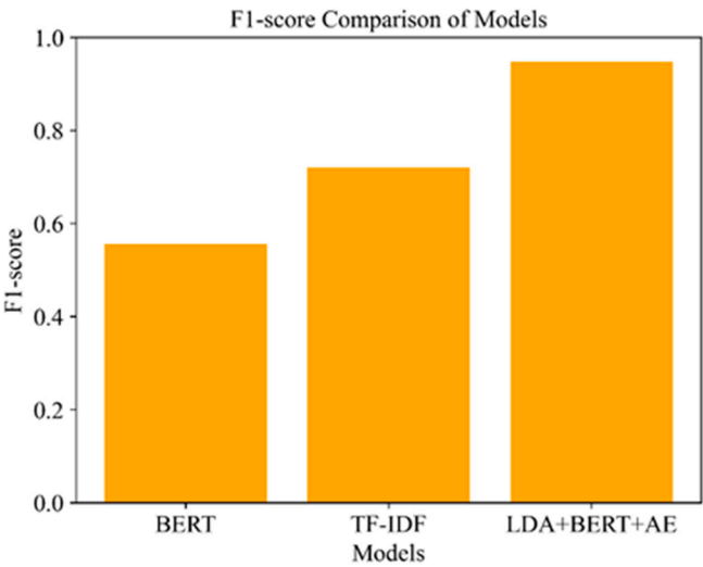
Figure 10. F1-score results of models.
