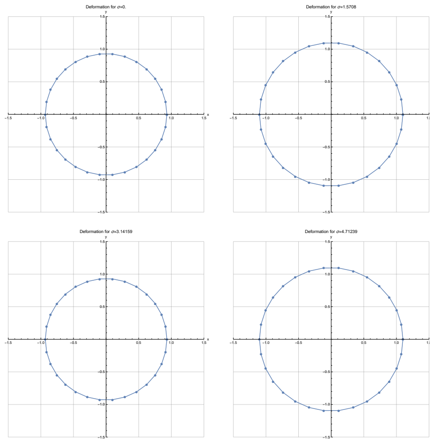
Figure 4. Deformation visualization for particles on a circle.
