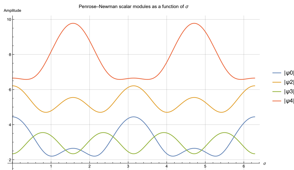
Figure 3. Oscillations of Penrose–Newman scalars.
