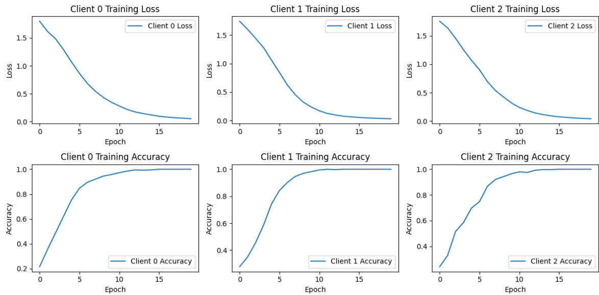
Figure 2. Training loss vs. Accuracy for BERT.
