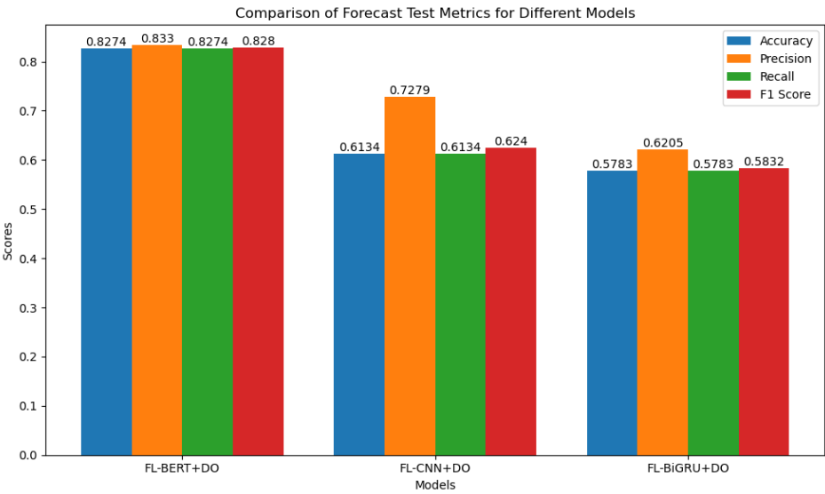
Figure 6. Comparative Analysis of Forecasting for Different Models.
