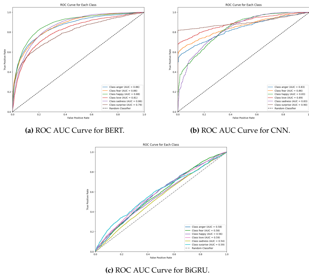
Figure 7. ROC AUC Curve for BERT, CNN, and BiGRU.
