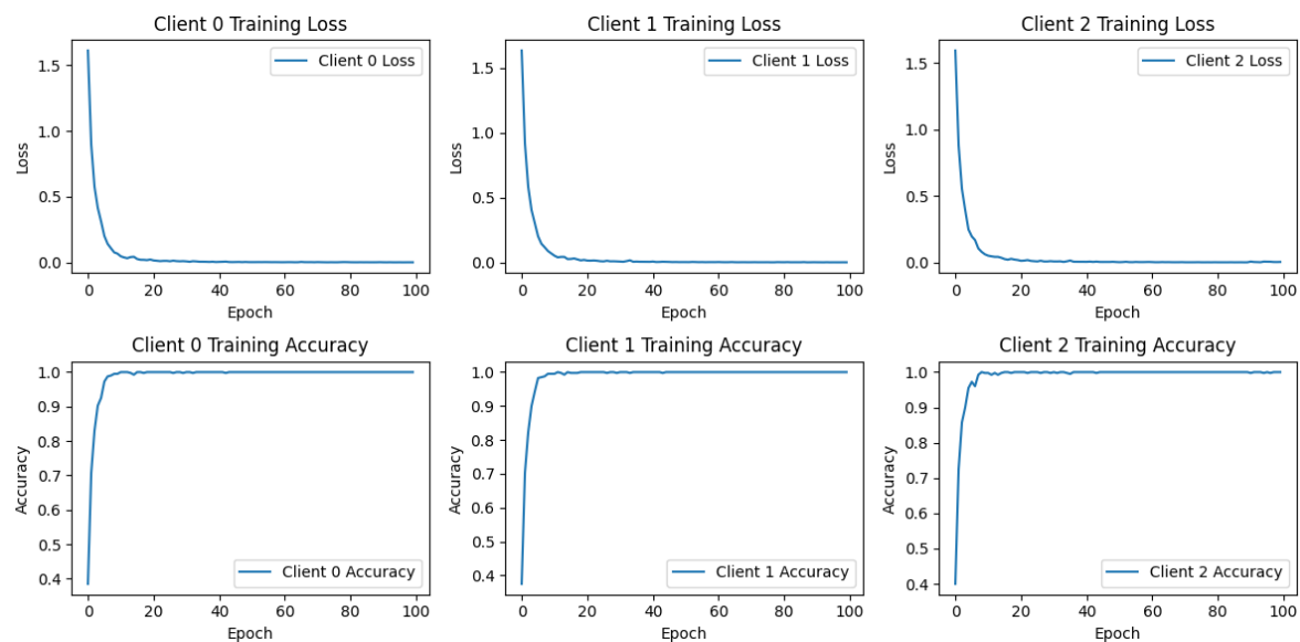
Figure 3. Training loss vs. Accuracy for CNN.
