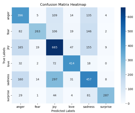
(c) Confusion Matrix for BiGRU.
