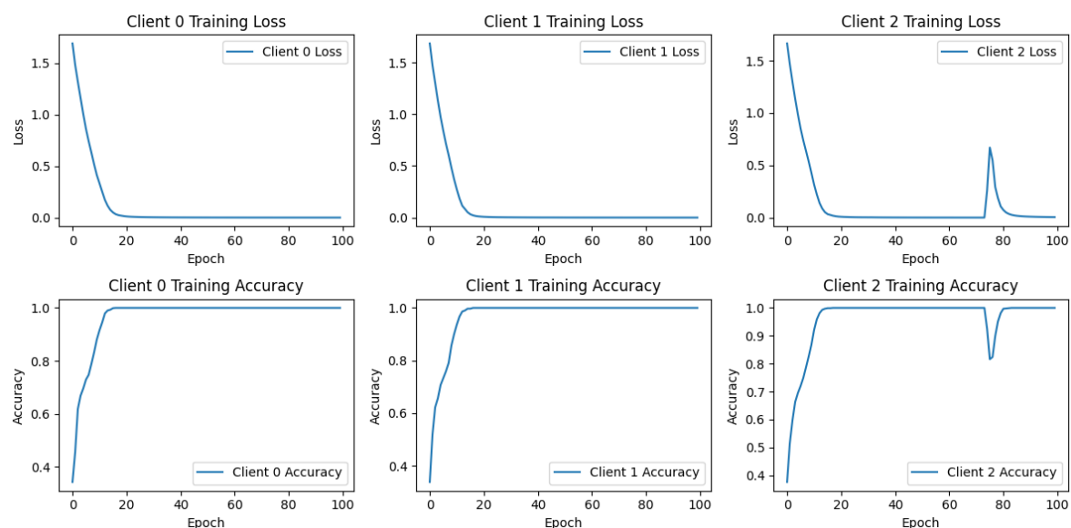
Figure 4. Training loss vs. Accuracy for BiGRU.
