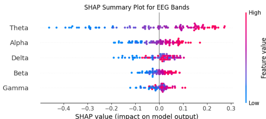
Figure 11. SHAP plot of the BiLSTM model.
