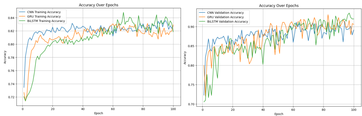
Figure 9. Training and Validation accuracies evaluation.
