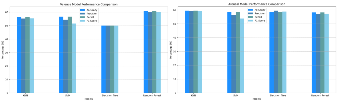
Figure 6. Classical ML Models Performance Comparison.
