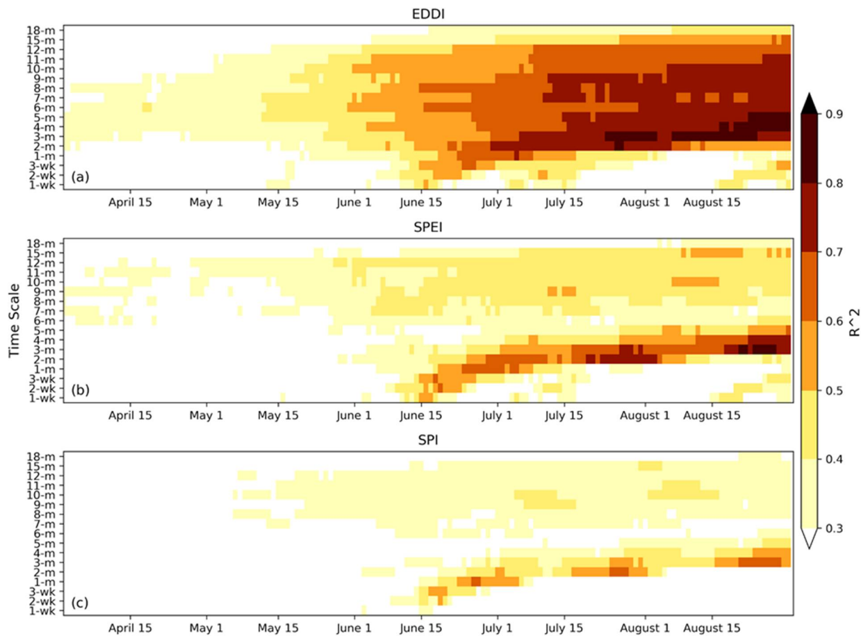
Figure 2: Average summer ERC correlated to (a) EDDI, (b) SPEI, and (c) SPI at the Northern Sierra Nevada, California PSA. Vertical axis indicates drought index time scale in weeks (wk) or months (m) and horizontal axis shows the drought index ending day for the correlation. The zero-day lag is indicated at 31 August and the start of season lag (~90-day) is indicated at 1 June.
