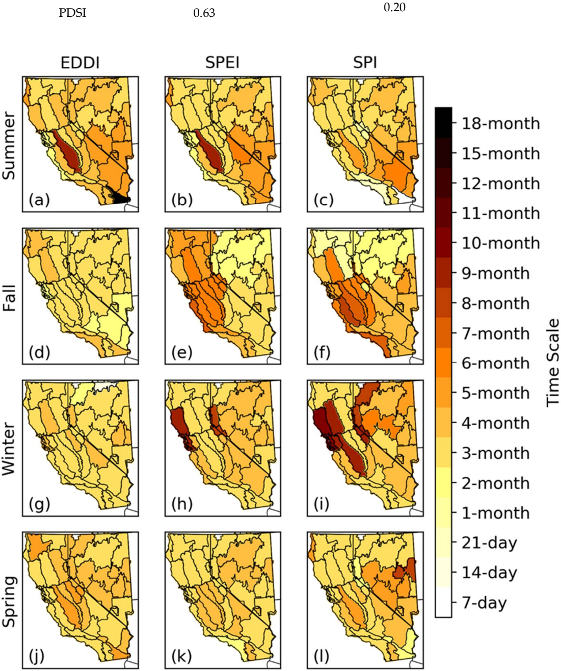
Figure 4: Time scale of each drought index associated with the maximum correlations shown in Figure 2.
