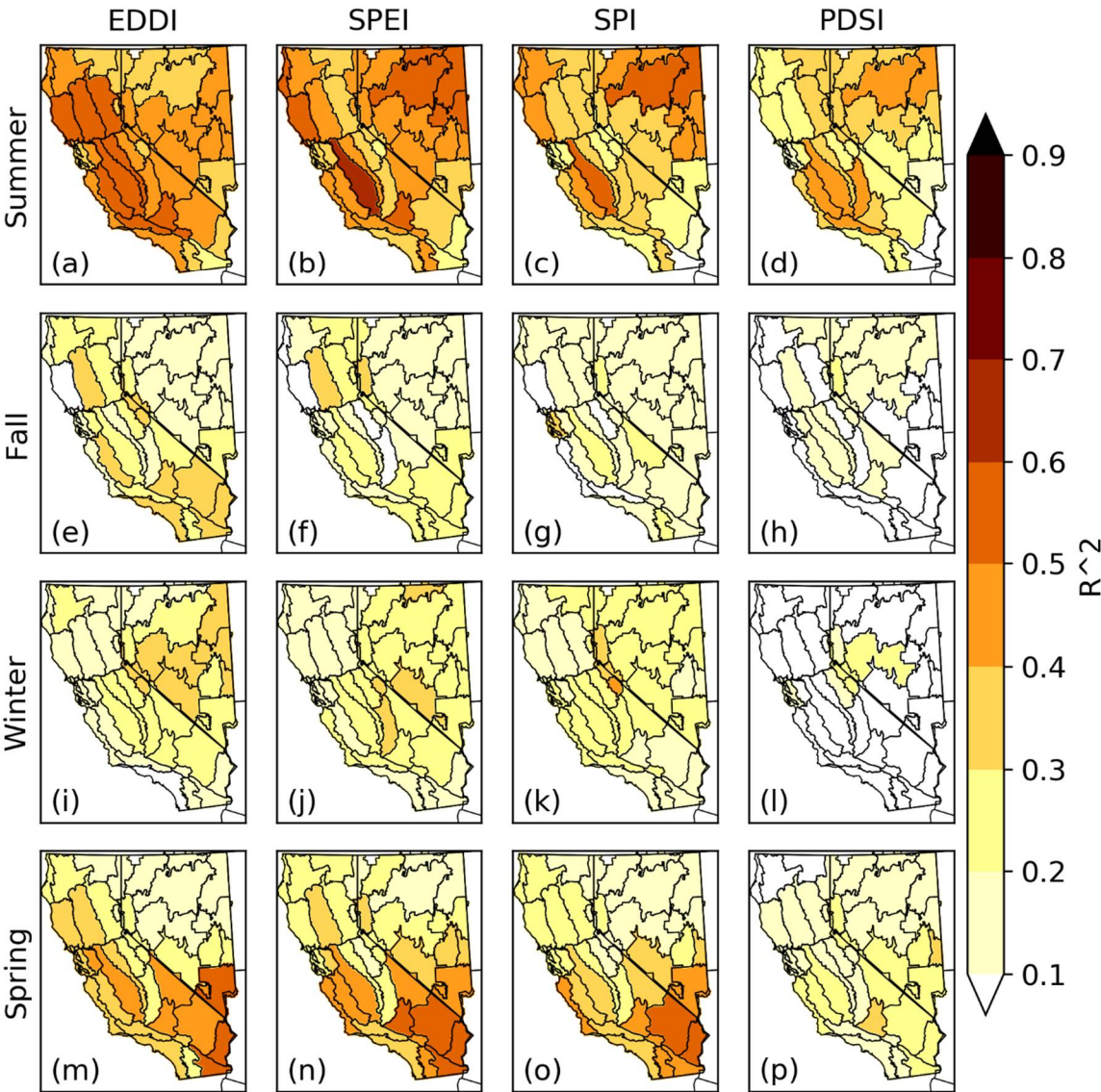
247 248 Figure 6: Start of season (90-day lag) R^2 of each drought index with the seasonal Energy Release 249 Component (ERC) fire danger index by season across the period 1979-2015 for each PSA in California 250 and Nevada.
