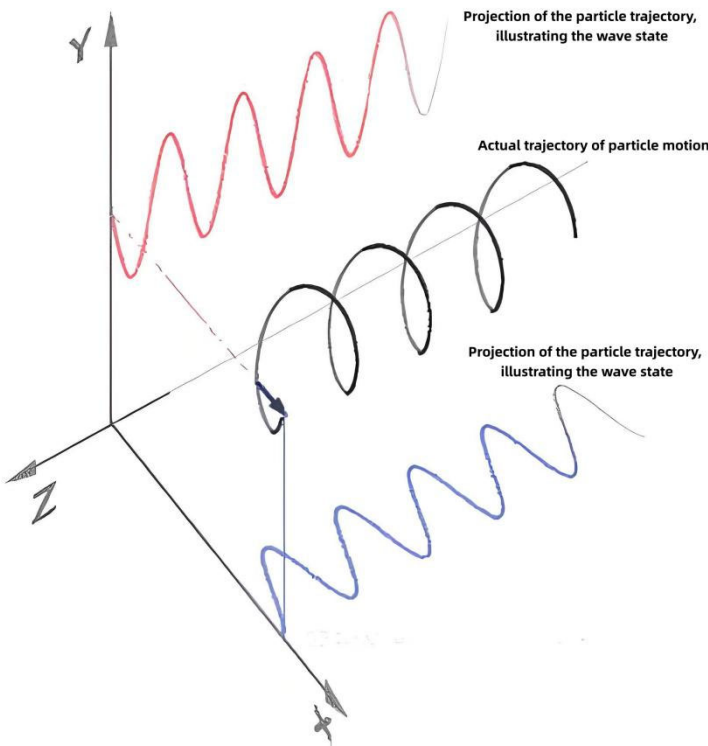
Figure 2. Schematic Diagram of the Geometric Trajectory and Projection of Photon Uniform Helical Linear Motion.
