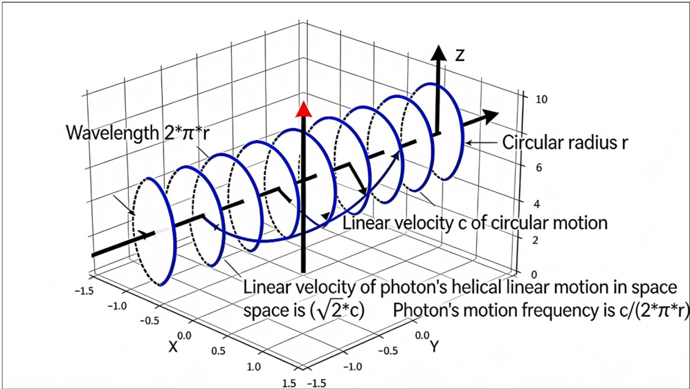
Figure 1. Schematic Diagram of the Geometric Trajectory and Key Parameters of Photon Uniform Helical Linear Motion.
