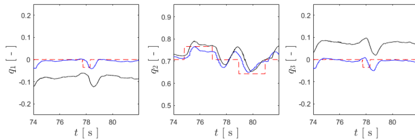
(a) From left to right: tracking results for q_1 , q_2 and q_3 for the IBKS controller, with the references shown in dashed red, the ground truth in black, and the estimated quaternion in blue.
