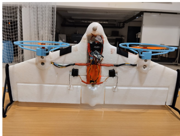
Figure 6. Experimental prototype based on the X-Vert VTOL.
