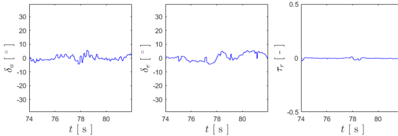
(b) From left to right: plots of \delta_a , \delta_e and \tau_r for the IBKS controller, in blue.
