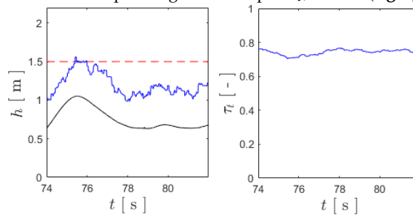
(b) Tracking results for h = -D for the experimental flight with the IBKS controller, with the reference in dashed red, the estimated value in blue, and the ground truth in black ( left ), and the corresponding throttle input \tau_t , in blue ( right ).
