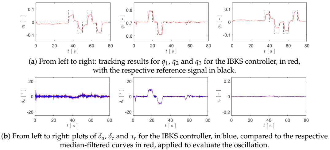
Figure 3. Plots for the HITL simulations using the IBKS controller.
