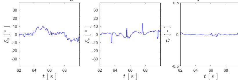
(b) From left to right: plots of \delta_a , \delta_e and \tau_r for the INDI controller, in blue.
