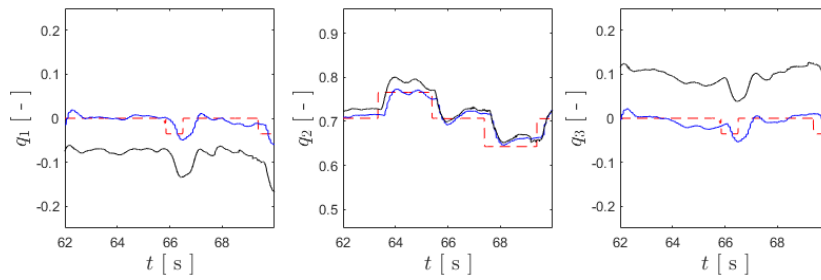
(a) From left to right: tracking results for q_1 , q_2 and q_3 for the INDI controller, with the references shown in dashed red, the ground truth in black, and the estimated quaternion in blue.
