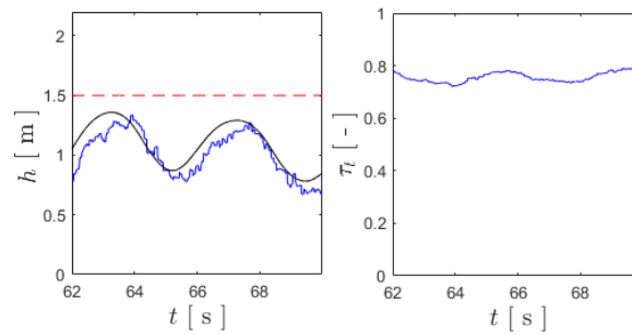
(a) Tracking results for h = -D for the experimental flight with the INDI controller, with the reference in dashed red, the estimated value in blue, and the ground truth in black ( left ), and the corresponding throttle input \tau_t , in blue ( right ).
