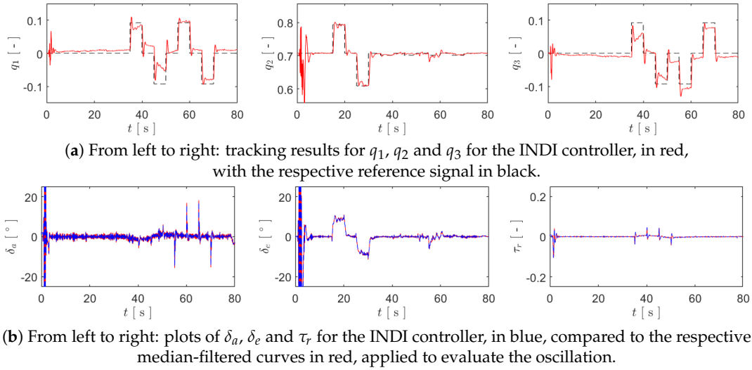
Figure 2. Plots for the HITL simulations using the INDI controller.
