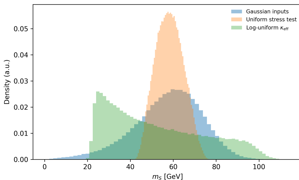
Figure 15. Prior-sensitivity illustration for the induced distribution of m_s in Eq. (56). The first curve uses the Gaussian benchmark inputs quoted in the main text; the second applies a uniform stress test around the central values; the third adopts a deliberately broader log-uniform prior for \kappa_{\text{eff}} . The purpose is not to advocate any particular prior but to make the protocol dependence of the inferred scale explicit.
