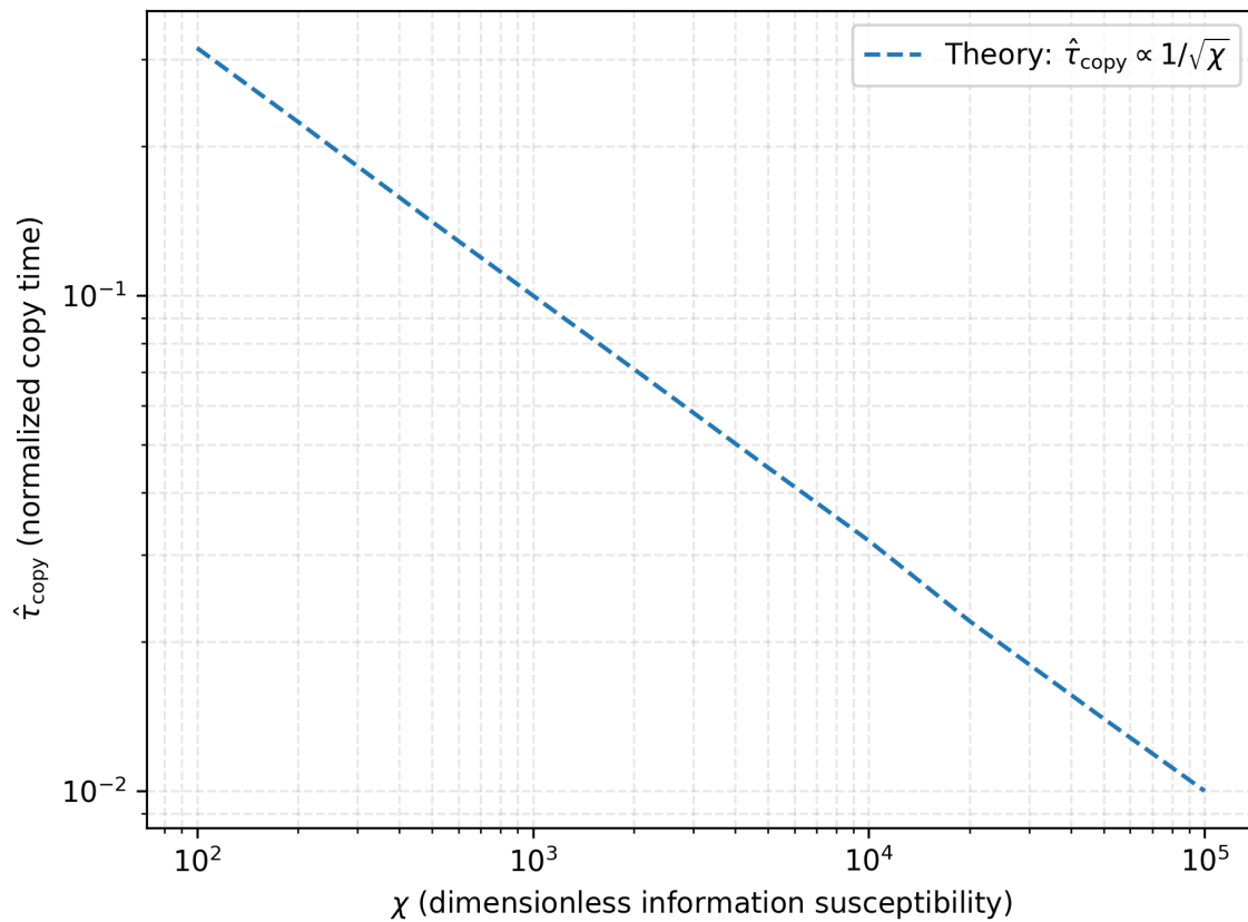
Figure 8. Benchmark relation between the copy time and the information susceptibility in stabiliser-code diffusion models (from the Supplemental Material). This is consistent with the interpretation that the local copy time encodes the effective “slowness” of information propagation.
