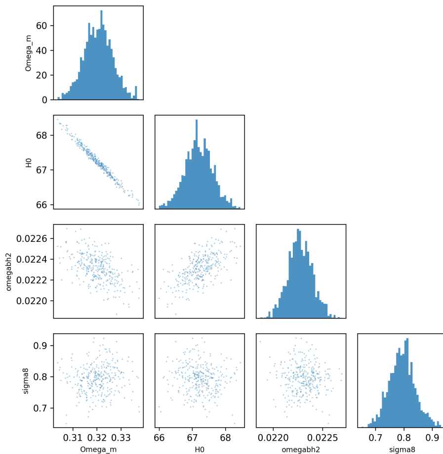
Figure 14. Identifiability diagnostic for the auxiliary MCMC consistency check used in the cosmology module of the reproducibility package. The plot illustrates correlations among the sampled parameters and highlights directions that would remain weakly constrained without informative priors. This figure is provided to make the role of priors explicit rather than to claim a definitive global fit.
