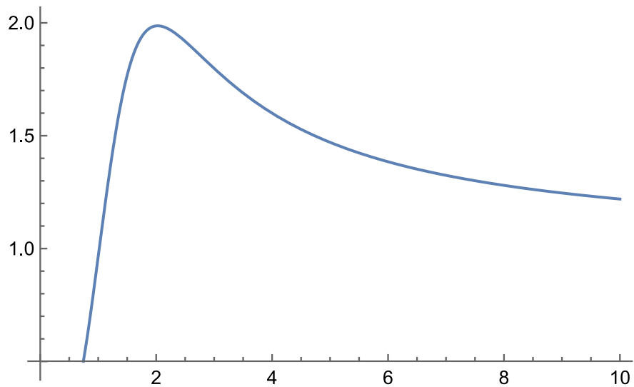
Figure 4.13. Interaction II. The function y = \frac{v^2(x)}{\sigma} for a point mass, if k = 0.1 . Source: Figure by author.
