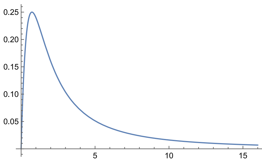
Figure 4.6. Interaction I. The function y = \frac{2GM}{\sigma^2} g(x) for a point mass, if k = 0 . Source: Figure by author.
