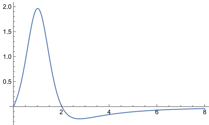
Figure 4.15. Interaction II. The function y = \frac{2GM}{\sigma^2} g(x) for a point mass, if k = 0.1 . Source: Figure by author.
