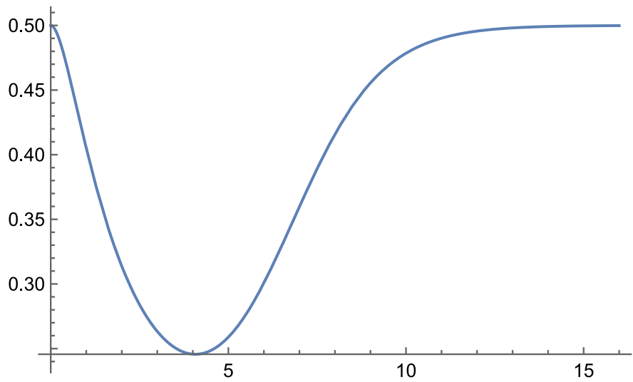
Figure 4.17. Interaction III. The function y = \frac{V(x)}{\sigma} for a point mass, if k = 0.1 . Source: Figure by author.
