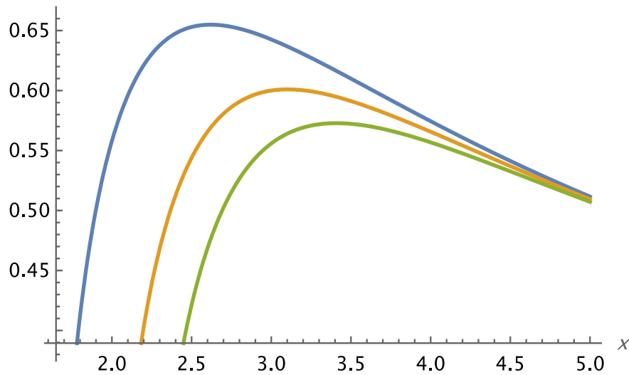
Figure 4.21. Interaction IV. The graph of the function y = \frac{2GM}{\sigma^2} g(x) for a point mass, if k = -1 .
