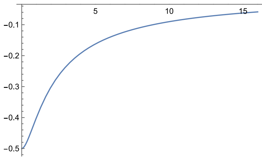
Figure 4.5. Interaction I. The function y = \frac{V(x)}{\sigma} for a point mass, if k = 0 . Source: Figure by author.
