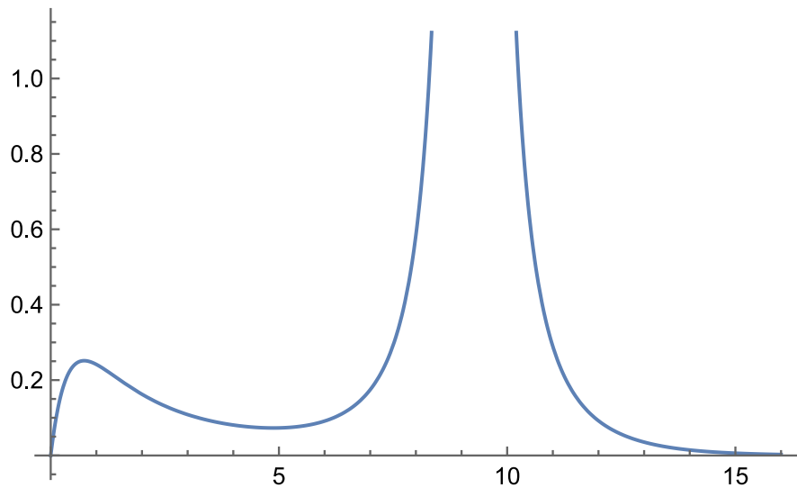
Figure 4.3. Interaction I. The function y = \frac{2GM}{\sigma^2} g(x) for a point mass, if k = -0.01 . Source: Figure by author.
