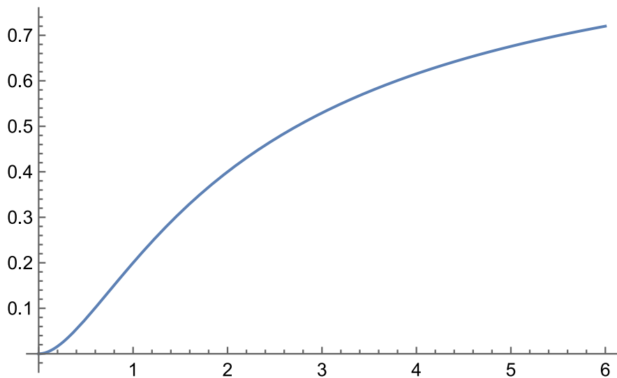
Figure 4.4. Interaction I. The function y = \frac{v^2(x)}{\sigma} for a point mass, if k = 0 . Source: Figure by author.
