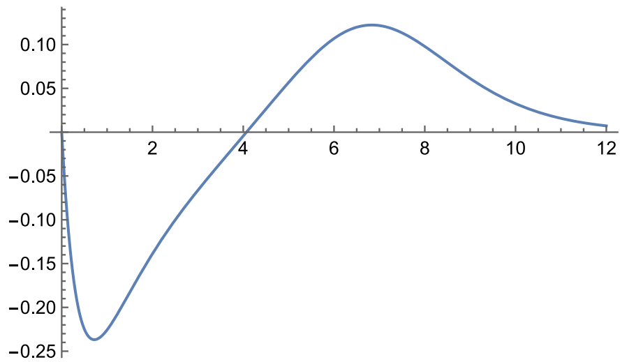
Figure 4.18. Interaction III. The function y = \frac{2GM}{\sigma^2} g(x) for a point mass, if k = 0.1 . Source: Figure by author.
