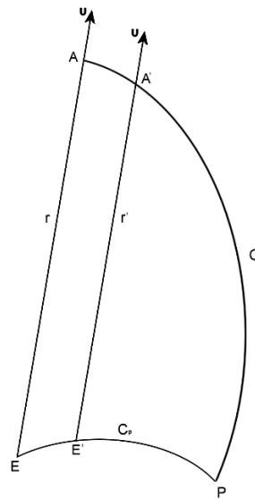
Figure 3.2. Curves C_p and C in the surrounding spacetime of a randomly moving point electric charge q . Source: Figure by author.
