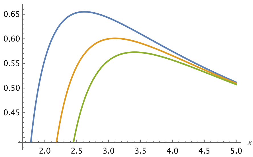
Figure 4.19. Interaction IV. The graph of the function y = \frac{v^2(x)}{\sigma} for a point mass, if k = -1 . Source: Figure by author.
