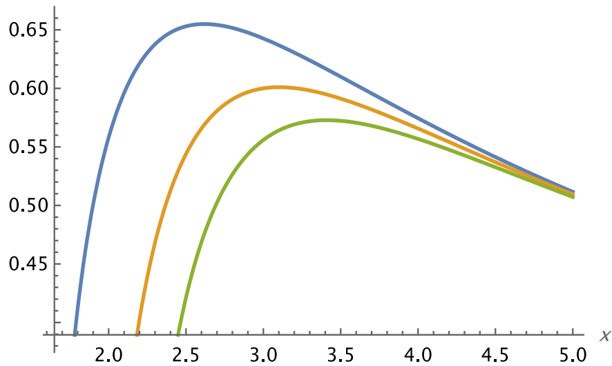
Figure 4.1. Interaction I. The function y = \frac{v^2(x)}{\sigma} for a point mass, if k = -0.01 . Source: Figure by author.
