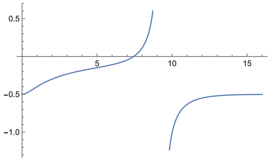
Figure 4.14. Interaction II. The function y = \frac{V(x)}{\sigma} for a point mass, if k = 0.1 . Source: Figure by author.
