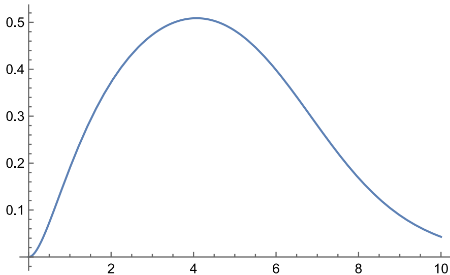
Figure 4.16. Interaction III. The function y = \frac{v^2(x)}{\sigma} for a point mass, if k = 0.1 . Source: Figure by author.
