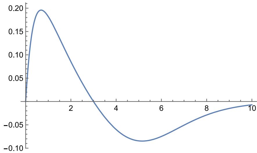
Figure 4.9. Interaction I. The function y = \frac{2GM}{\sigma^2} g(x) for a point mass, if k = 0.5 . Source: Figure by author.
