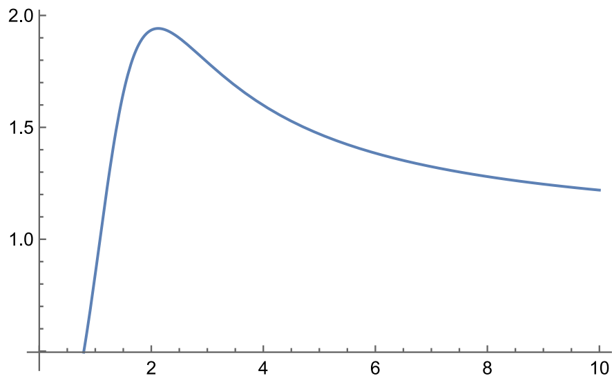
Figure 4.10. Interaction II. The function y = \frac{v^2(x)}{\sigma} for a point mass, if k = 0.5 . Source: Figure by author.
