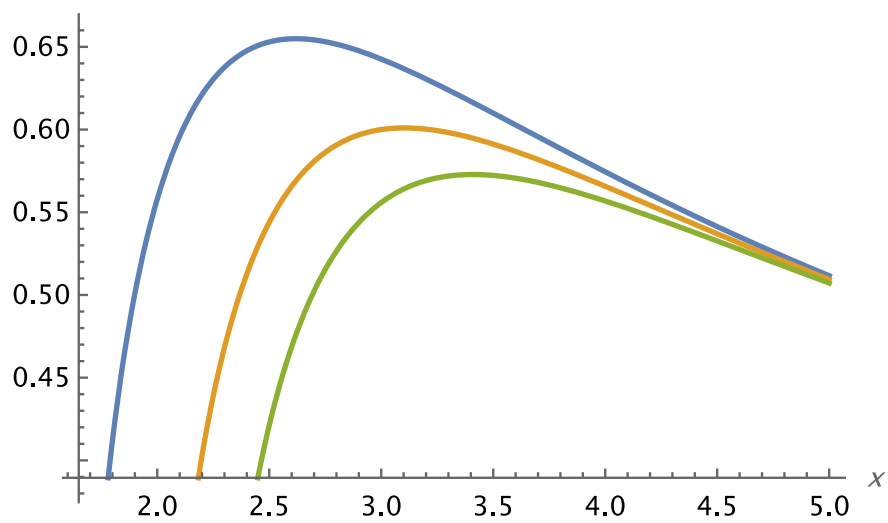
Figure 4.20. Interaction IV. The graph of the function y = \frac{V(x)}{\sigma} for a point mass, if k = -1 . Source: Figure by author.
