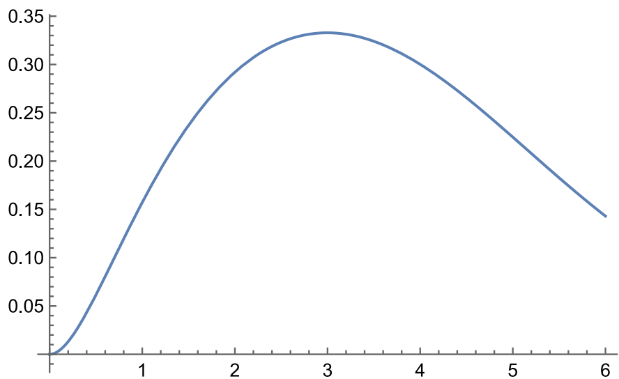
Figure 4.7. Interaction I. The function y = \frac{v^2(x)}{\sigma} for a point mass, if k = 0.5 . Source: Figure by author.
