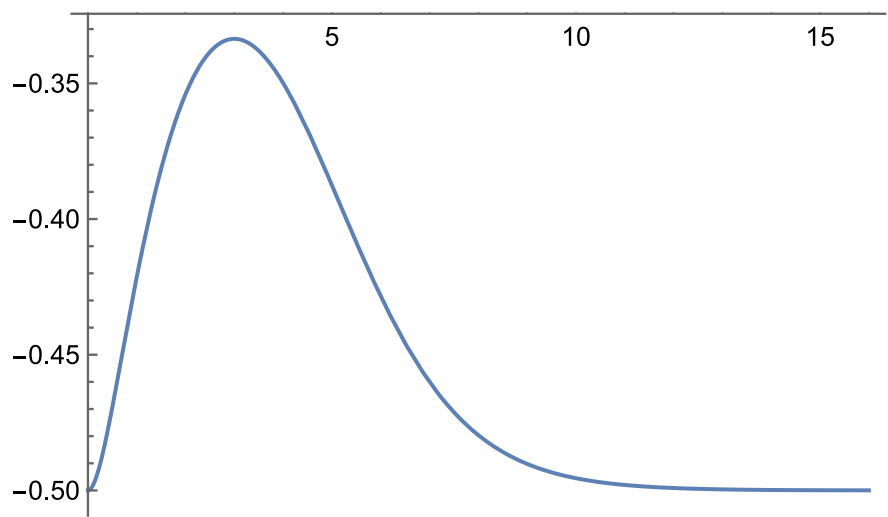
Figure 4.8. Interaction I. The function y = \frac{V(x)}{\sigma} for a point mass, if k = 0.5 . Source: Figure by author.
