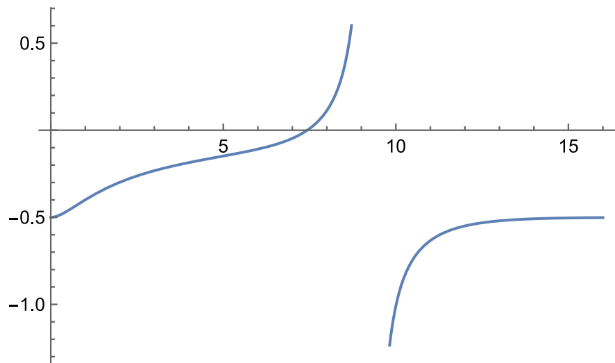
Figure 4.2. Interaction I. The function y = \frac{V(x)}{\sigma} for a point mass, if k = -0.01 . Source: Figure by author.
