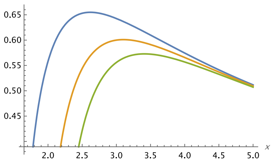
Figure 4.11. Interaction II. The function y = \frac{V(x)}{\sigma} for a point mass, if k = 0.5 . Source: Figure by author.
