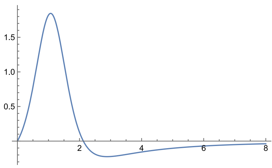
Figure 4.12. Interaction II. The function y = \frac{2GM}{\sigma^2} g(x) for a point mass, if k = 0.5 . Source: Figure by author.
