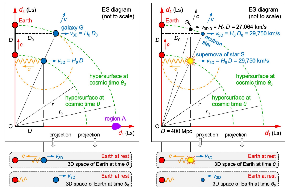
Figure 6. ER-based model of cosmology. The green arcs show parts of a 3D hypersurface. The orange circles show where most of the energy emitted by G or S at the time \theta is today at \theta_0 . Left: G recedes from O at the speed c and from the d_4 axis at the speed v_{3D} . Right: If S_0 happens to be at the same distance D today at which the supernova of S occurred, S_0 recedes more slowly from d_4 than S.
