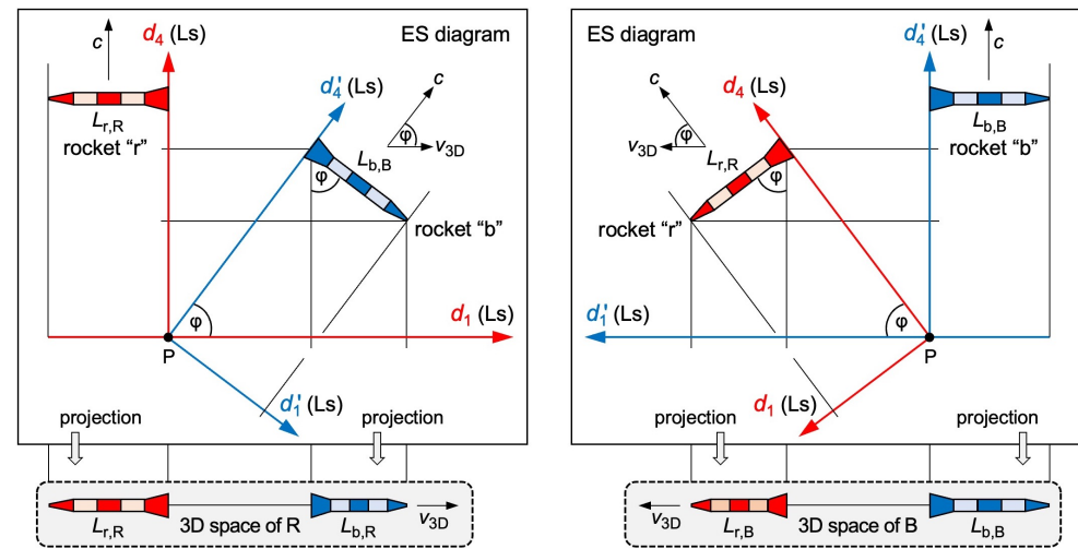
Figure 3. ES diagrams of two rockets "r" and "b". Observer R (or B) is in the rear end of "r" (or else "b"). Left: "r" moves in the d_4 axis. "b" moves in the d'_4 axis. In the 3D space of R, "b" contracts to L_{b,R} . Right: The ES diagram has been rotated only. In the 3D space of B, "r" contracts to L_{r,B} .
