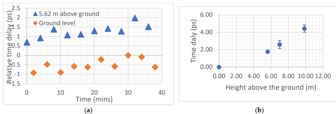
Figure 2. (a) Experimental results. Relative time delays measured at the ground level and at a height of 5.62 m above the ground level. Measurements were carried out in every 2 minutes and repeated 10 times. (b) Measured time delays as a function of heights above the ground.
