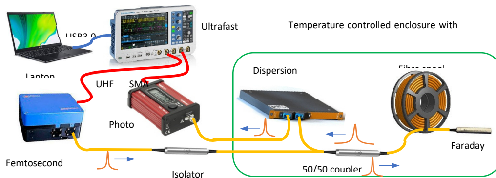
Figure 1. A schematic diagram of the experimental setup for measuring dependence of the speed of light on the gravitational field.
