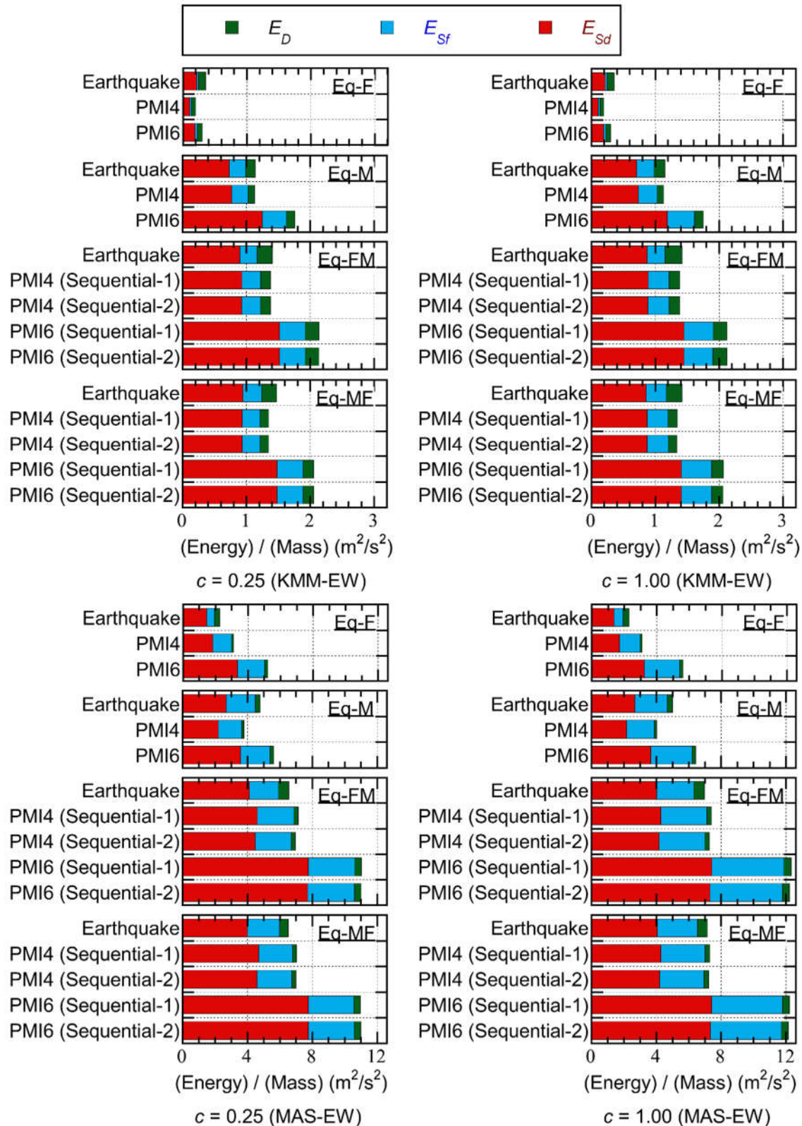
Figure 8. Comparisons of cumulative energy.
