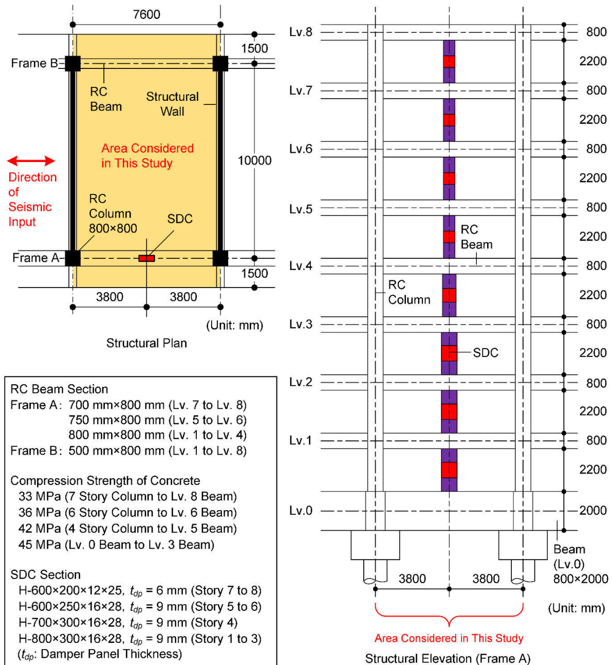
Figure 3. Building model.
