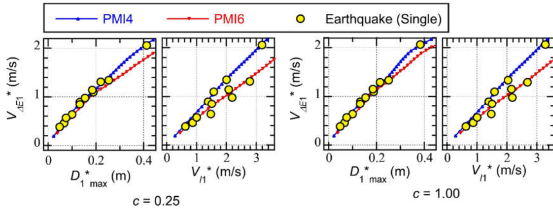
Figure 14. V_{\Delta E1}^* - D_{1\max}^* and V_{\Delta E1}^* - V_{I1}^* relationship.
