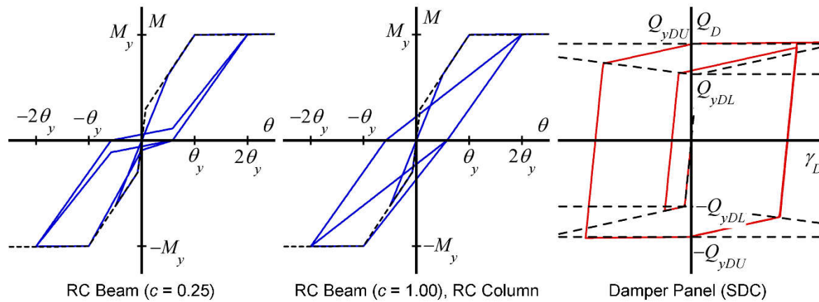
Figure 4. Hysteresis rule of RC members and SDCs.
