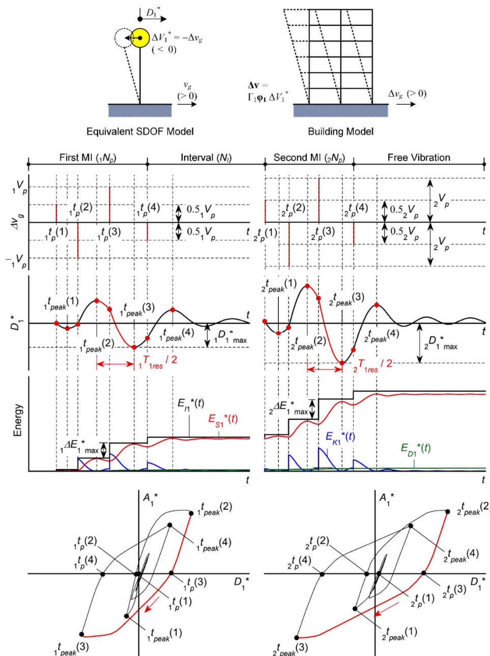
Figure 1. Extended critical PMI analysis considering sequential input (in case of 1N_p = 2N_p = 4 ).
