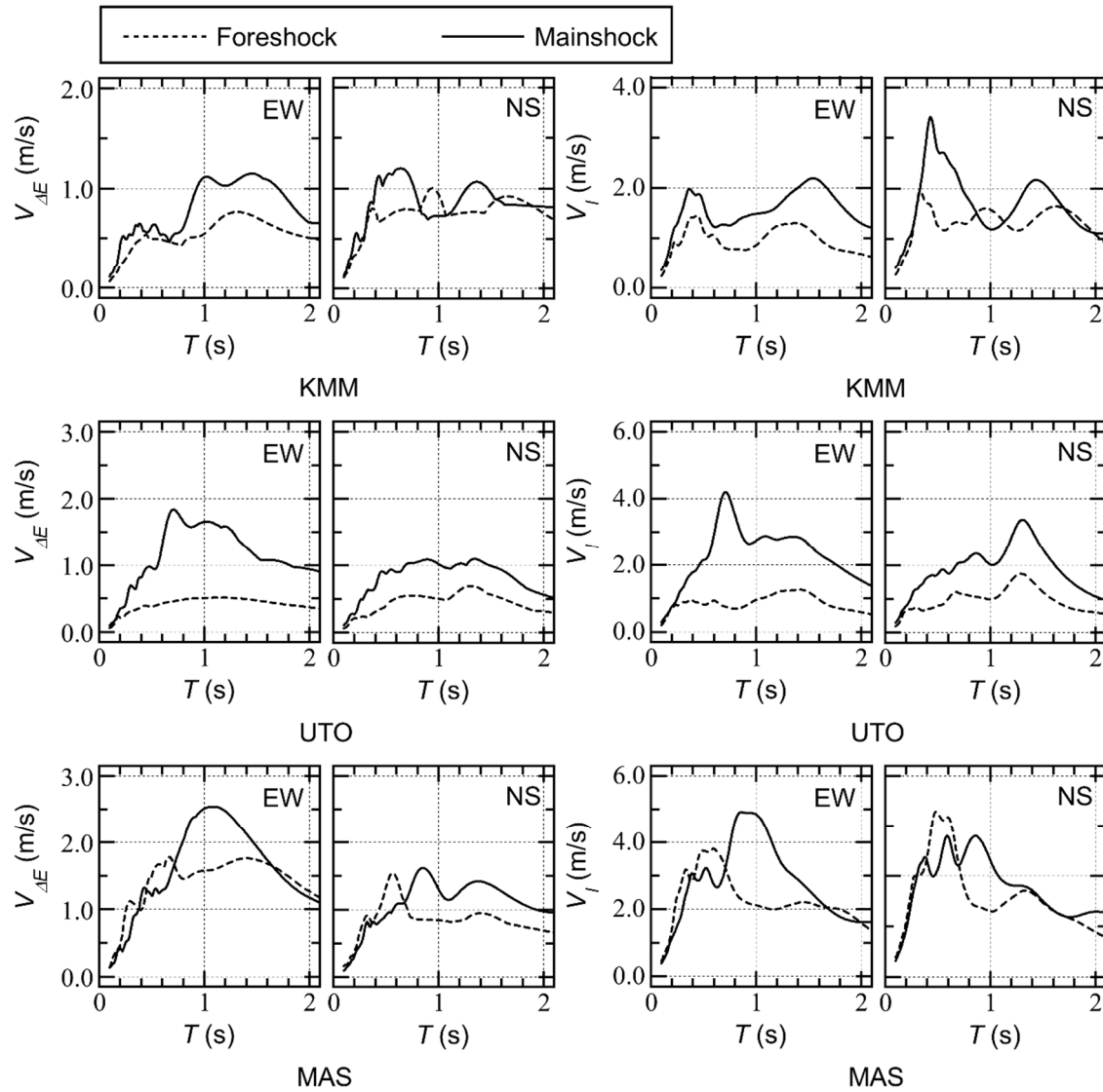
Figure 5. V_{\Delta E} and V_I spectrum of ground motion set.
