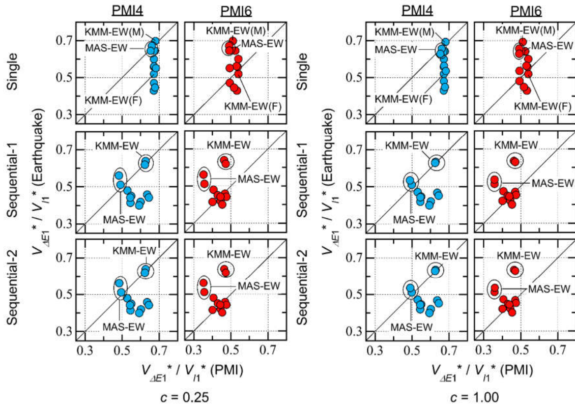
Figure 15. Relationship between the (V_{\Delta E1}^* / V_{I1}^*) ratio obtained using recorded ground motions and that obtained from critical PMI analysis.
