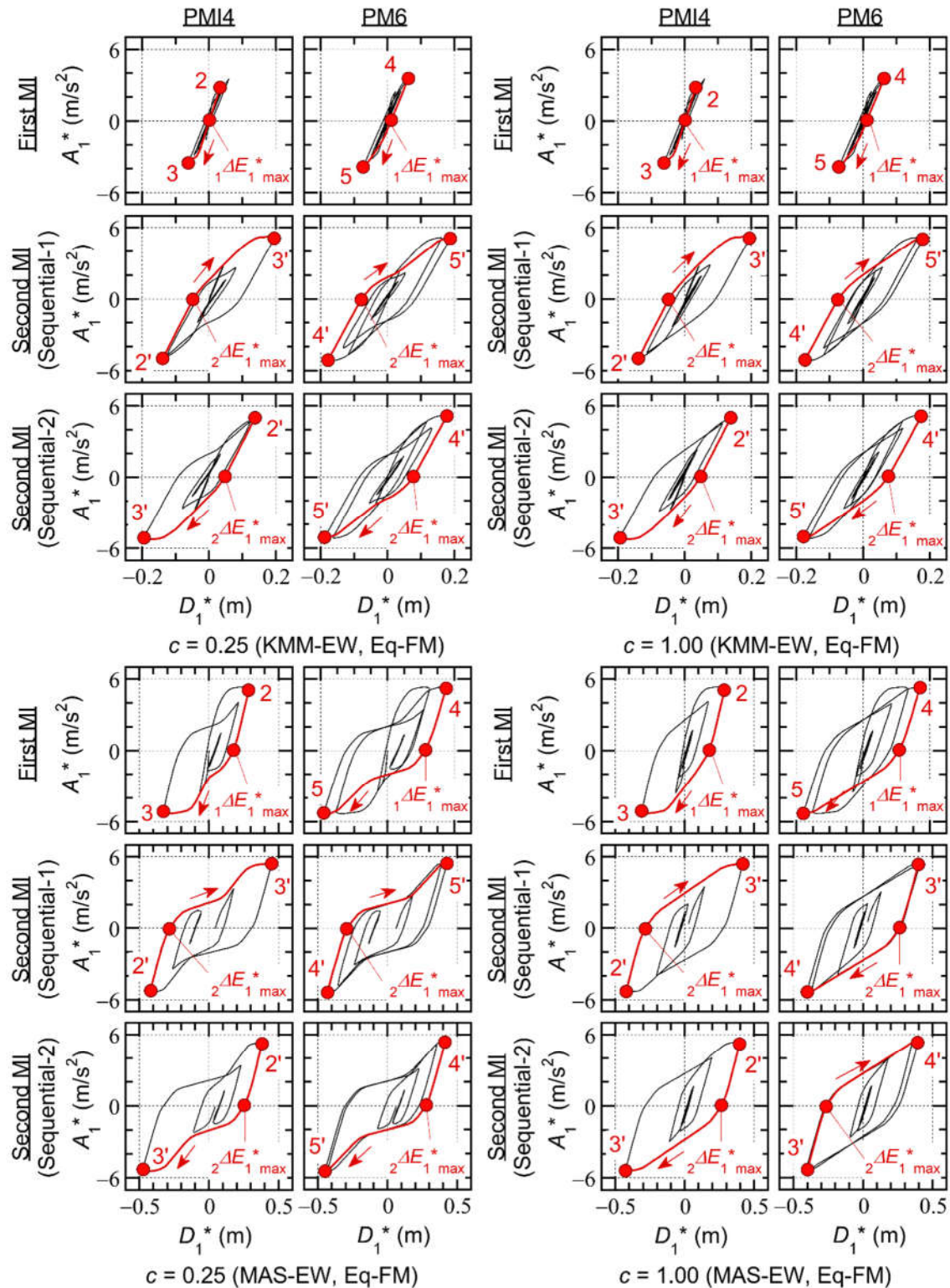
Figure 7. Hysteresis loop obtained from PMI analysis.
