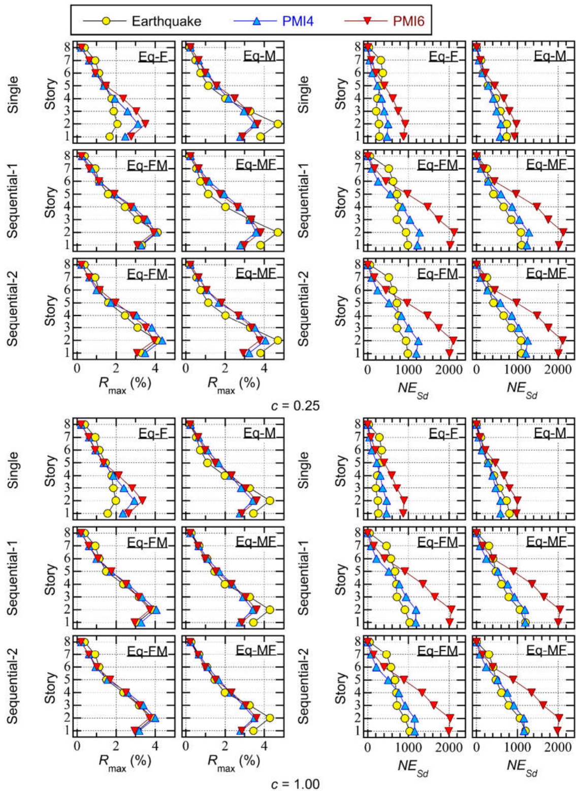
Figure 10. Comparisons of local response (MAS-EW).
