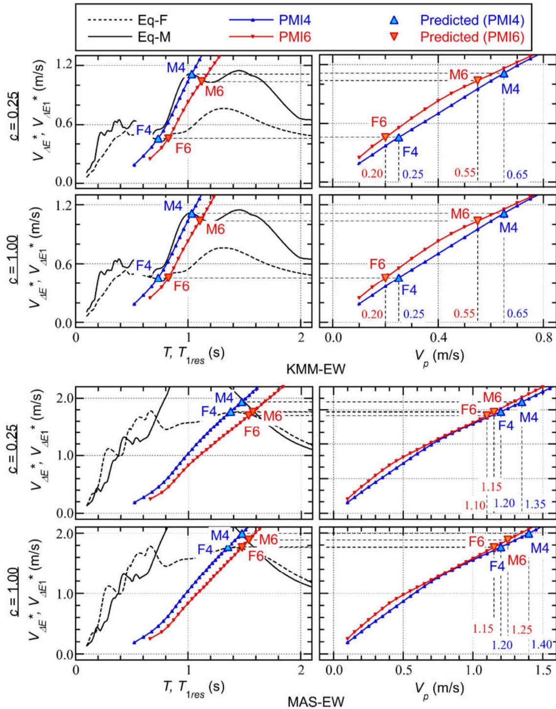
Figure 6. Evaluation of {}_1V_p and {}_2V_p .
