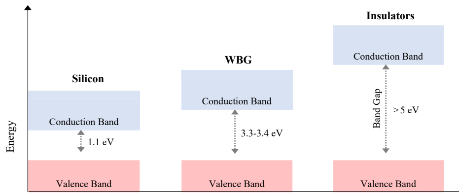
Figure 6. Simplified Energy Diagram and Band Gap Energy of Si, WBG, and Insulators.
