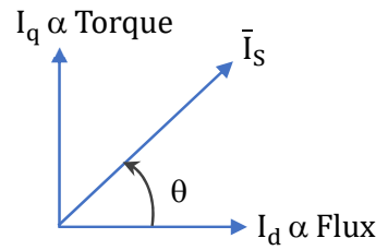
Figure 7. Phasor diagram of stator current components with FOC.
