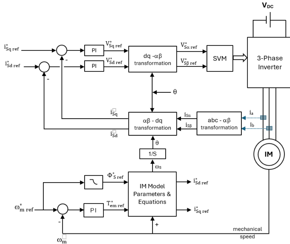
Figure 8. Block Diagram of the Basic Scheme of FOC of IM Drives.
