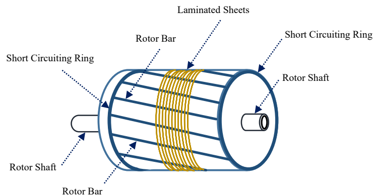
Figure 5. Rotor of a Squirrel Cage 3-F Induction Motor.
