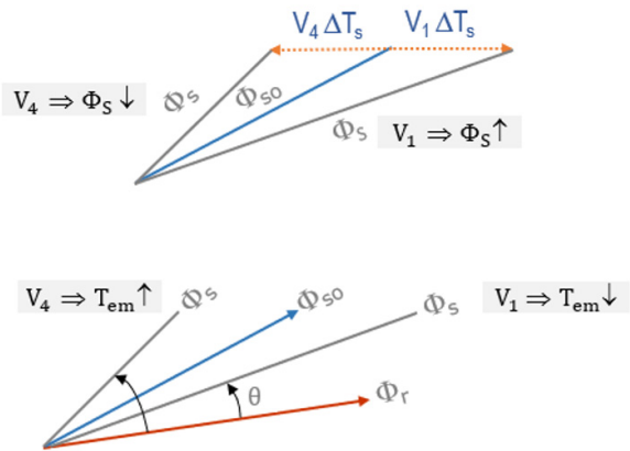
Figure 11. Control of Motor Stator Flux and Torque In Sector 1.
