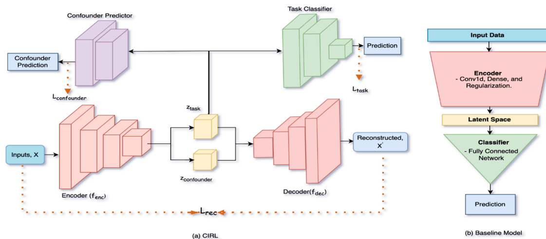
Figure 4. (a) Overview of the proposed disentangled autoencoder (CIRL) architecture. The input data ( X ) is passed through the encoder f_{enc} , which generates two disentangled latent representations: z_{task} and z_{confounder} . These representations are used by the decoder f_{dec} for reconstruction, on the other hand z_{task} used by the task classifier and confounder predictor for their respective outputs. The overall training is governed by the loss functions \mathcal{L}_{rec} , \mathcal{L}_{task} and \mathcal{L}_{confounder} , combined into \mathcal{L}_{total} . (b) The architecture of the baseline model. The baseline model was designed to isolate the effect of CIRL's architecture. It uses an encoder and task classifier identical to CIRL's but lacks the decoder, the split latent space, and the adversarial confounder predictor, mapping all features to a single latent space. This ensures a fair comparison where performance gains can be directly attributed to the proposed disentanglement mechanism.
