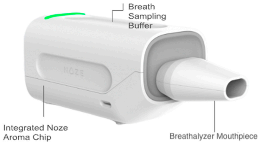
Figure 3. The DiagNoze breathalyzer setup used for the experiments conducted on human breath.
