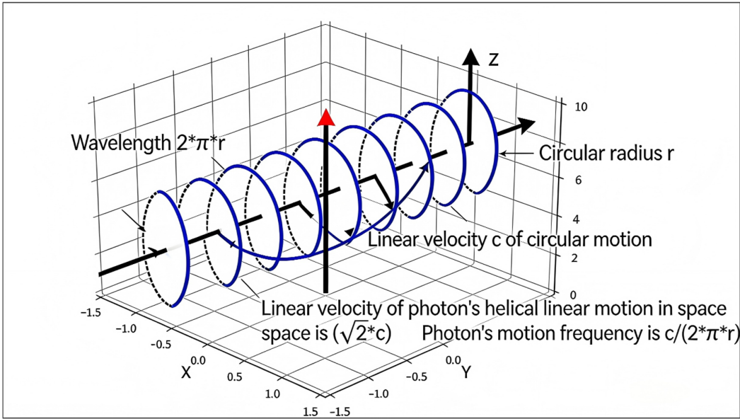
8.1. Figure 1: Schematic Diagram of the Geometric Trajectory and Key Parameters of Photon Uniform Helical Linear Motion
