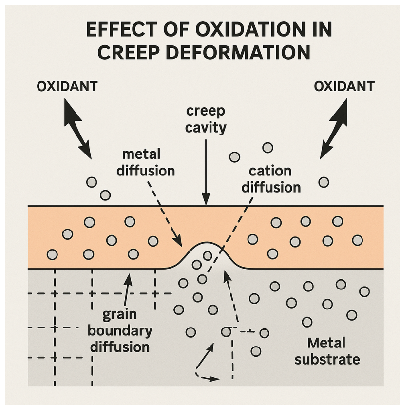
Figure 27. Effect of Oxidation in Creep Deformation
