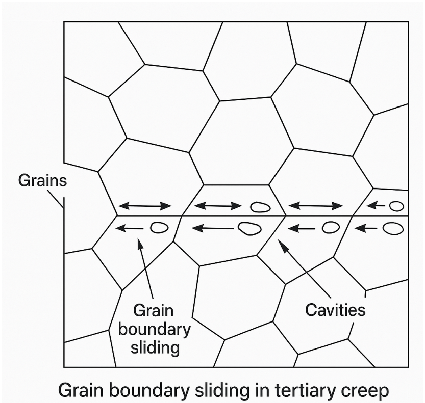
Figure 24. Grain Boundary Sliding in Tertiary Creep
