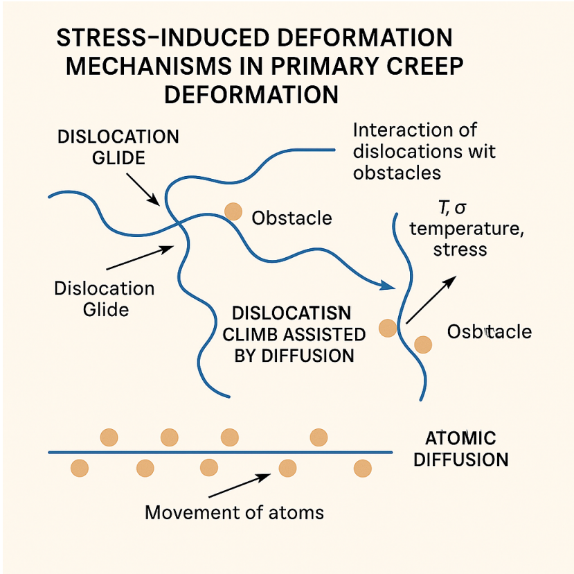
Figure 15. Stress-induced Deformation in Primary Creep
