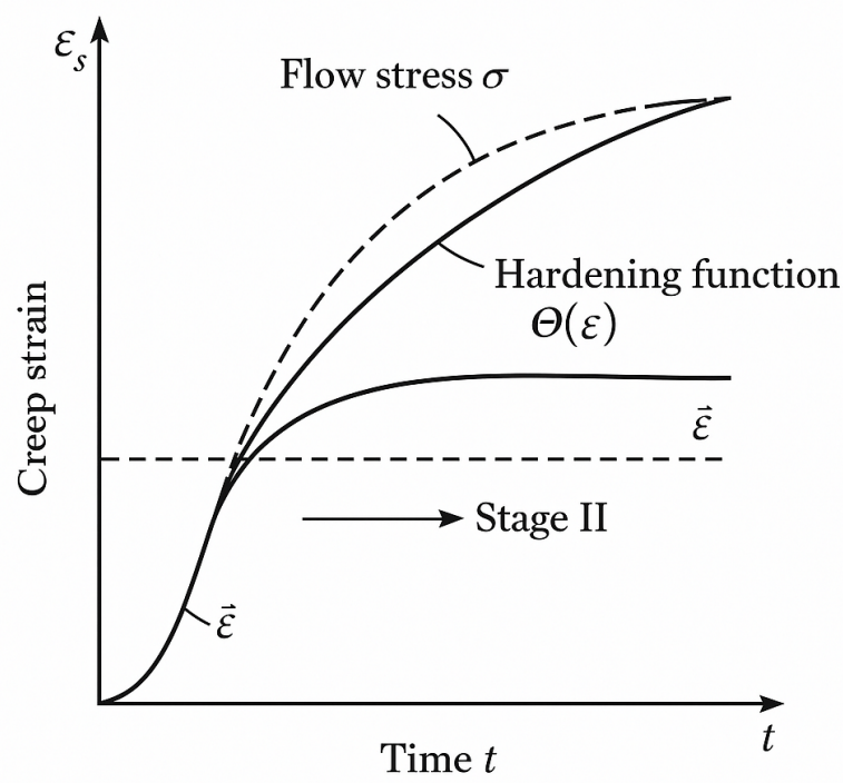
Figure 18. Work Hardening in Secondary Creep
