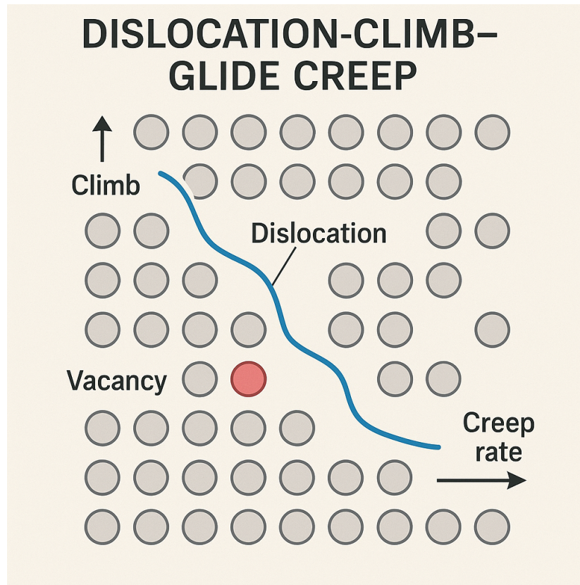
Figure 11. Dislocation Climb-Glide Creep
