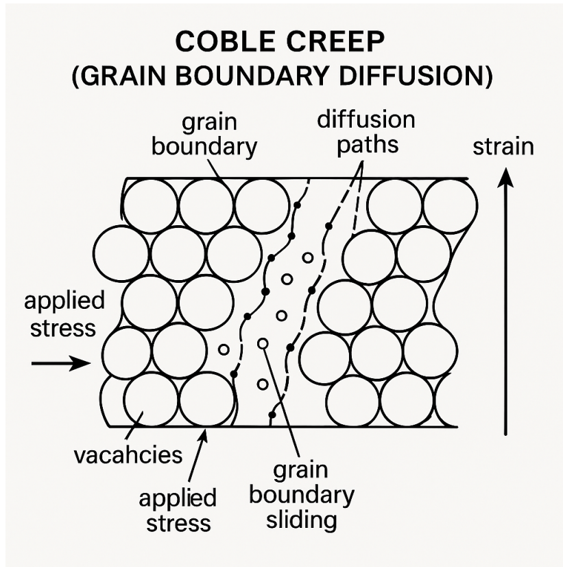
Figure 2. Coble Creep (Grain Boundary Diffusion)
