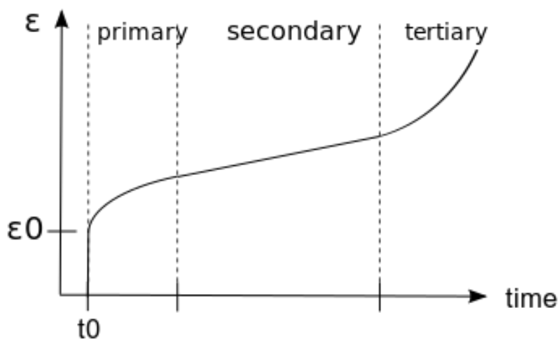
Figure 14. 3 Stages of Creep (Reference: By Strafpeloton2 - Own work, CC0, https://commons.wikimedia.org/w/index.php?curid=8138618 )
