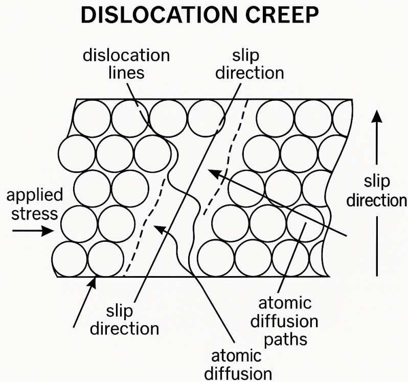
Figure 3. Dislocation Creep
