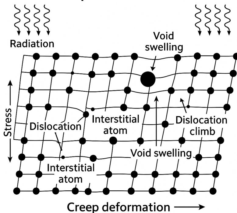
Figure 28. Effect of Irradiation in Creep Deformation
