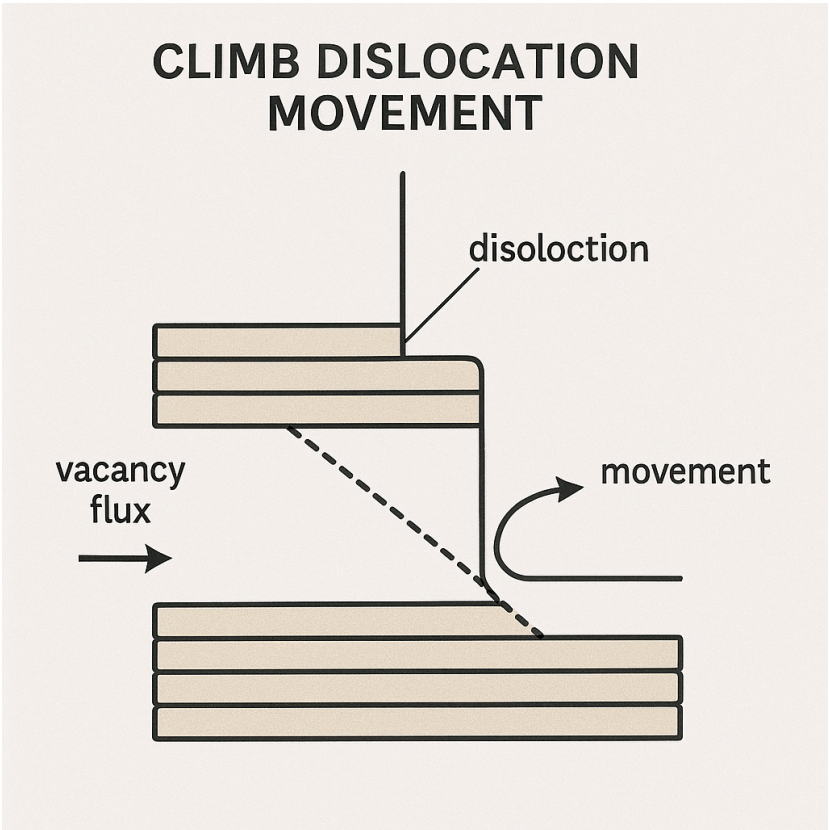
Figure 6. Climb Dislocation Movement
