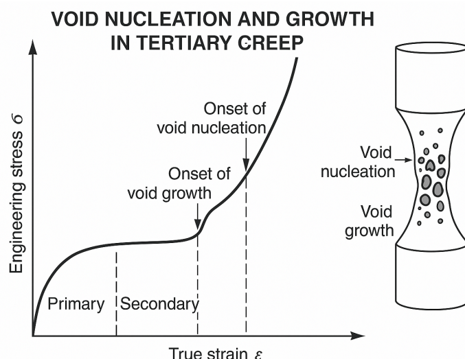
Figure 22. Void Nucleation and Growth in Tertiary Creep
