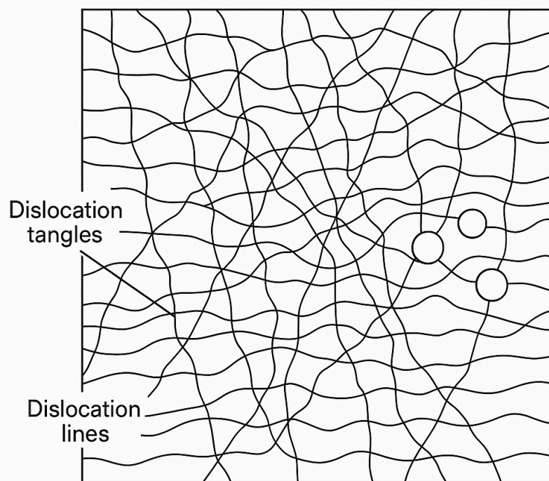
Dislocation networks in secondary creep
