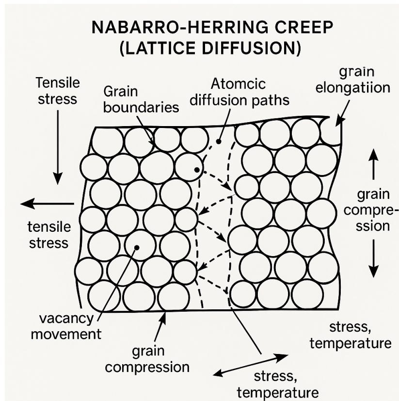
Figure 1. Nabarro-Herring Creep (Lattice Diffusion)
