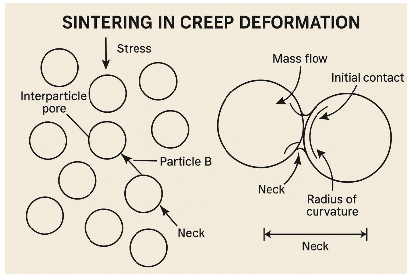
Figure 26. Sintering in Creep Deformation
