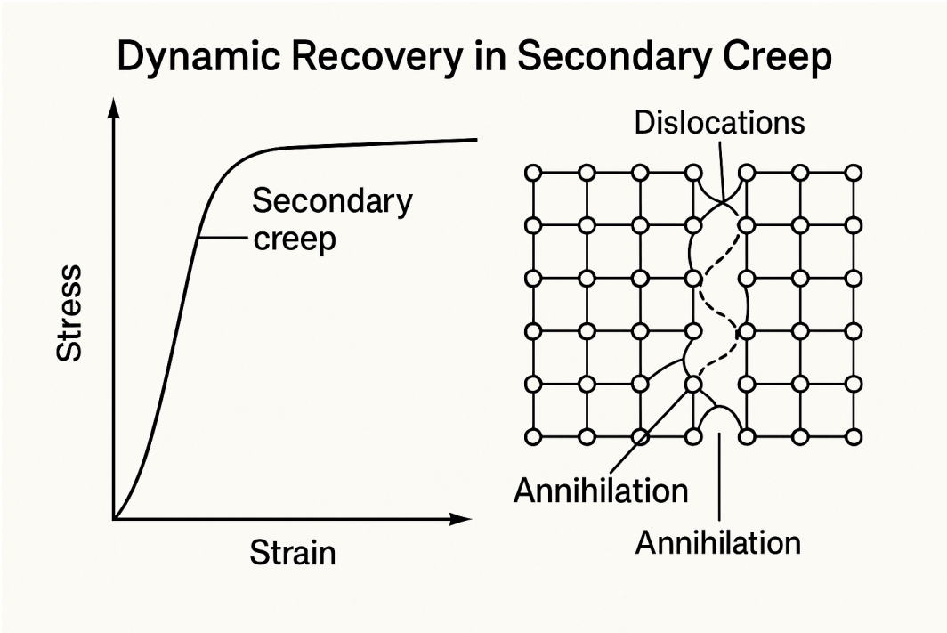
Figure 19. Dynamic Recovery in Secondary Creep
