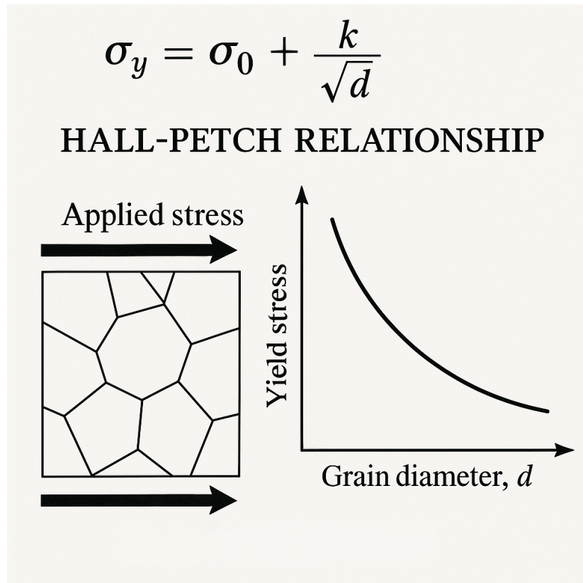
Figure 9. Hall-Petch Relationship
