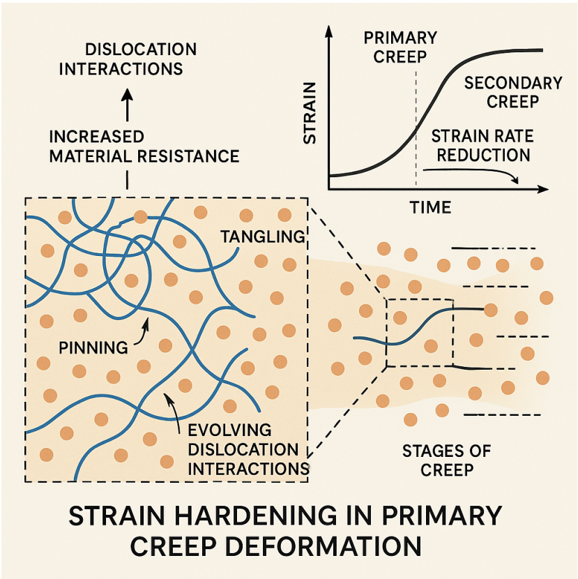
Figure 16. Strain Hardening in Primary Creep
