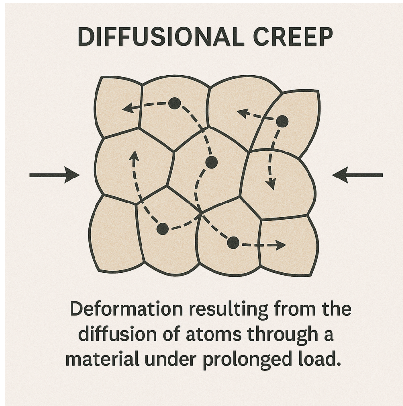
Figure 8. Diffusional creep
