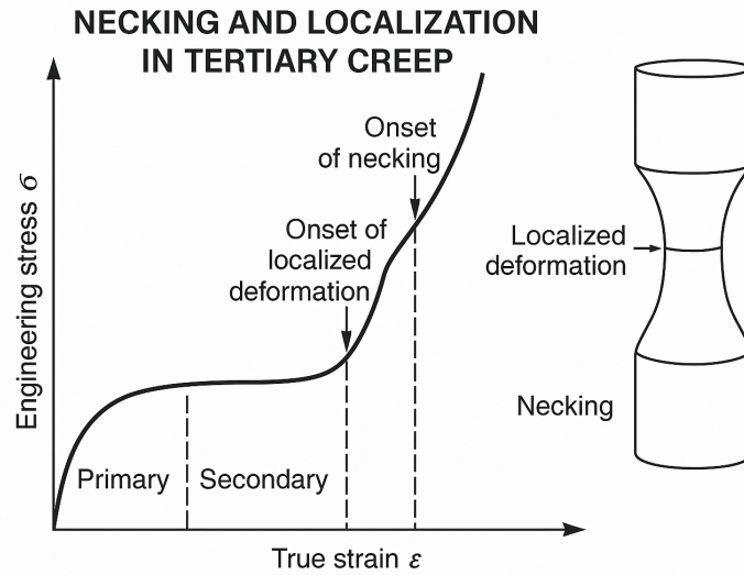
Figure 25. Necking and Localization in Tertiary Creep
