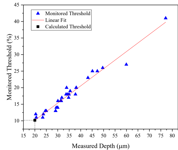
Figure 12. Threshold calculated for a depth of 20 \mu\text{m} .
