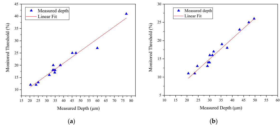
Figure 11. Depth and threshold of monitored defects: (a) Batch 1; (b) Batch 2.
