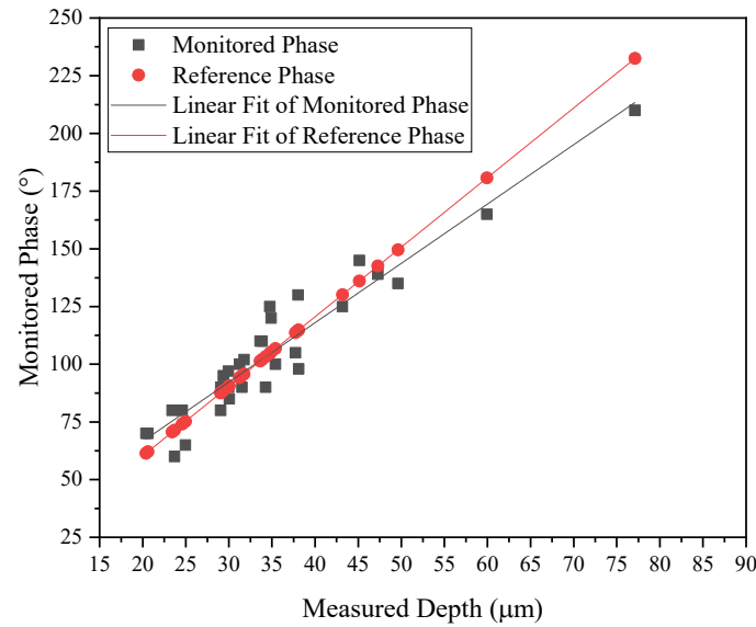
Figure 15. Comparison between measured phase signal and reference phase signal using RMSE.
