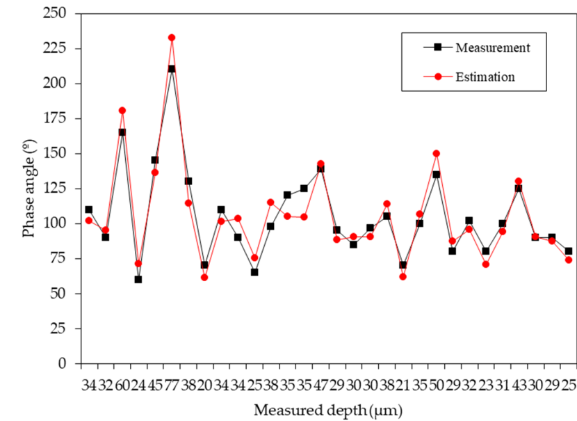
Figure 14. Comparison between measured phase signal and reference phase signal.
