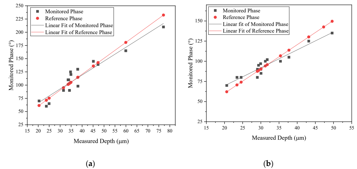
Figure 13. Depth and phase angle signal of monitored defects: (a) Batch 1; (b) Batch 2.
