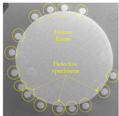
Figure 5. Defects detected under scanning electron microscope.
