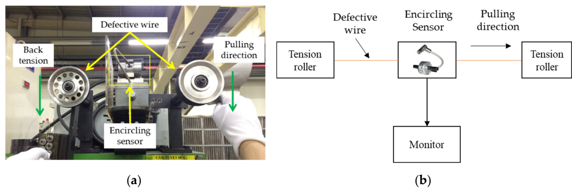
Figure 4. (a) Position of encircling sensor; (b) Block diagram of experiment.
