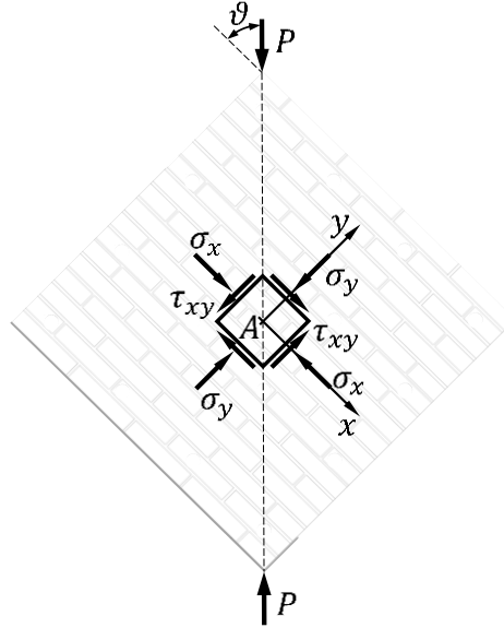
Figure 1. Normal and shear stresses in the infinitesimal neighborhood of the center of gravity, A , of the masonry wallette.
