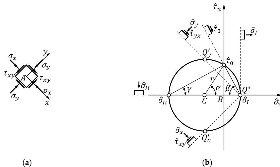
Figure 3. Stress state for the infinitesimal neighborhood of point A in: (a) the reference frame of Figure 1; (b) the modified Mohr plane of origin B, according to the RILEM interpretation of the diagonal compression test.
