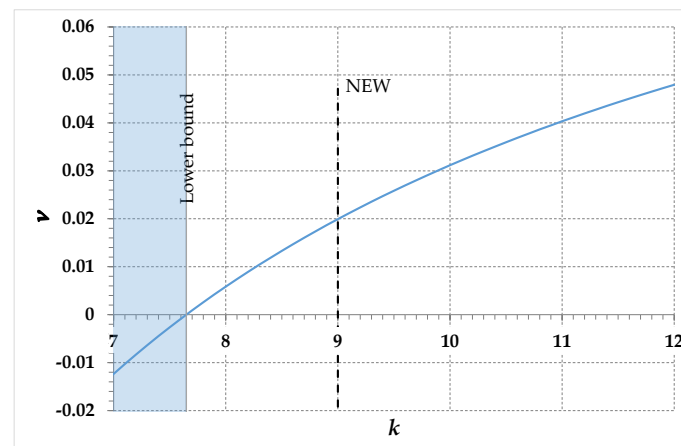
Figure 14. Detail of the relationship between the Poisson ratio, \nu , and the parameter k , in the range 7 \leq k \leq 12 .
