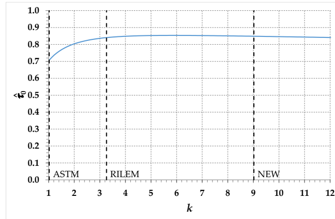
Figure 10. Plot of the normalized pure shear stress, \hat{\tau}_0 , as a function of the parameter k .
