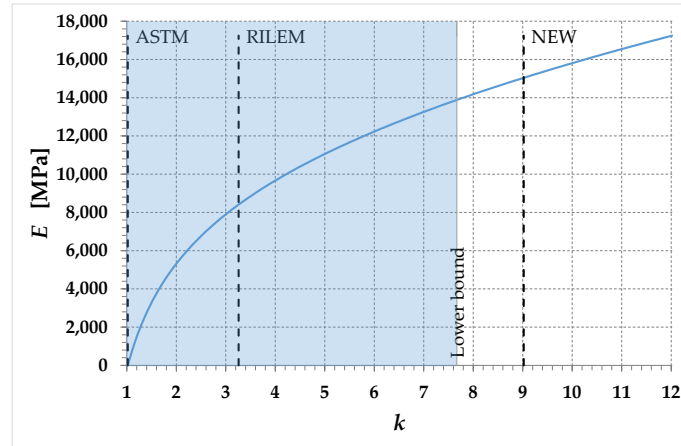
Figure 11. Plot of the Young modulus, E , as a function of the parameter k .
