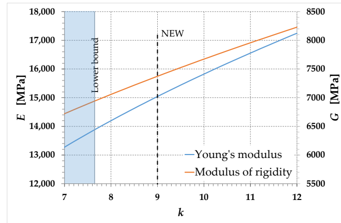
Figure 13. Detail of the relationship between the Young modulus, E , and the parameter k , in the range 7 \leq k \leq 12 .
