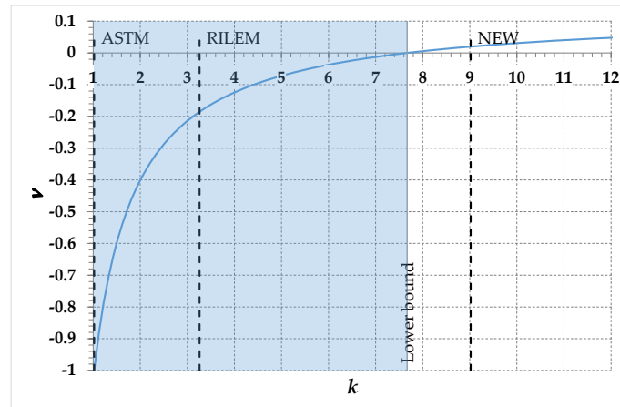
Figure 12. Plot of the Poisson ratio, \nu , as a function of the parameter k .
