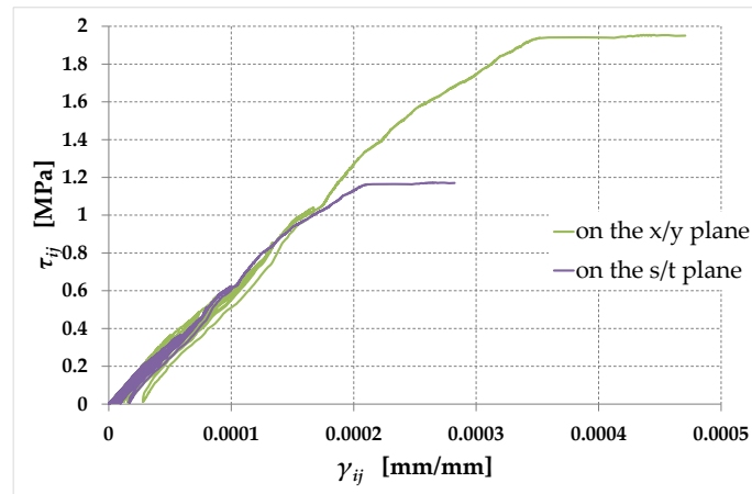
Figure 16. Shear stress–shear strain curves for the new interpretations of the diagonal compression test, in the x/y and s/t planes.
