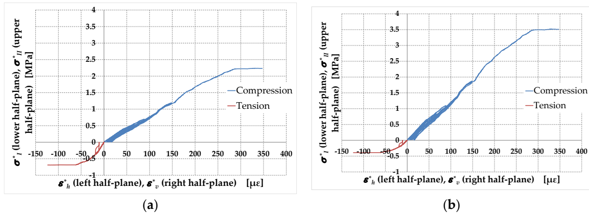
Figure 17. Stress-strain relationships along the principal directions of stress and strain, for: (a) the RILEM interpretation of the diagonal compression test; (b) the new interpretation of the diagonal compression test.
