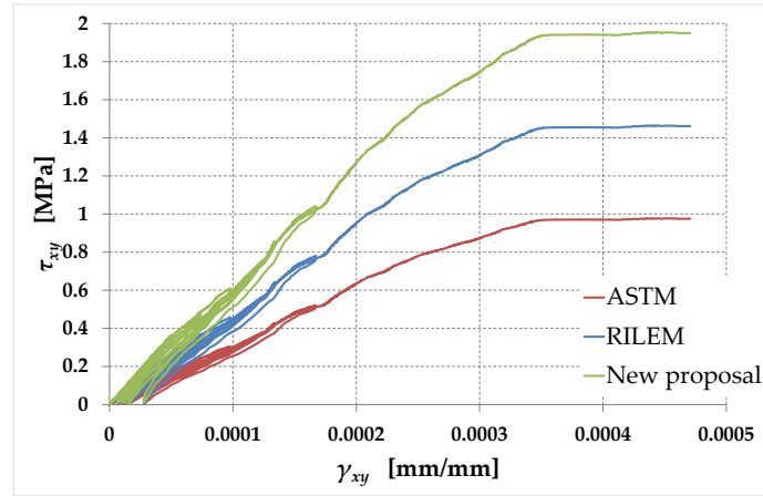
Figure 15. Shear stress–shear strain curves for the ASTM, RILEM and new interpretations of the diagonal compression test ( x/y plane).
