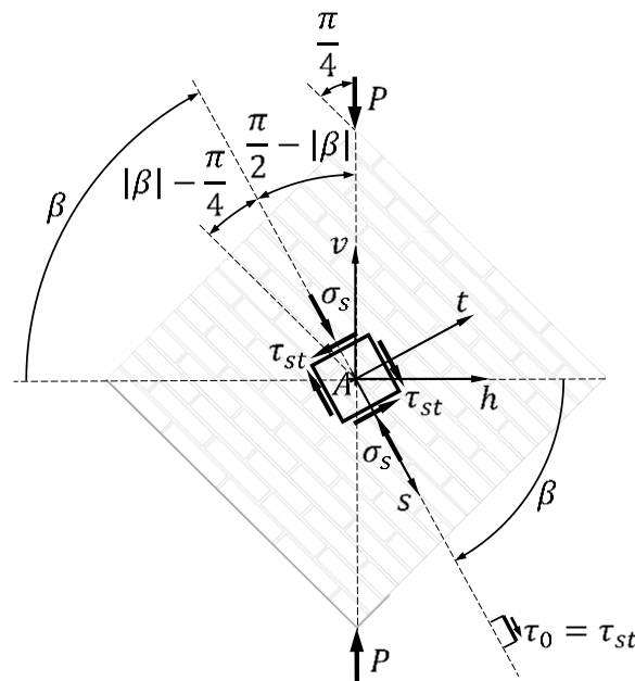
Figure 7. Stress state of an elementary cube with faces parallel and orthogonal to the trace with positive pure shear stress.
