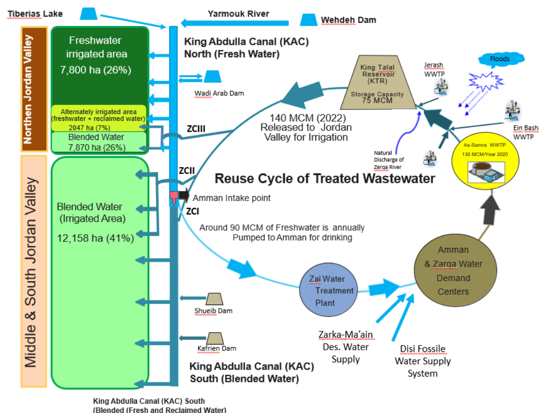
Figure 1. Reuse cycle of treated wastewater.
