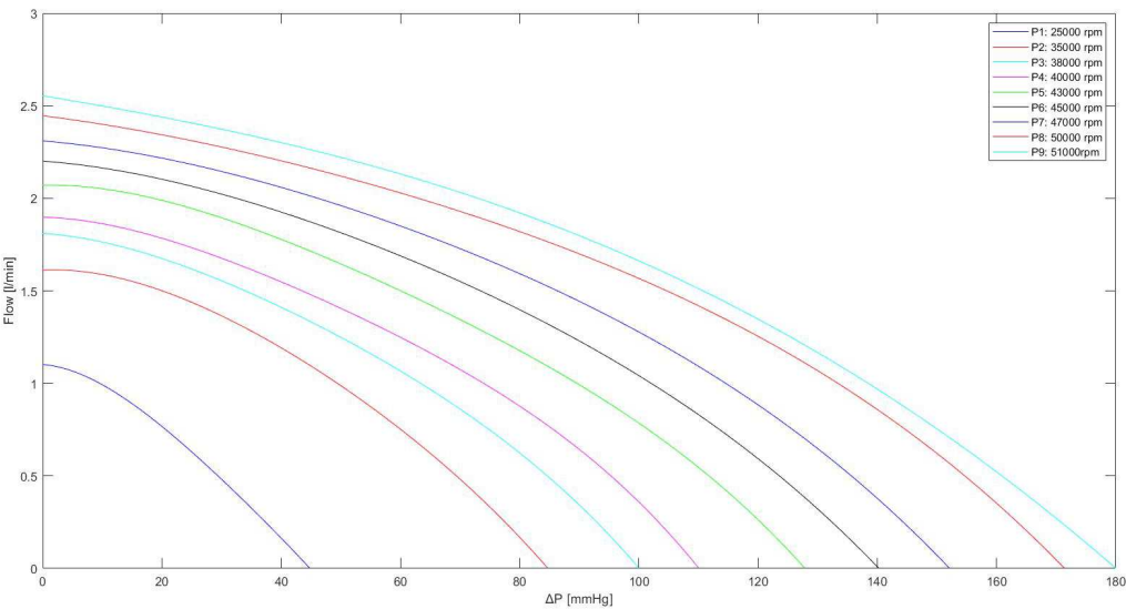
Figure 4. Relationship between the flow through the Impella 2.5 pump and the pressure difference for different rotational speeds. The curves were obtained using equation (3) with the values listed in Table 1.
