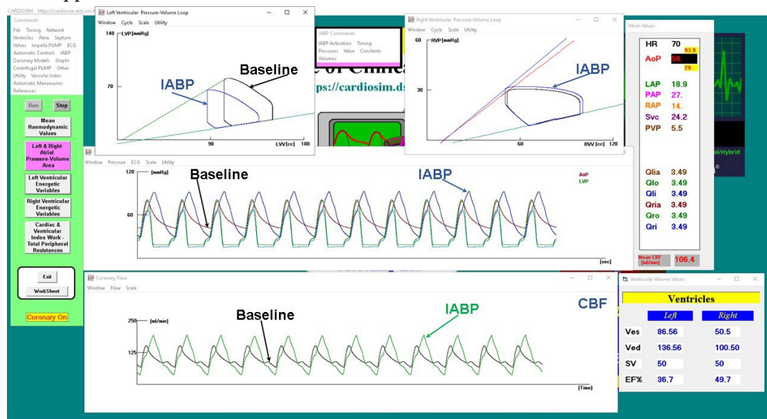
Figure 10. CARDIOSIM® screenshot showing baseline and assisted conditions with IABP. Proceeding from the top left to the right and then down, the left (top left side) and right (top right side) ventricular pressure-volume loops for baseline and IABP support are observed. The left ventricular and aortic pressure waveforms for baseline (red line) and IABP assistance (blue line) are plotted in the middle window. The bottom window shows the coronary blood flow waveforms.
