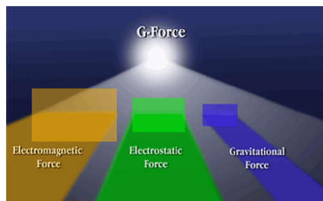
Figure 1. The three forces are manifestations of the one Gforce. The charges and mass could be depicted as three colored glass panes through which we view a light. The same light illuminates each pane of glass, even though each color is different.
