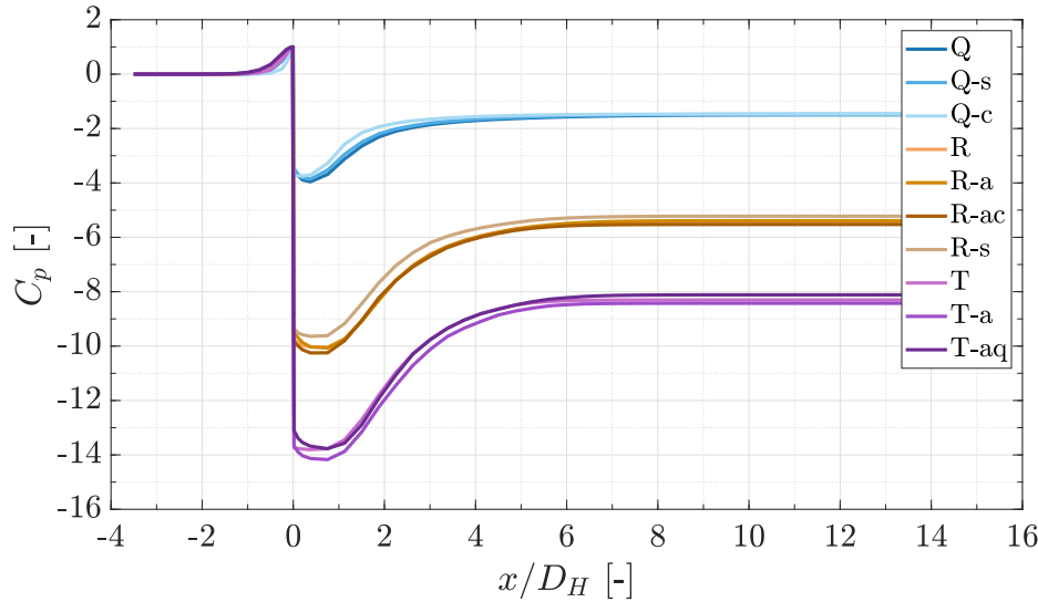
Figure 9. Modulus configuration, \alpha = 0^\circ . Total pressure coefficient C_p as a function of the normalised streamwise distance x/D_H for all tested geometries; sampling along the central bulk line.
