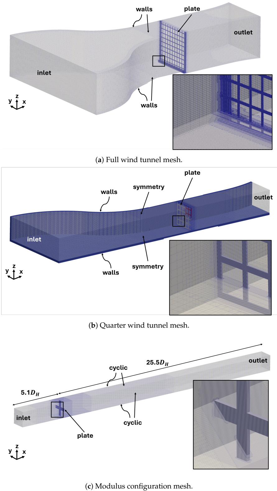
Figure 4. Meshes and computational domain employed along with a zoom to highlight refinement near the walls.
