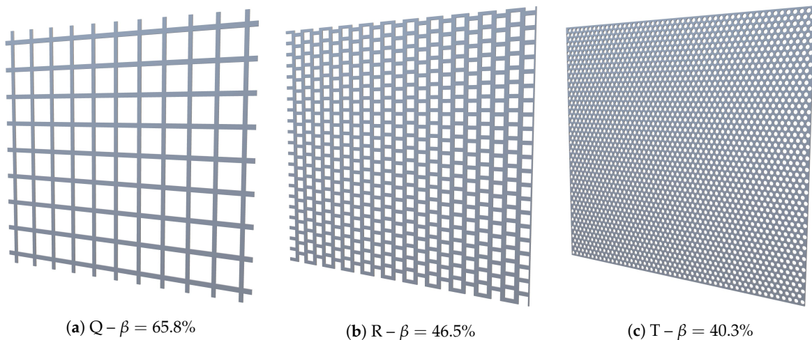
Figure 2. CAD model of the three tested plates.
