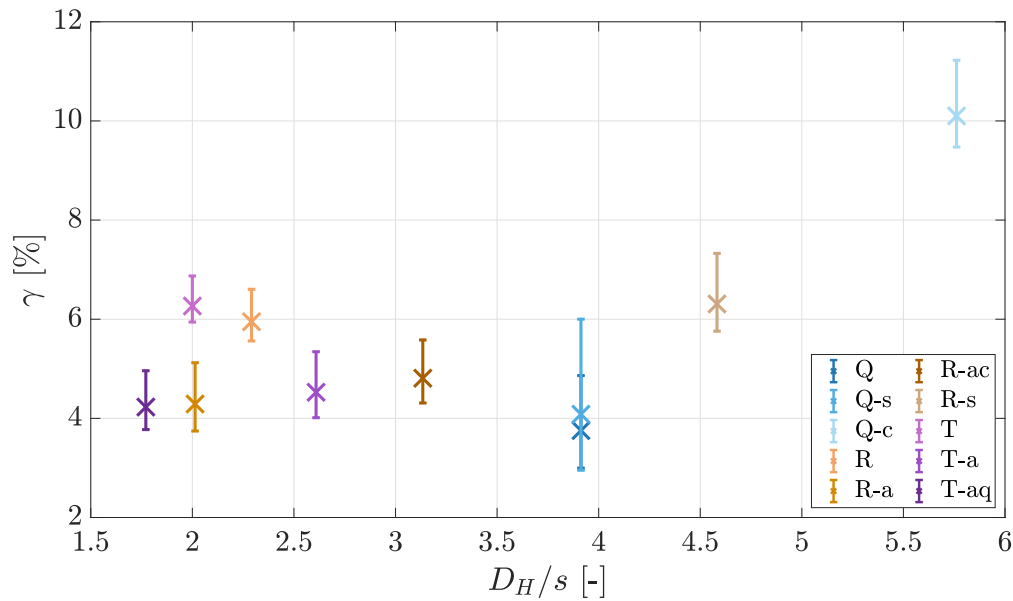
Figure 8. Pressure correction coefficient \gamma for all tested geometries, plotted against the non-dimensional spacing D_H/s . Each geometry is colour-coded by porosity: blue ( \beta = 65.8\% ), yellow ( \beta = 46.5\% ), and purple ( \beta = 40.3\% ). Error bars reflect measurements repeated at different wind speeds.
