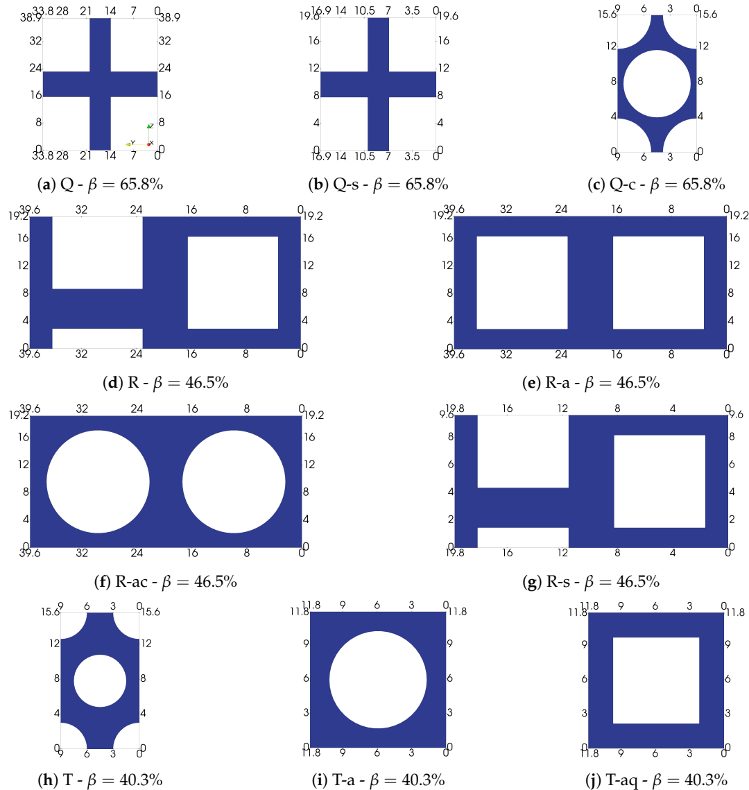
Figure 5. Geometries of the ten considered moduli simulated in cyclic conditions. Dimensions in millimetres.
