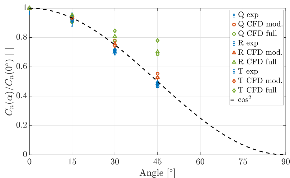
Figure 11. Drag coefficient reduction C_n(\alpha)/C_n(0^\circ) against wind attack angle \alpha . Comparison between experimental test (blue), CFD modulus configuration (orange), CFD full WT (green).
