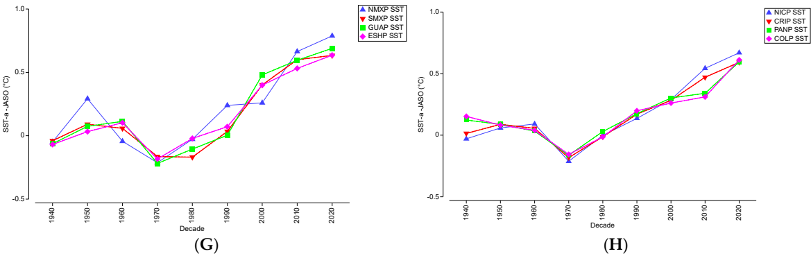
Figure 6. Spatio-temporal variation in country-level decadal means of JASO sea surface temperature anomalies: (a) Western Caribbean, (b) Southwestern Caribbean, (c) Southern Caribbean, (d) Eastern Caribbean, (e) Northern Caribbean, (f) Northwestern Caribbean, (g) Northeastern tropical Pacific, (h) Southeastern tropical Pacific. Country acronyms described in Table S1.
