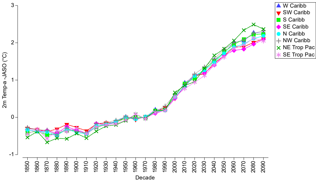
Figure 7. Projected spatio-temporal variation in decadal JASO regional mean 2m temperature anomaly across the wider Caribbean and eastern tropical Pacific regions between 1851 and 2100 based on Scenario 4.5.
