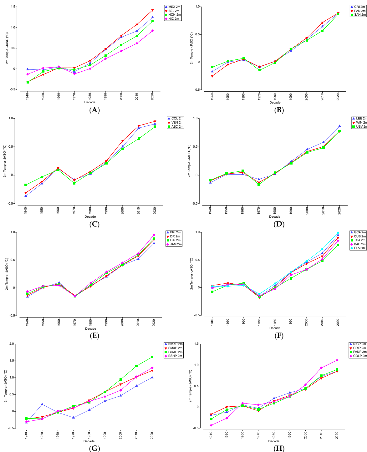
Figure 5. Spatio-temporal variation in country-level decadal means of JASO surface (2m) temperature anomalies: (a) Western Caribbean, (b) Southwestern Caribbean, (c) Southern Caribbean, (d) Eastern Caribbean, (e) Northern Caribbean, (f) Northwestern Caribbean, (g) Northeastern tropical Pacific, (h) Southeastern tropical Pacific. Country acronyms described in Table S1.
