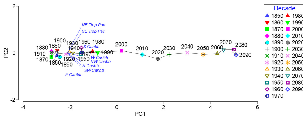
Figure 10. Principal component analysis (PCA) of the projected mean decadal variation in JASO sea surface temperature anomaly across the wider Caribbean and eastern Pacific regions between 1851 and 2100 based on Scenario 4.5. This solution explains 99.9% of the observed variation.
