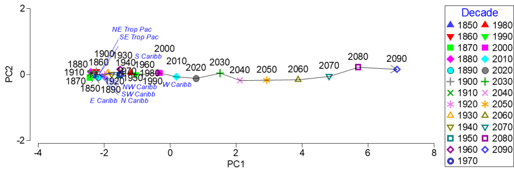
Figure 12. Principal component analysis (PCA) of the projected mean decadal variation in JASO 2m temperature anomaly across the wider Caribbean and eastern Pacific regions between 1851 and 2100 based on scenario 8.5. This solution explains 100% of the observed variation.
