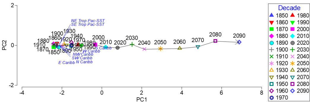
Figure 14. Principal component analysis (PCA) of the projected mean decadal variation in JASO sea surface temperature anomaly across the wider Caribbean and eastern Pacific regions between 1851 and 2100 based on scenario 8.5. This solution explains 100% of the observed variation.
