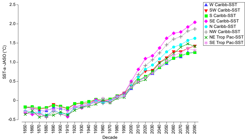
Figure 9. Projected spatio-temporal variation in decadal JASO regional mean sea surface temperature anomaly across the wider Caribbean and eastern tropical Pacific regions between 1851 and 2100 based on Scenario 4.5.
