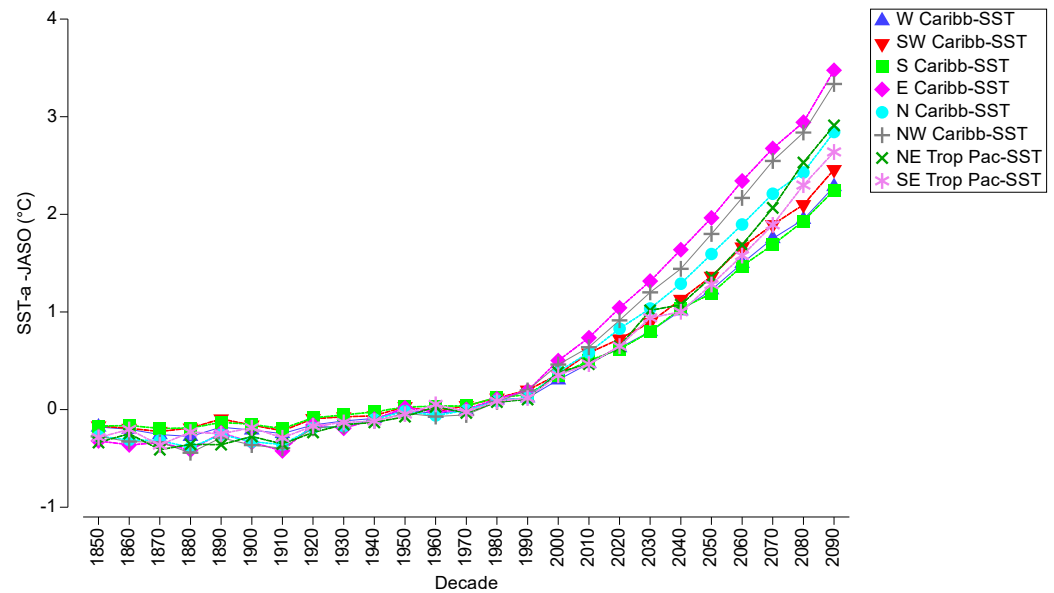
Figure 13. Projected spatio-temporal variation in decadal JASO regional mean sea surface temperature anomaly across the wider Caribbean and eastern tropical Pacific regions between 1851 and 2100 based on scenario 8.5.
