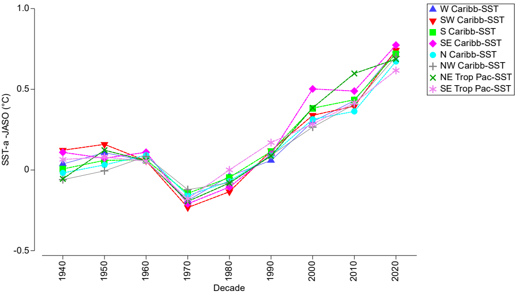
Figure 4. Spatio-temporal variation in decadal JASO regional mean sea surface temperature anomaly (SST-a) across the wider Caribbean and eastern Pacific regions between 1940 and 2023.
