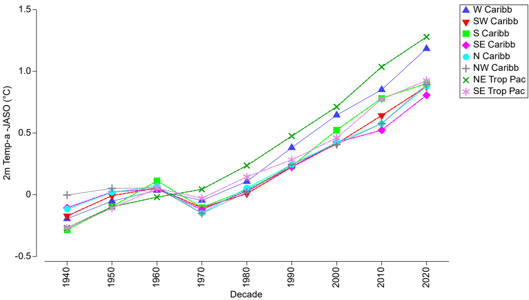
Figure 3. Spatio-temporal variation in decadal JASO regional mean surface (2m) temperature anomaly across the wider Caribbean and eastern Pacific regions between 1940 and 2023.
