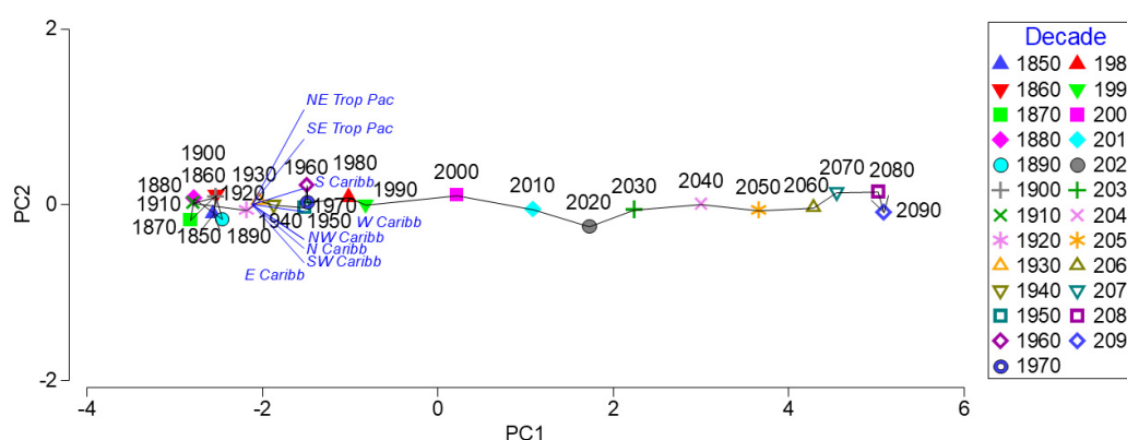
Figure 8. Principal component analysis (PCA) of the projected mean decadal variation in JASO 2m temperature anomaly across the wider Caribbean and eastern Pacific regions between 1851 and 2100 based on Scenario 4.5. This solution explains 99.9% of the observed decadal variation.
