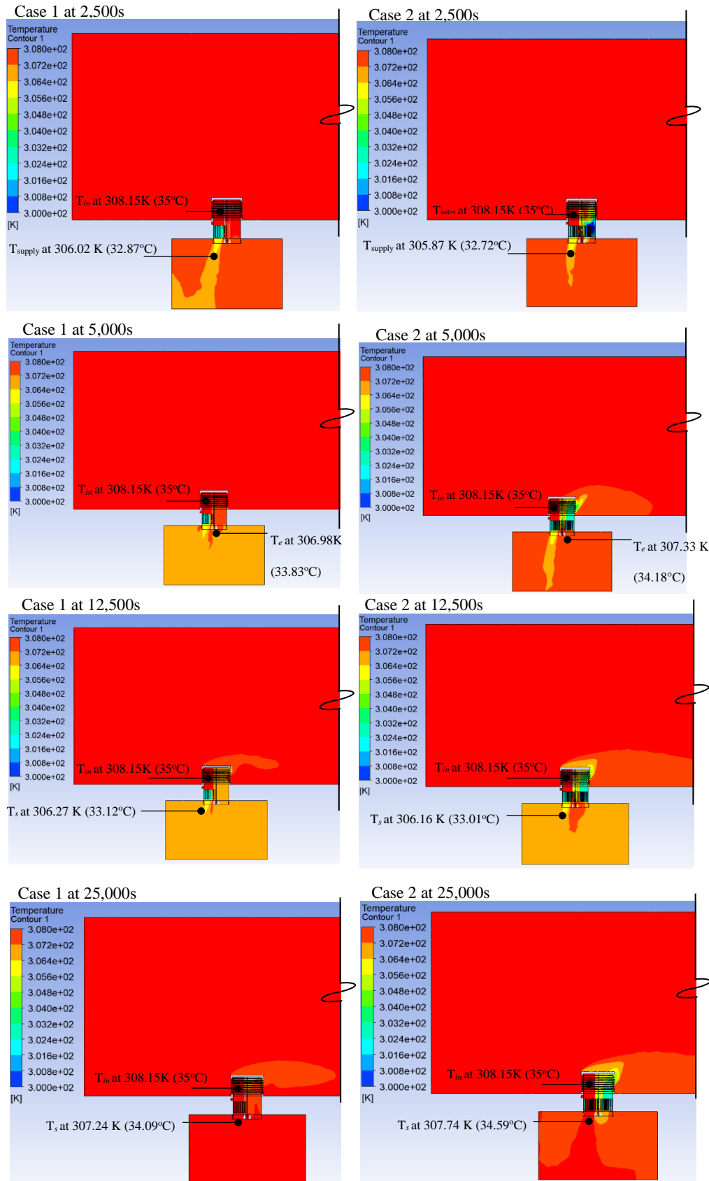
Figure 25. Air temperature contours showing exhaust ( T_e ) and supply ( T_s ) temperature variations from 2,500 s to 25,000 s based on the inclusion of E-PCM-T in the airstreams in Case 1 and Case 2.
