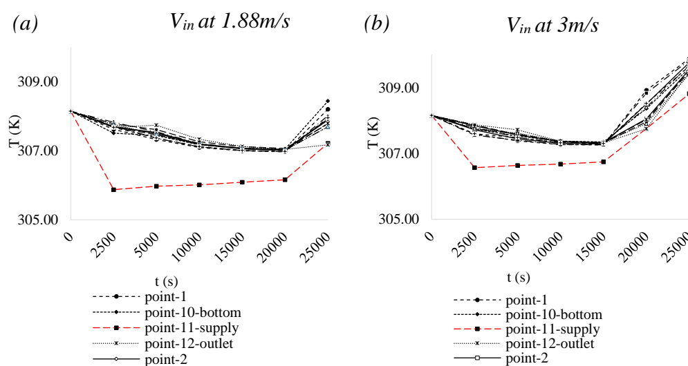
Figure 24. The air temperature T profile throughout the simulation flow time from 0 s – 25,000 s when (a) V_{in} is 1.88 m/s and (b) V_{in} is 3 m/s.
