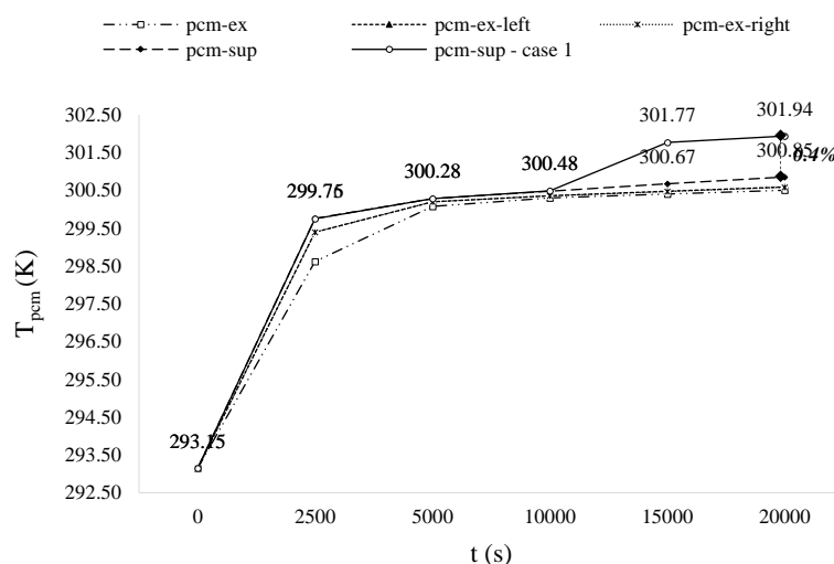
Figure 30. Comparison of PCM temperature T_{pcm} comparison for Case 1 and Case 2.
