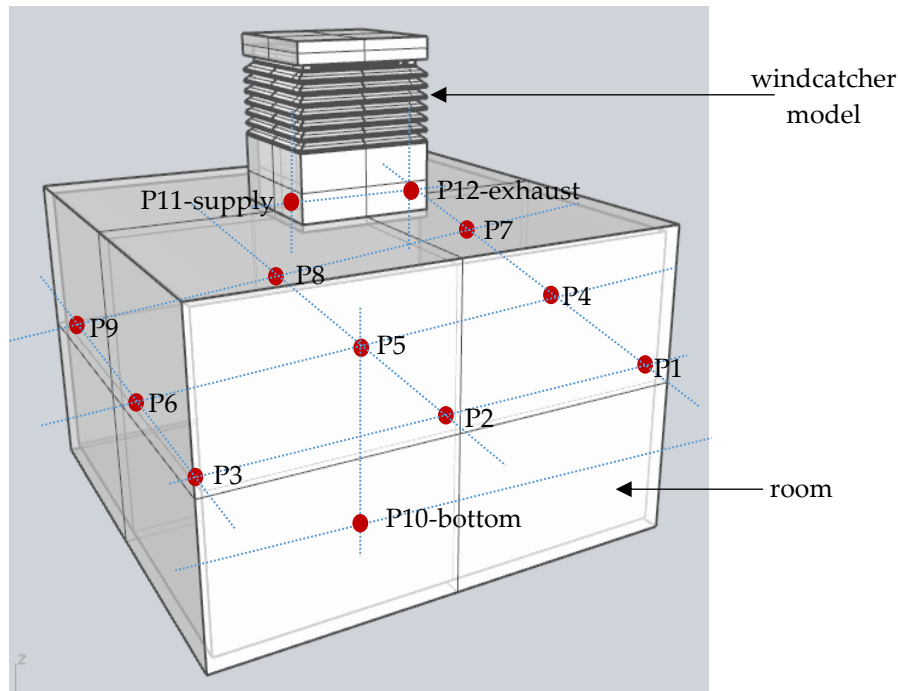
Figure 7. The twelve (12) monitored points where readings were taken throughout the windcatcher simulation study.
