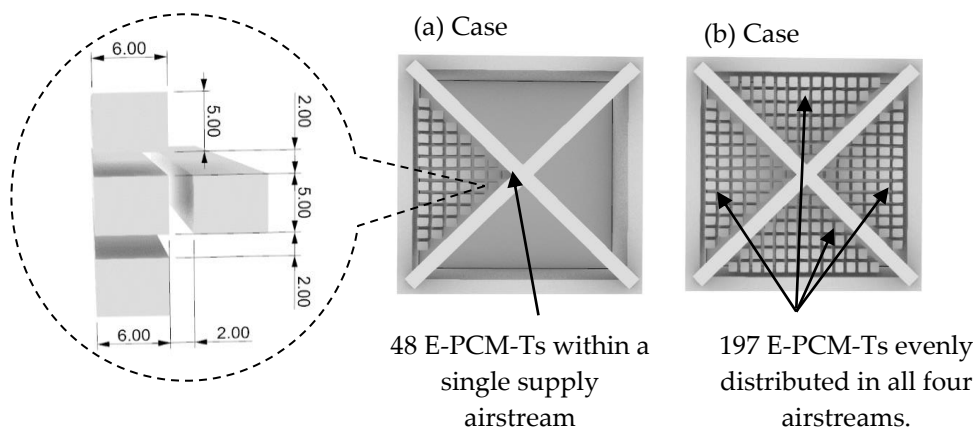
Figure 4. Two different arrangements of the E-PCM-Ts within the integrated windcatcher airstreams.
