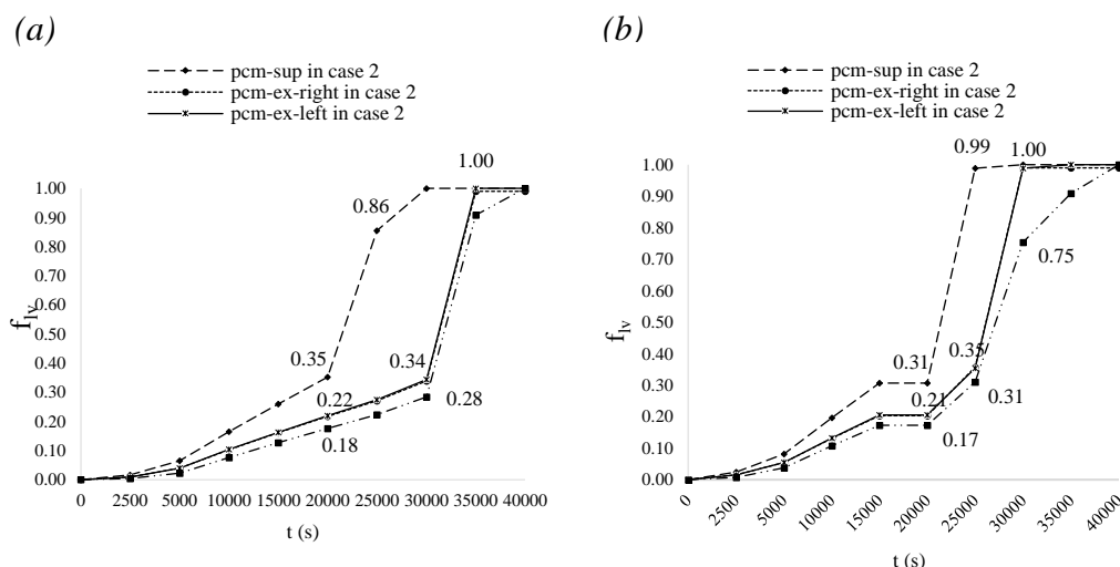
Figure 27. Effect of variation in V_{in} on PCM liquid fraction in Case 2 (a) when V_{in} is 1.88 m/s and (b) when V_{in} is 3 m/s.
