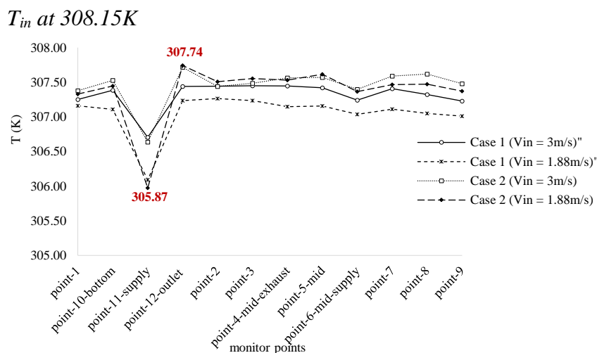
Figure 23. Comparison of air temperature T monitored at P_1 – P_{12} for Cases 1 and 2 at V_{in} of 1.88 m/s and 3 m/s after 1.4 hours of simulation.
