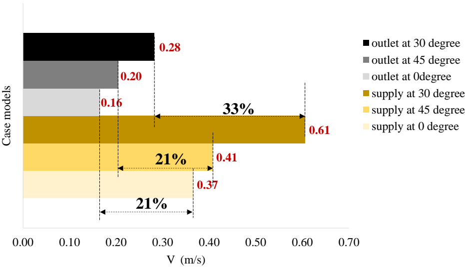
Figure 18. Comparison of the effect of different wind angles V_{\infty} on the supply and exhaust air velocities in the model.
