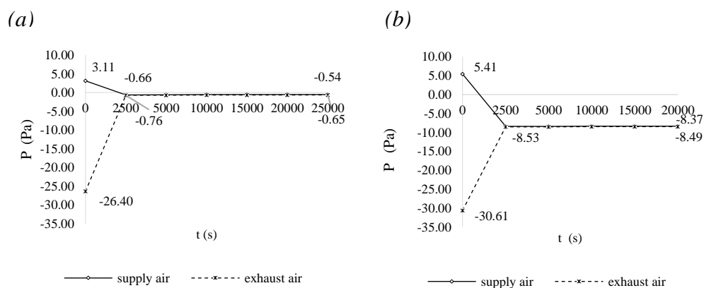
Figure 22. Air pressure P drops between supply and exhaust air at V_{in} is 1.88m/s at 0^\circ V_\infty : (a) Case 1 (b) Case 2.
