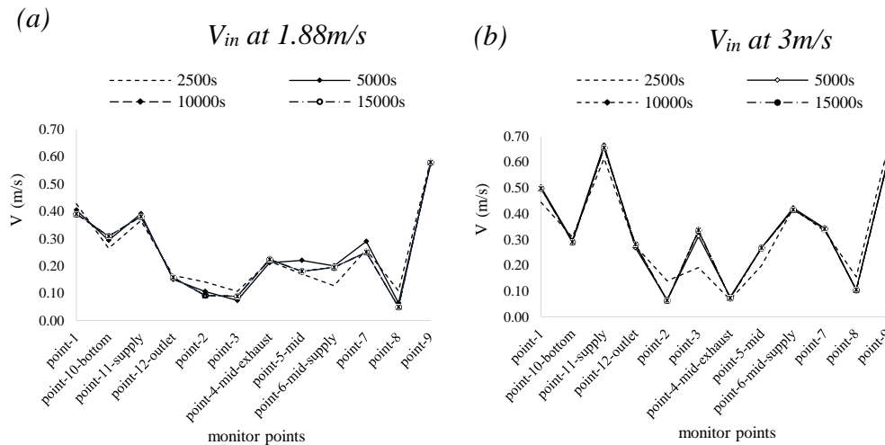
Figure 15. Air velocity profiles for Case 2 when V_{\infty} is 0^{\circ} at (a) V_{in} 1.88m/s and (b) V_{in} 3m/s.
