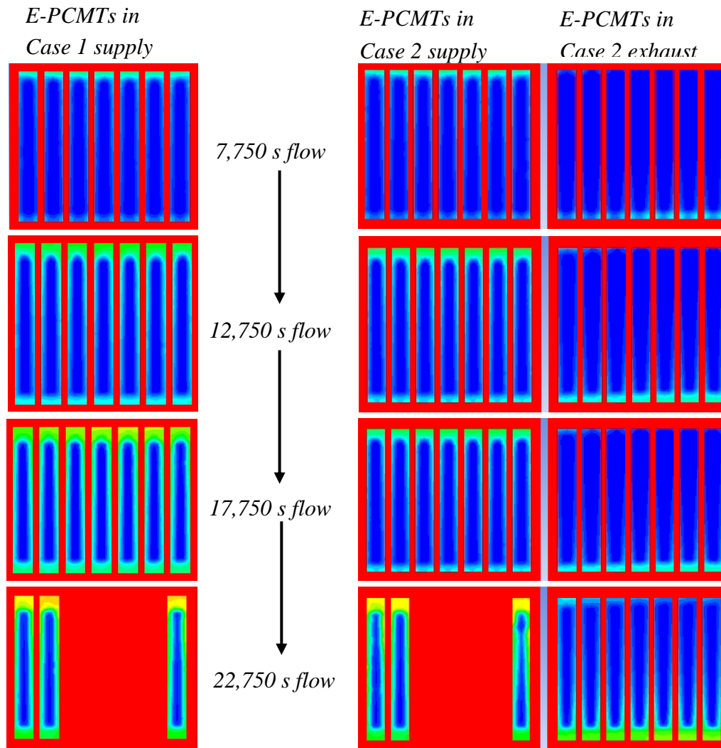
Figure 28. Contour showing PCM liquid fraction comparison between Case 1 and Case 2 based on the E-PCMT arrangement in supply and exhaust airstreams.
