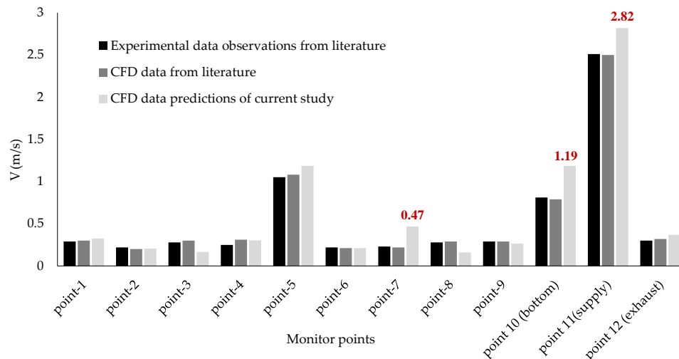
Figure 9. Comparison of indoor velocity CFD and experimental observation data showing C_p having the highest air flow discrepancy values at P_7 , P_{10} , and P_{11} -supply.
