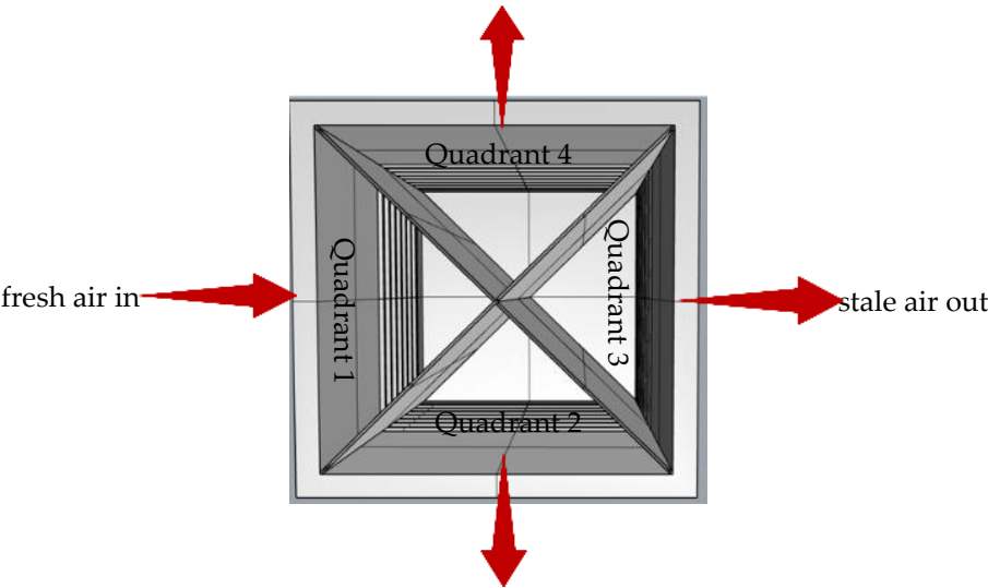
Figure 2. Cross-section of a four-sided multidirectional windcatcher showing airflow patterns through the X-shaped partitions/quadrants.
