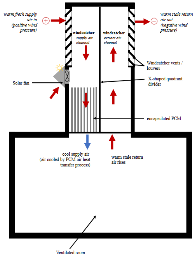
Figure 5. Airflow and cooling process in the hybrid windcatcher system.
