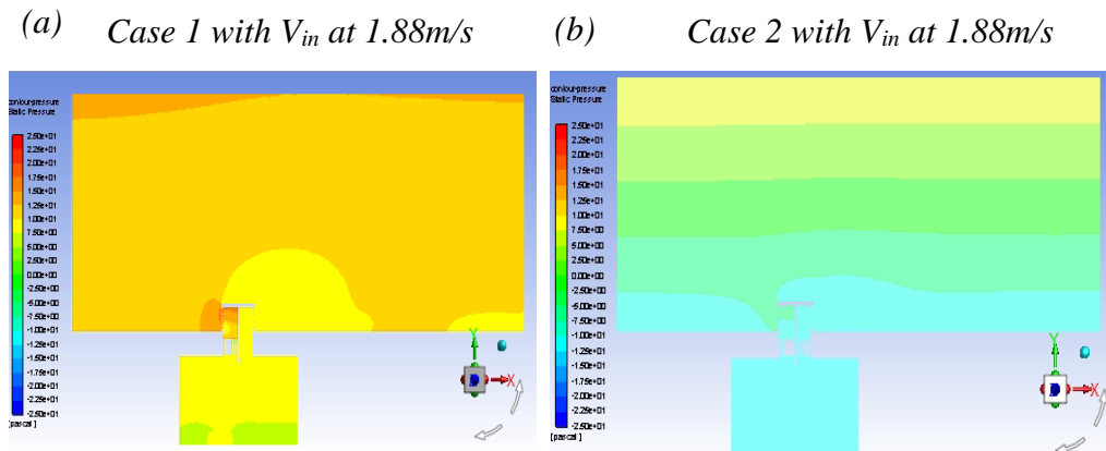
Figure 21. Air pressure contours show a comparison of the air pressure distribution comparison across a ventilated room in (a) Case 1 and (b) Case 2.
