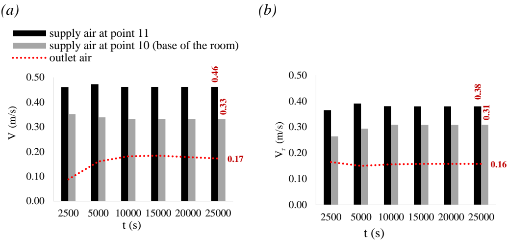
Figure 17. Comparison of air velocities at the supply, base of room, and outlet points when V_{in} is 1.88m/s for (a) Case 1 and (a) Case 2.
