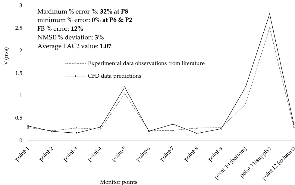
Figure 10. Comparison of indoor velocity CFD predictions ( C_p ) and experimental observation C_o data at P_1 - P_{12} -exhaust at 3 m/s outdoor wind speed showing the % deviation values.
