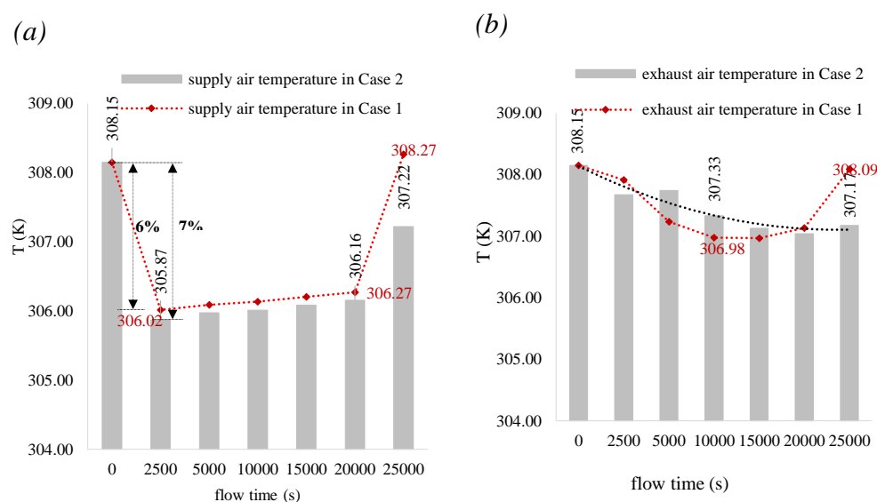
Figure 26. E-PCM-T arrangements' impact on temperatures—(a) Variation in supply air temperatures T_s for Case 1 and Case 2, and (b) Variation in exhaust air temperatures T_e for Case 1 and Case 2.
