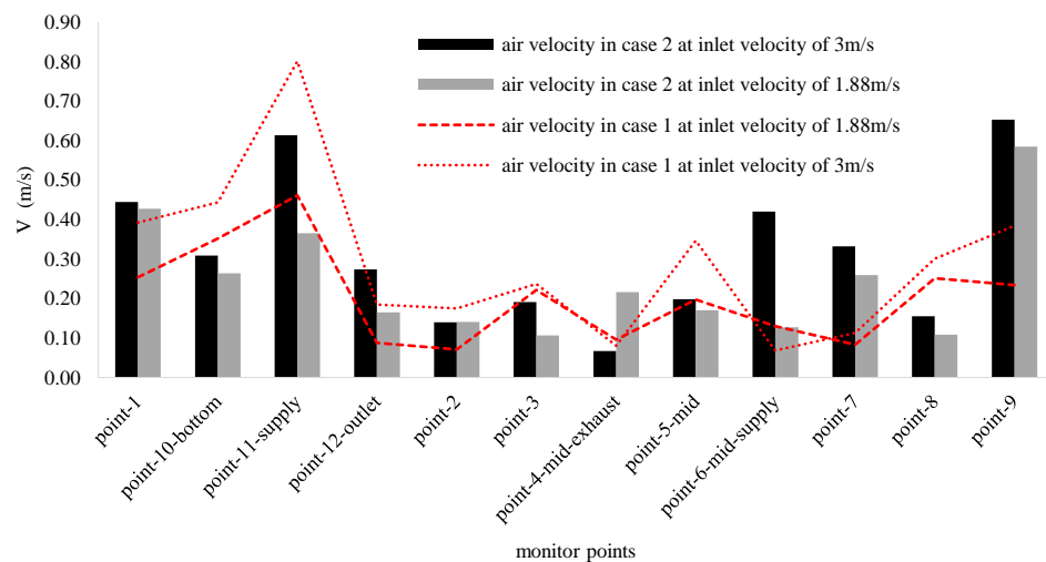
Figure 16. Comparison of air velocity variation in Cases 1 and 2 based on V_{in} 1.88m/s and 3m/s scenarios.
