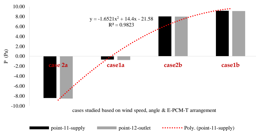
Figure 20. Air pressure comparison between four different windcatcher model cases based on varied V_\infty at 0^\circ and 45^\circ .
