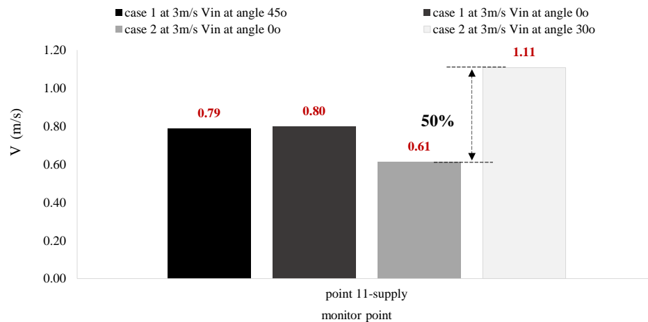
Figure 19. Comparison of the effect of wind angle V_\infty on the solar fan air flow performance on the windcatcher.
