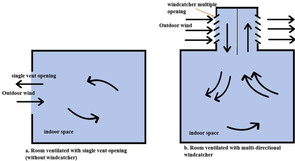
Figure 1. Airflow pattern comparison between single window opening and top-mounted windcatcher with multiple openings.
