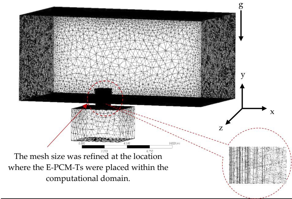
Figure 8. The computational grid is based on a non-uniform hybrid mesh.
