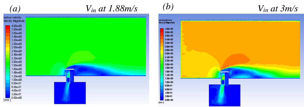
Figure 13. contour showing the variation in the air velocity magnitude in Case 1 when (a) V_{in} is at 1.88 m/s and (b) V_{in} is at 3 m/s.
