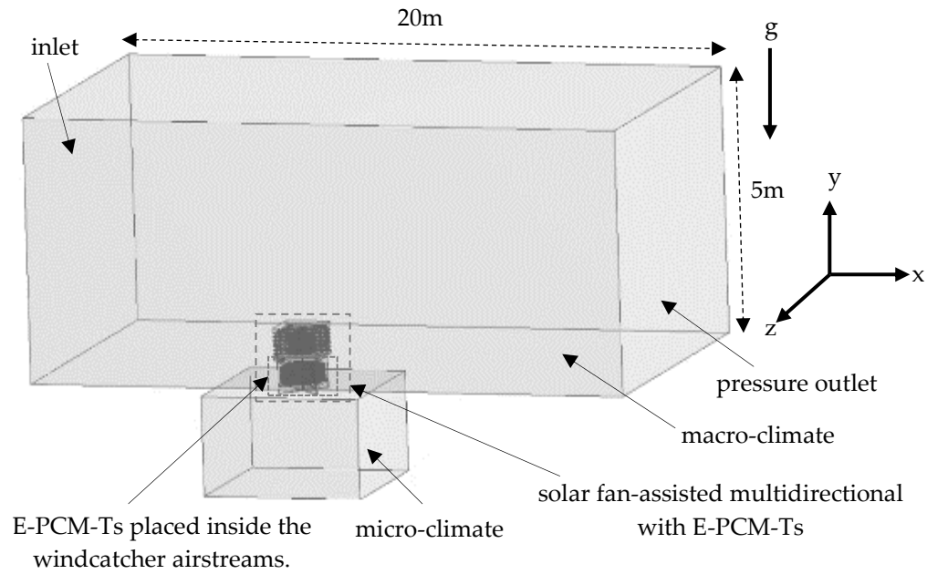
Figure 6. Computational domain and boundary conditions.
