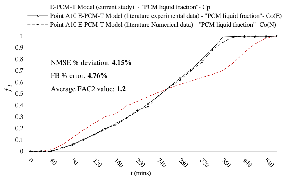
Figure 11. Validation of E-PCM-T Model – comparison of PCM liquid fraction CFD predictions C_p in the current study, experimental observations C_o(E) from the literature, and CFD predictions C_o(N) in literature.
