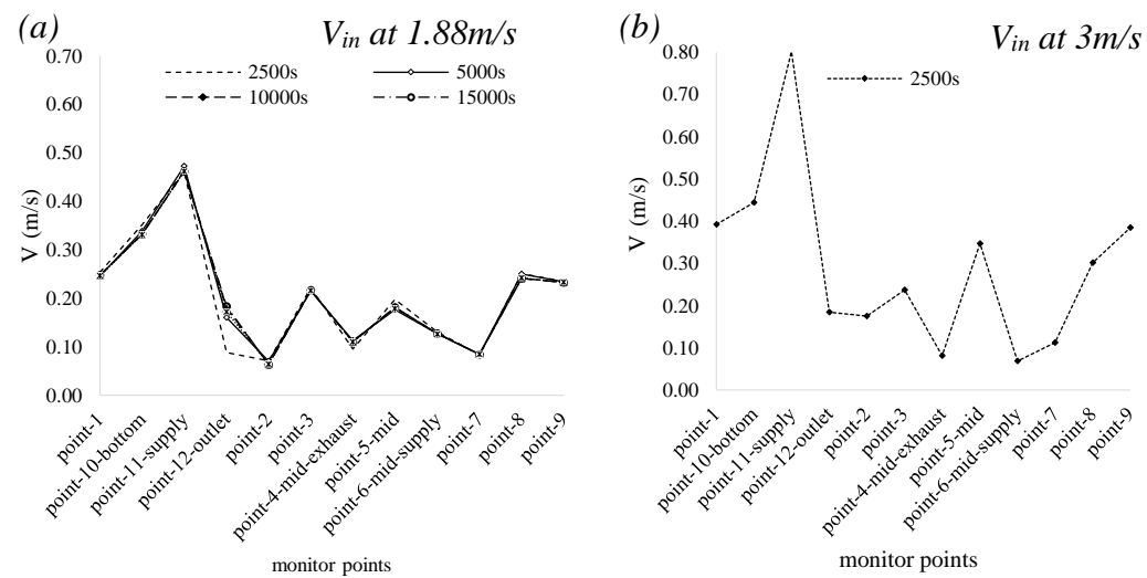
Figure 14. Air velocity profiles for Case 1 when V_{\infty} is 0^{\circ} at (a) V_{in} 1.88m/s and (b) V_{in} 3m/s.
