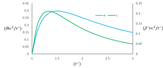
Figure 29. Release distribution and accretion luminosity.
