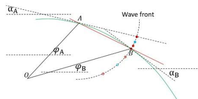
Figure 24. Probability of ballistic trajectory method for light deviation.
