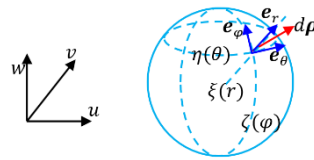
Figure 14. Covariant space.
