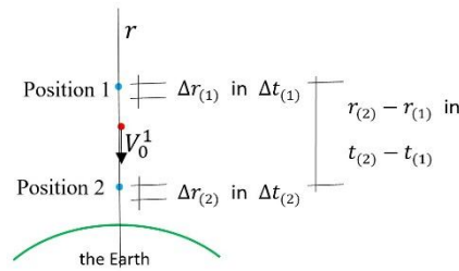
Figure 17. Free falling measurement.
