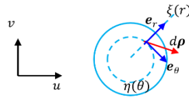
Figure 10. Covariant space.
