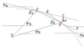
Figure 23. A diagram of ballistic method for a close-to-light-speed motion.
