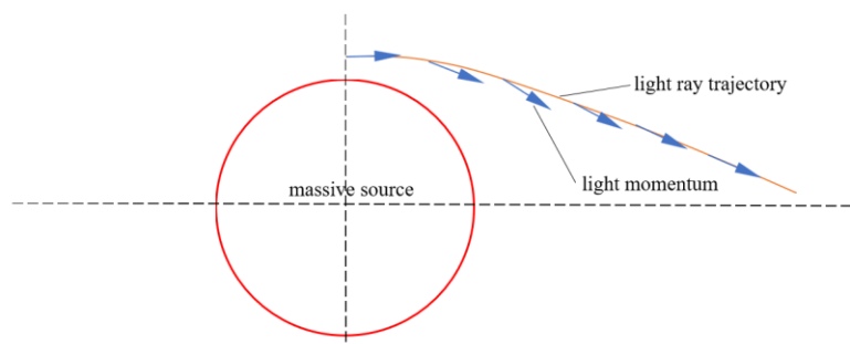
Figure 25. Light momentum vectors on the trajectory
