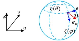
Figure 12. Covariant space.
