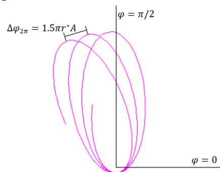
Fig. 22 The renovated trajectory of planet
