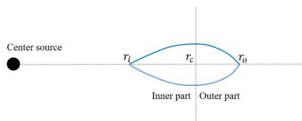
Figure 27. Driving condition with no shear motion in inner part.
