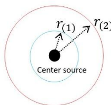
Figure 1. Center source field.
