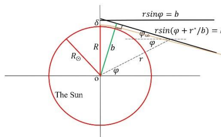
Figure 20. Asymptotic line with an overlapped \varphi_{\infty} .
