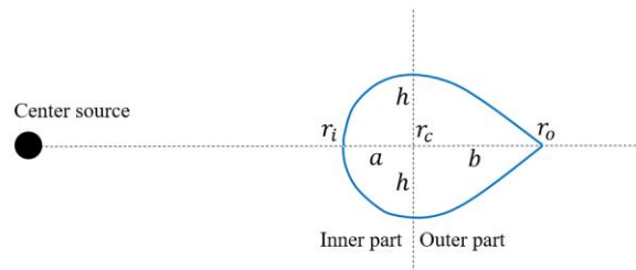
Figure 26. Fluid ring in one source field.
