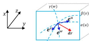
Figure 3. A super surface as covariant space in 3-dimensional space .
