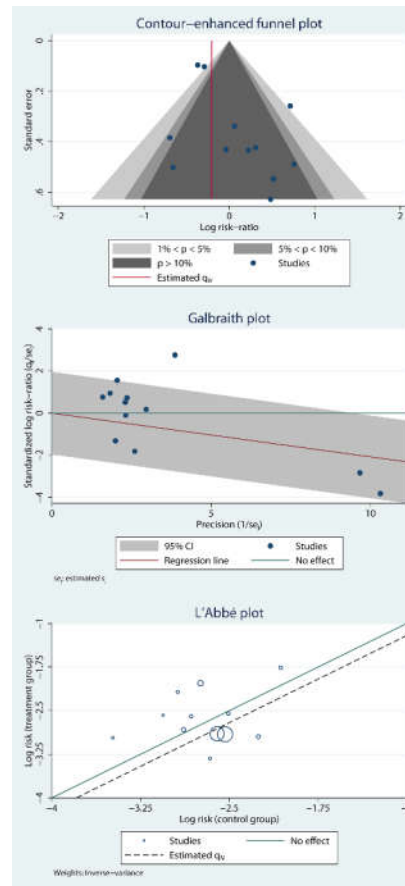
Figure 7. Top: contour-enhanced funnel plot assessing small-study effects and potential publication bias. Middle: Galbraith (radial) plot assessing overall heterogeneity and study precision. Bottom: L'Abbé plot illustrating between-study variability in event rates (heterogeneity exploration).
