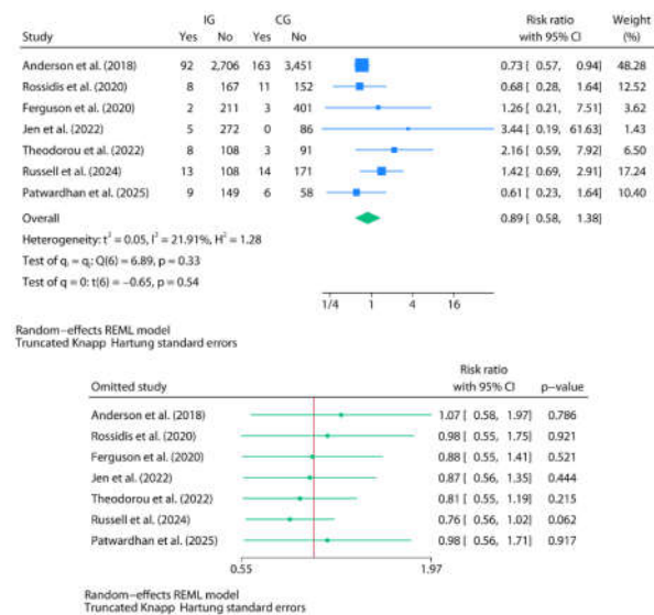
Figure 4. Top: Forest plot of the random-effects meta-analysis for surgical site infections (SSI) using REML with Knapp–Hartung adjustment (IG vs. CG). Bottom: Leave-one-out forest plot for the same analysis.
