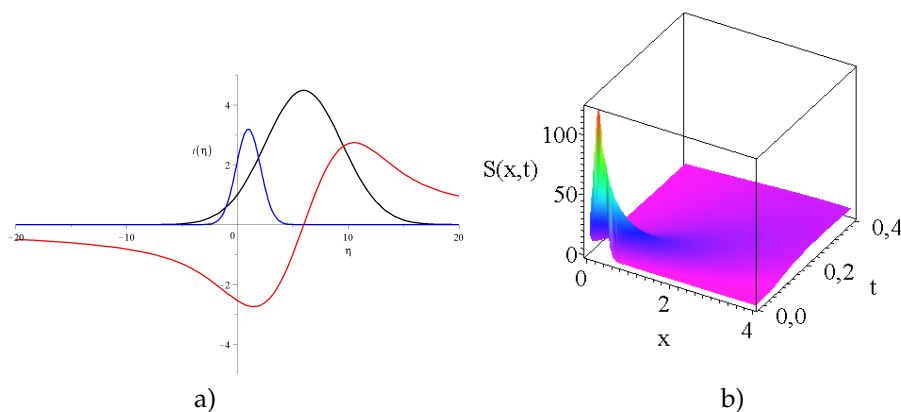
Figure 2. a) The shape functions of the salinity equation Eq. (15). The black and blue curves are for real part of the solution c_3 = 0 for the numerical parameters sets of (1, 3, 3) and of (2.1, 0.5, 0.3) for the parameters of (c_4, c, k_S) . The third red curve shows the imaginary part c_4 = 0 for the parameters of (1, 3, 3). b) Shows the projection of the real part of salinity distribution S(x, z, t) for z = 0 , with the parameters of (1, 3, 3), respectively.
