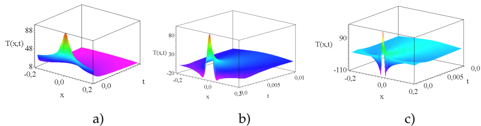
Figure 6. The Kummer's M part of the temperature distribution. The three figures from left to right have the source strength of (d = -1/3, 1/3, 2) the common parameters are k_T = c = 1 , respectively.
