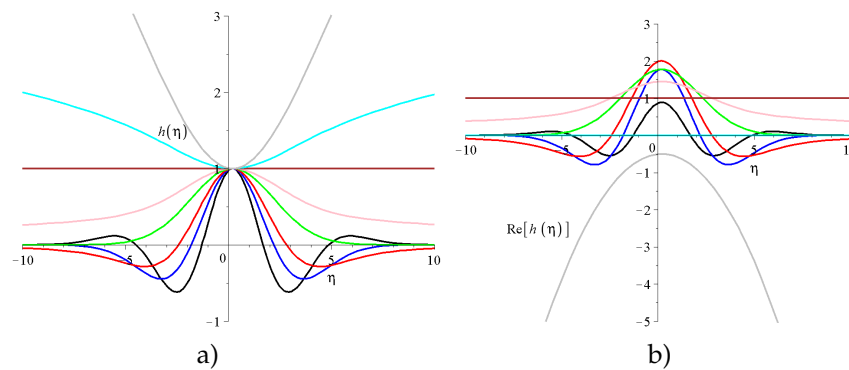
Figure 5. a) The Kummer's M part of the shape functions of the temperature Eq. (25). The common parameters are ( c_1 = 1, c_2 = 0, c = 0.1 and k_T = 1 ). The black, blue, red, green, pink, brown, cyan, gray lines are for numerical values of the source strength parameter d of (2, 1, 1/2, 0; -1/4, -1/2, -1, -3/2). b) The real part of the Kummer's U part with the same parameters.
