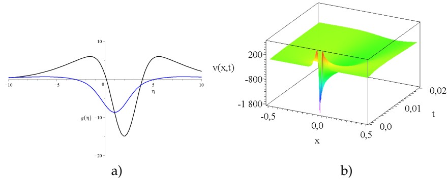
Figure 3. a) Two shape functions of the velocity equation Eq. (17). The common parameters are (G, c_2, c_4, c_6) are (10, 2, -6.2, 1) . The black and the blue curves have different values of the parameters (k_S, k_T, \alpha, \beta, \nu, c) namely (0.4, 1.3, 0.8, 38.18, 1) , and (0.4, 1.6, 5.3, 2.8, 8.18, 0.5) , respectively. b) The velocity distribution v(x, z = 0, t) with the parameters of the black curve, respectively.
