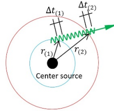
Figure 16. A photon traveling in center source field.
