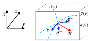
Figure 3. A super surface as covariant space in 3-dimensional space.
