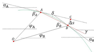
Figure 21. A diagram of ballistic method for a close-to-light-speed motion.
