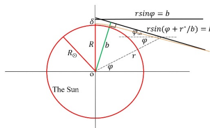
Figure 20. Asymptotic line with an overplayed \varphi_\infty .
