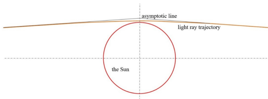
Figure 18. Light rays passing across the Sun.
