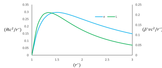
Figure 25. Release distribution and accretion luminosity.
