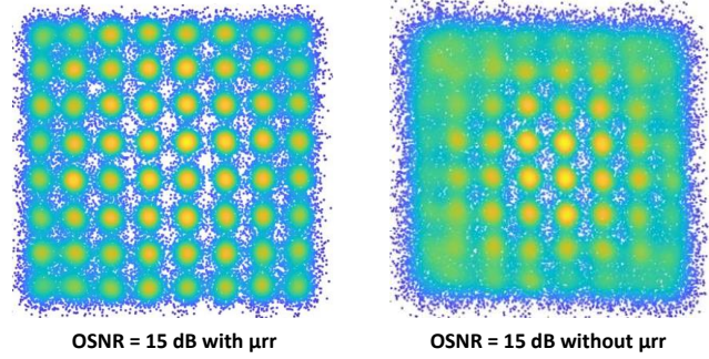
Fig. 9 Signal constellations as a results of distilled and bypassed carrier lines at OSNR = 15 dB.
