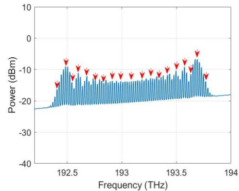
Fig.4 Electro-optic frequency comb after attenuation and amplification with the red arrows representing the lines used in the experiment.
