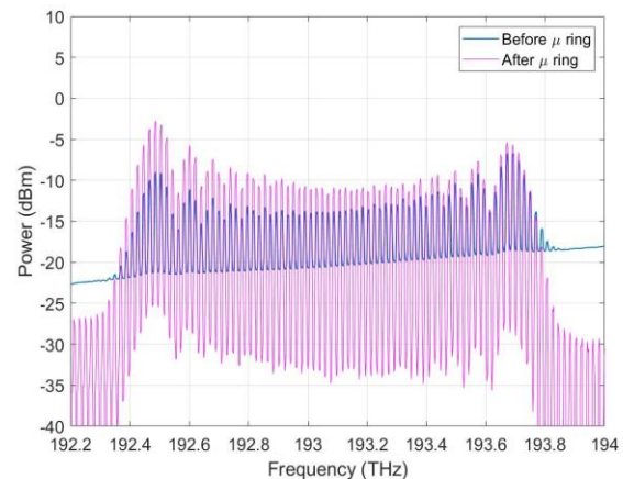
Fig. 2 Spectra for amplified (blue) comb before being distillation and distilled (magenta) EO comb.
