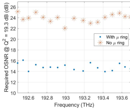
Fig. 7 Required OSNR at Q^2 = 19.3 dB, for both bypassed and distilled carriers against frequency of comb lines.
