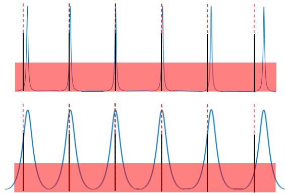
Fig. 15 Comb distillation by microring resonator with narrow bandwidth (top) and wide bandwidth (bottom) of resonances, where the comb lines are shown in black with noise floor in red and the equidistant grid is illustrated as the red dashed lines.
