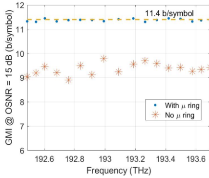
Fig. 8 GMI plot for distilled and bypassed carrier lines at OSNR of 15 dB with the limit of GMI = 11.4 b/symbol as indicated with the dashed line.
