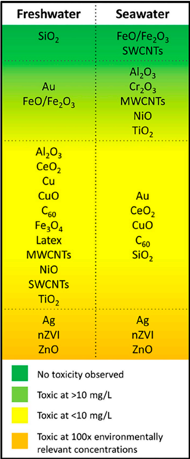
Figure 1. Toxicity of ENPs in freshwater and seawater [31].
