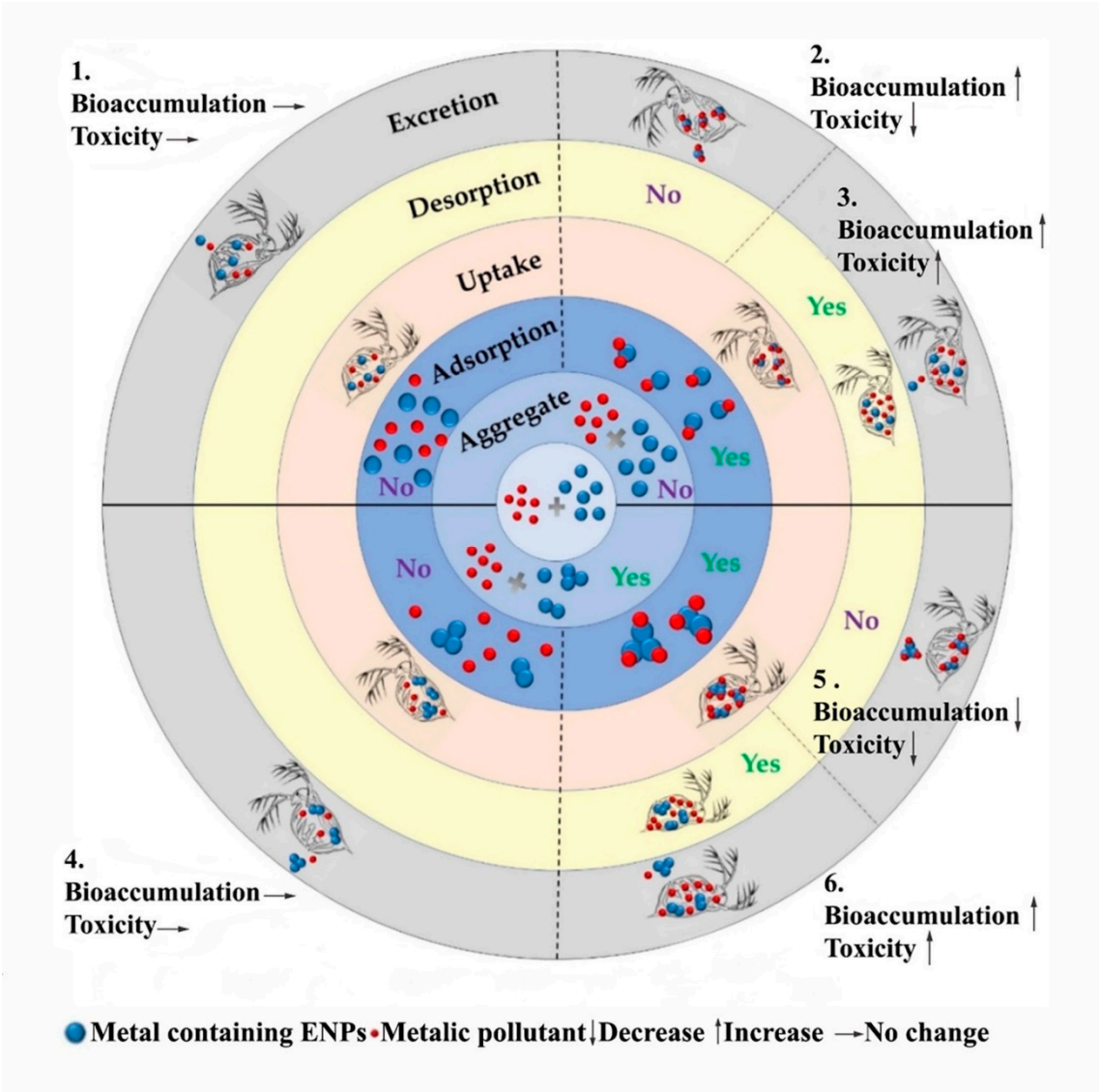
Figure 4. Conceptual demonstration of various situations regarding collective effects of combinations of metallic pollutants with ENPs and to environmentally significant aquatic species Daphnia magna [64].
