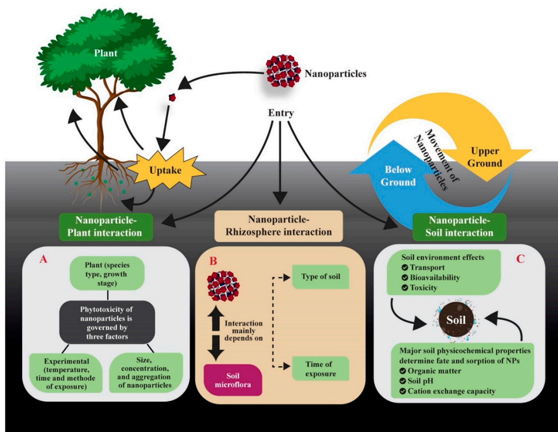
Figure 6. Interactions of ENPs with three elements of soil- (i) soil itself, (ii) soil microflora, & (iii) plants. NPs and Plant interaction (panel A) showed the three factors by which phytotoxicity of NPs is governed which are: (i) plant: species type and growth stage (ii) experimental: temperature, time, and method of exposure, and finally (iii) physicochemical characteristics of NPs, i.e., size, concentration, aggregation, and chemical
