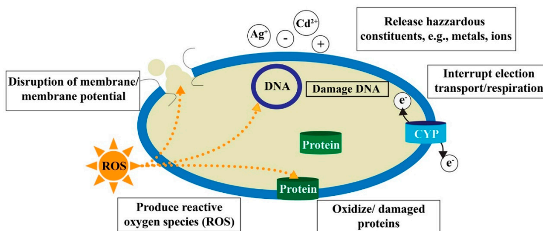
Figure 3. Schematic of toxic behavior of ENPs in bacteria.
