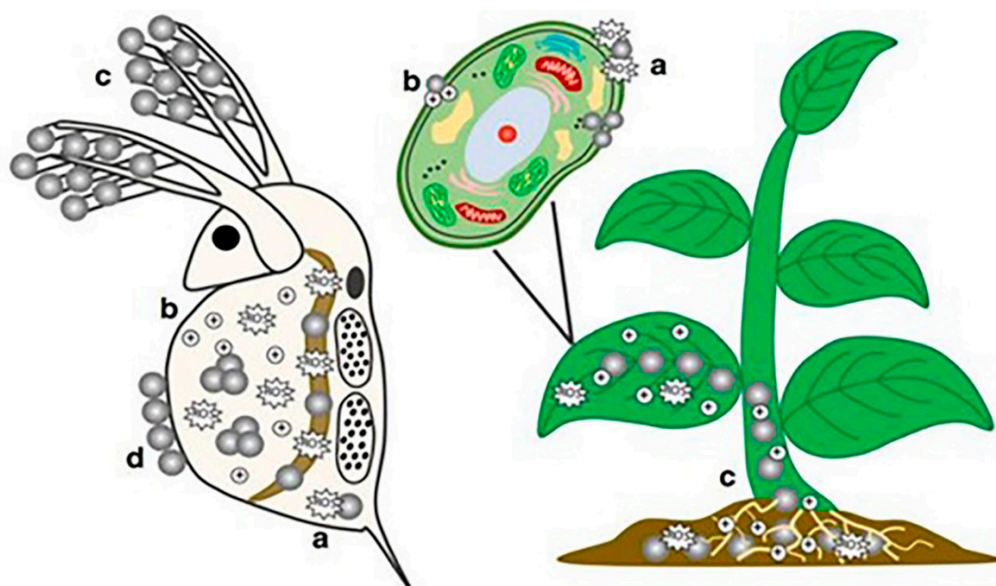
Figure 2. Ecotoxicity of ENPs in aquatic and terrestrial regimes, showing the mechanisms as a) formation of ROS, b) ion release, c) internalization, and d) biological surface coating [38,39].
