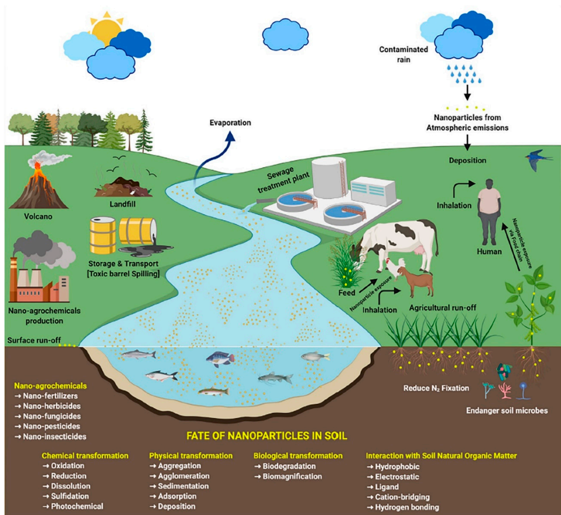
Figure 5. Illustration of the fate of ENPs in Soil-Plant Systems [76].
