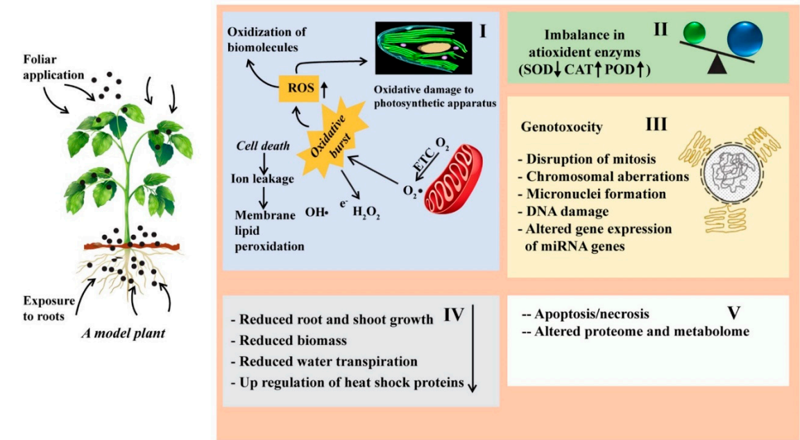
Figure 7. Toxic effects of ENPs on the plant through ROS generation, peroxidation of the lipid membrane, and damage of mitochondria and chloroplasts (Panel-I). Oxidative stress creates an imbalance in enzymes (Panel-II); interaction of NPs with plant cells causes genotoxicity through disruption of the usual cell cycle, generation of micronuclei, anomalies of chromosomal, etc. (Panel-III). Disturbing effects of NPs on plants contain biomass reduction and water transpiration etc. (Panel-IV); interaction of NPs with cells of plant results in necrosis, apoptosis, and change in metabolome and proteome (Panel-V), which eventually lead to the death of plant cell. [85].
