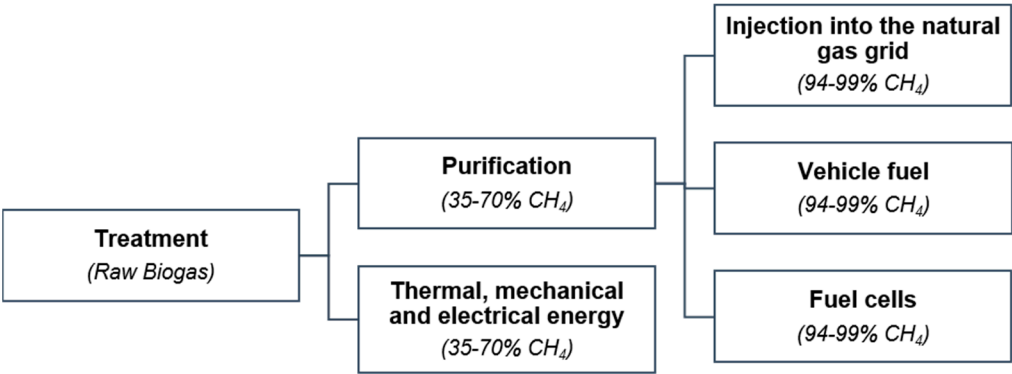
Figure 2. Biogas treatment and purification steps for biomethane concentration according for its final use, based on [41].
