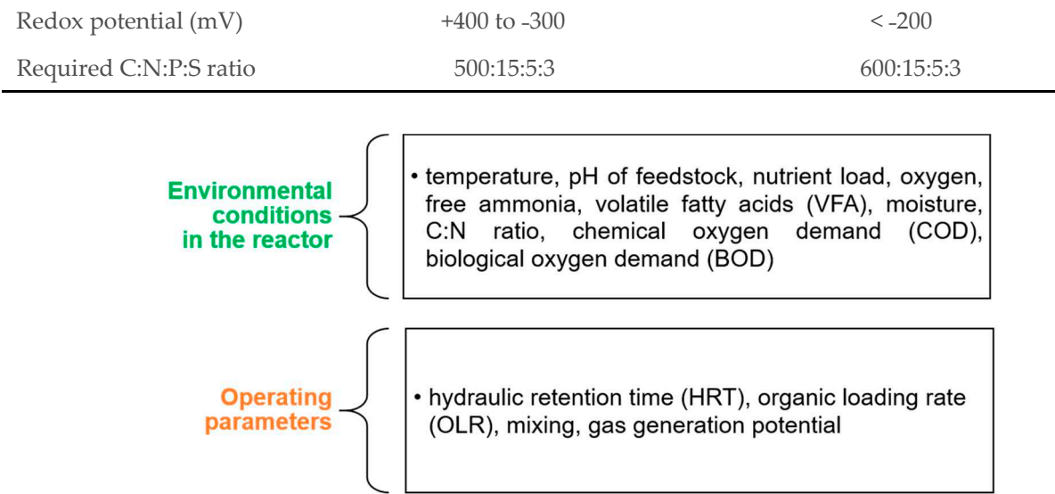
Figure 1. The scheme of main conditions affecting anaerobic digestion (VFA – volatile fatty acids, C:N ratio – carbon:nitrogen ratio, COD – chemical oxygen demand, BOD – biological oxygen demand).
