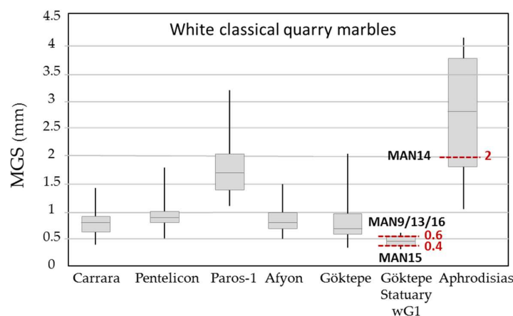
Figure 6. Maximum Grain Size (dashed red line) of the white sculptural marbles studied from Valdetorres de Jarama collection Fine-grained marbles (samples 9, 13 and 16) and Extremely fine (sample 15) are compared to the MGS of the most important fine-grained marbles of statuary quality. Both types are associated to the wG1 statuary white Göktepe. Medium to Coarse-grained marble (sample 14) is discussed in section 3.4.2.
