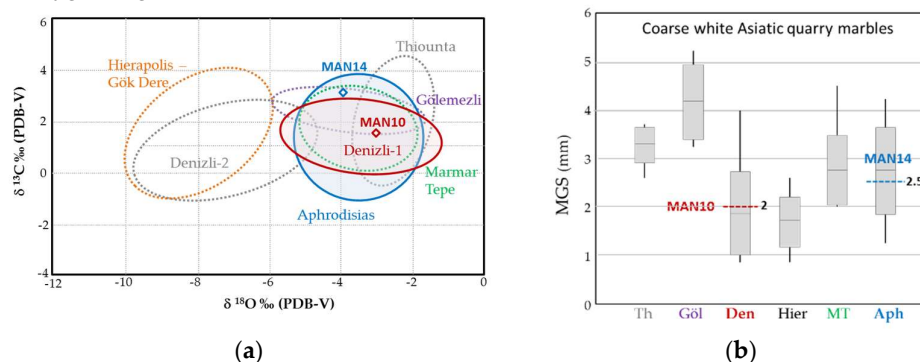
Figure 9. Analytical diagrams referring to Anatolian quarries with medium-coarse-grained white marbles (Caria and Phrygia regions): Th (Thionta), Göl (Gölmezezi), Den (Denizli), Hier (Hierapolis-Gök Dere), MT (Marmar Tepe), Aph (Aphrodisias). (a) isotopic diagram; (b) grain size diagram (MGS) [40–42].
