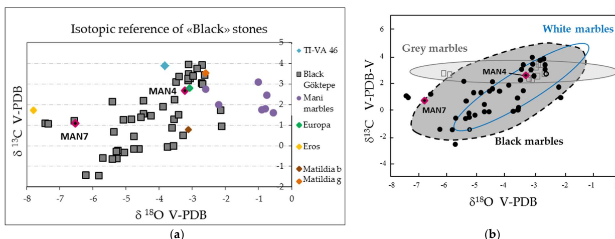
Figure 3. Isotopic signature of “Black”, Dark Grey samples (MAN4, MAN7), from Valdeterres de Jarama in two isotopic diagrams, in red symbol; (a) In the isotopic diagram of data of two different quarries of Black and some important archaeological pieces to compare [24,37]; (b) In the general isotopic diagram for Göktepe quarries [27 and references therein].
