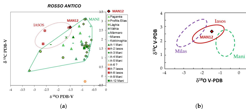
Figure 5. Isotopic signature of the red marble under study (MAN12). (a) In the diagram for Iasos and Mani quarry red marbles and twelve archaeological artifacts (A-1 to A-12) from literature [38]; (b) In the isotopic diagram proposed in [39] which includes both Carian red from Milas and Iasos.
