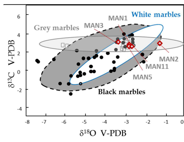
Figure 4. Isotopic signature of Light Grey samples in red symbol (MAN1, MAN2, MAN3, MAN5, MA11) from Valdeterres de Jarama in the general isotopic diagram for Göktepe quarry marbles [1,4,27].
