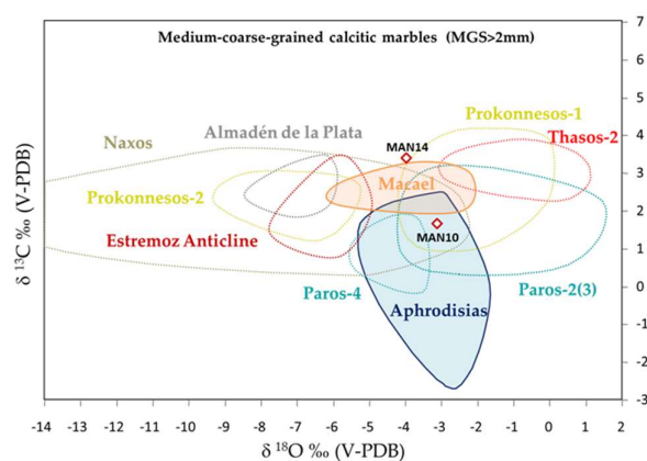
Figure 8. Isotopic signature of the archaeological samples (in red) plotted on the general isotopic diagram for medium-coarse-grained marbles modified from [43] with data of Hispanic marbles: Estremoz Anticline, Almadén de la Plata and Macael [31,32]. The hypothetical idea of a local marble being used in the bases of the figures (sample 10) must be completely ruled out, not only by isotopes but also by petrography and CL. On the contrary, its assignment to the marble from the city of Aphrodisias, although isotopically compatible, must be
