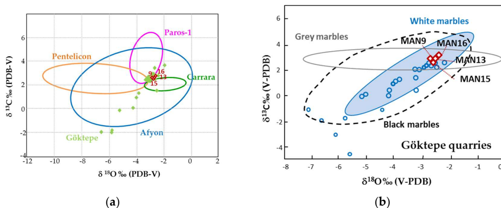
Figure 7. Isotopic signature of the archaeological samples (in red) of fine-grained white marbles plotted on two different isotopic diagrams; (a) Isotopic diagram with the 90% probability ellipses of the most important classical marbles [40] with the data points of white Göktepe quarry marbles [10]; (b) Scatterplot of the C and O isotopic values of the white Göktepe quarry marble with its 90% probability ellipse (in blue) adapted from [27] and papers therein.
