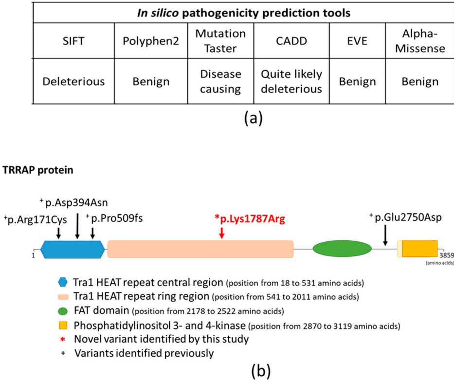
Figure 8. (a) Pathogenicity prediction of the novel variant using in silico tools and (b) location of the newly identified variant on the TRRAP protein.
