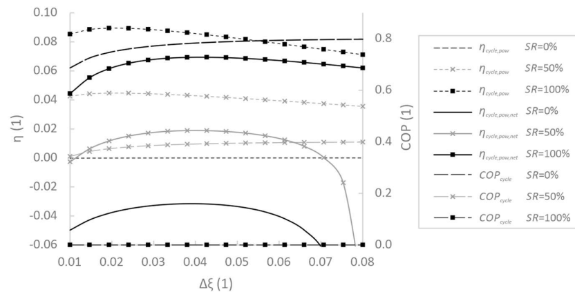
Figure 6. COP and gross and net APCC system efficiencies at varied concentration differences.
