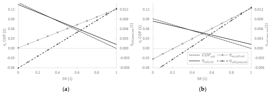
Figure 7. Energy and exergy efficiency and COP for heat source utilization with respect to the splitting ratio, for APCC (a) and ORC-VCC (b).
