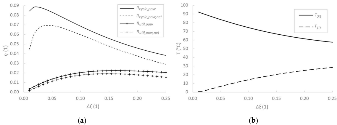
Figure 9. APC system ( SR = 1 ) parameters at varied concentration difference for higher heat recovery from the heat source: cycle and utilization efficiency (a) and heat source outlet and evaporator temperature (b).
