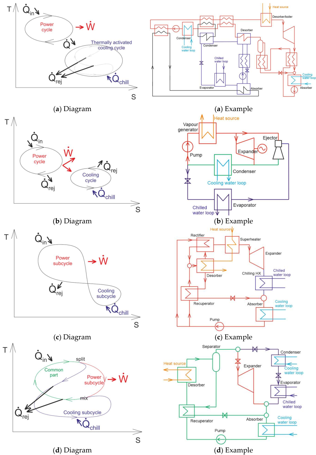
Figure 1. Schematic process diagrams of combined power and cooling systems with: (a) two separate cycles coupled by heat [18], (b) two separate cycles coupled by work [19], (c) single-branch thermodynamic cycle [11], and (d) two-branch thermodynamic cycle [20]
