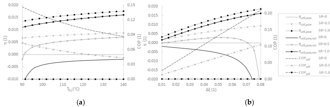
Figure 8. Utilization COP and gross and net APCC system efficiencies at varied heat source temperature (a) and varied concentration difference (b).
