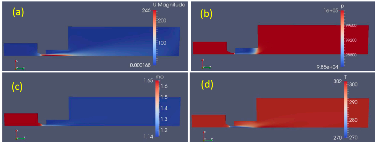
Fig. 3: (a) The field of gas velocity magnitude |U| (m/s), (b) pressure p (Pa), (c) gas density \rho (kg/m 3 ), and (d) gas temperature T (K) for the nominal case configuration at Q = 1200 sccm.
