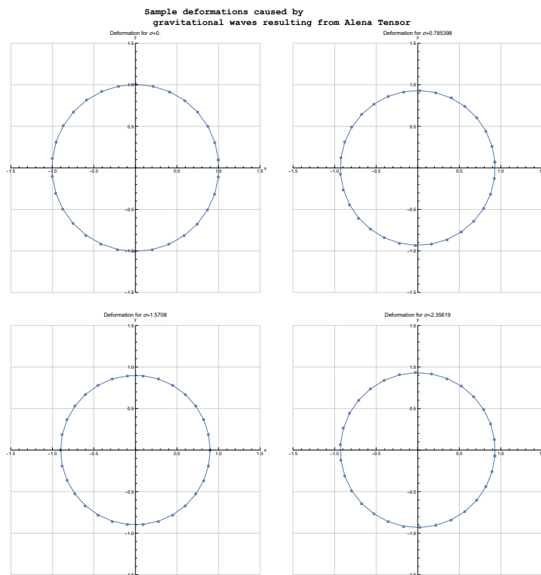
Figure 3. Deformation visualization for particles on a circle.
