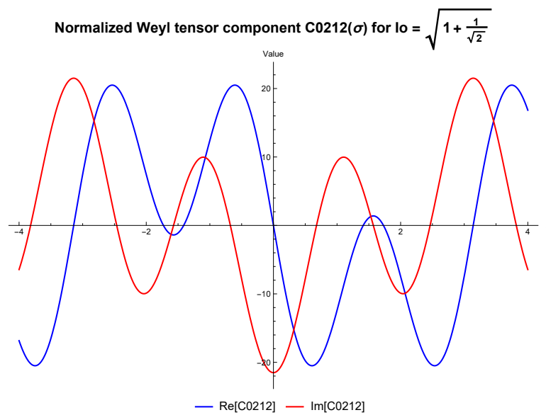
Figure 2. Weyl tensor C^{0212} component as a wave.
