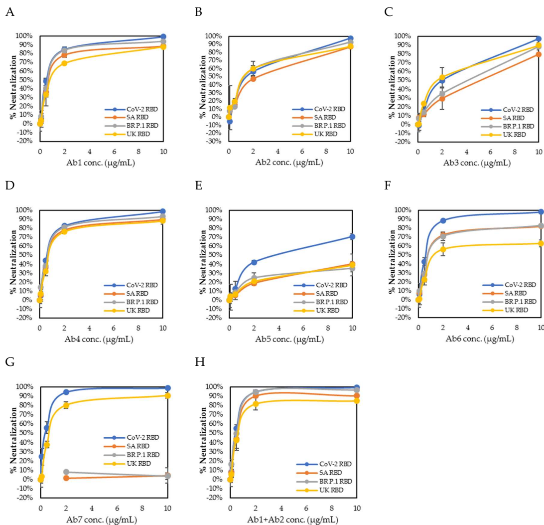
Figure 6. Neutralization kinetics by lateral flow cassette neutralization assays. (6A-6G) Kinetic curves for individual antibodies against the four RBDs. (6H) Kinetic curve for the combined two antibodies against the four RBDs.
