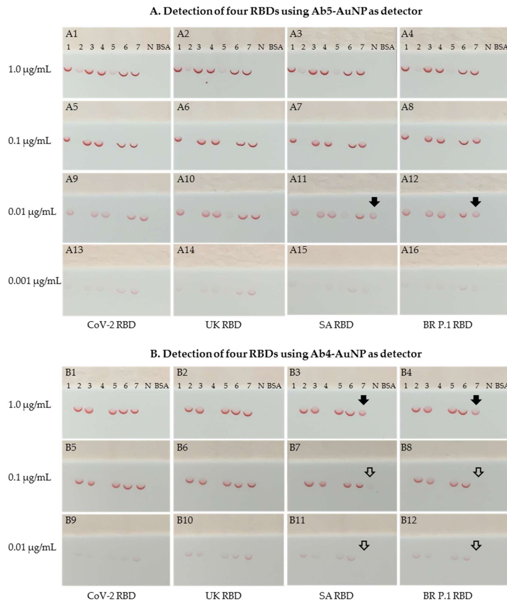
Figure 4. Comparative binding characteristics to four RBDs using Ab4-AuNP and Ab5-AuNP as detectors. Representative photographs of test results. (A) Binding behavior of Ab5-AuNP conjugate to four RBDs. (B) Binding behavior of Ab4-AuNP conjugate to four RBDs. (Note 1) Solid arrow in dipsticks (A11, A12, B3, B4) indicates similar signal intensity at Ab7 spot. Open arrow in dipsticks (B7, B8, B11 and B12) indicates very faint or invisible signal at Ab7 spot. (Note 2) Both Ab4-AuNP and Ab5-AuNP conjugates were coated at 20 µg antibody per mL 20 OD AuNP solution.
