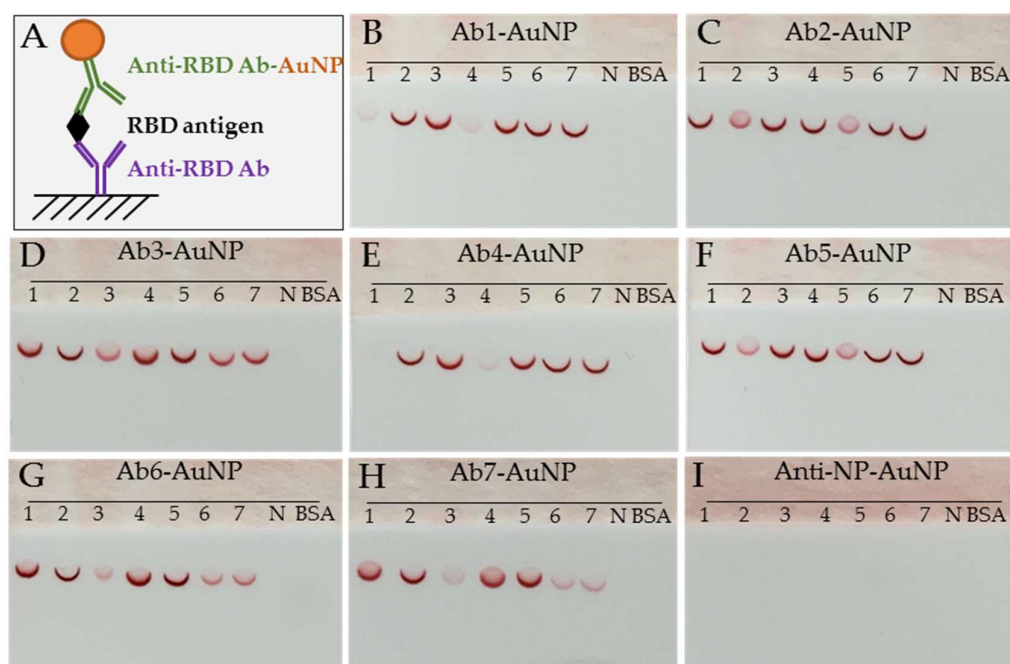
Figure 3. Antibody pairing capability and epitope binning. (3A). Sandwich immunoassay principle. (3B-3I). Photographs of a representative set of lateral flow dipstick assays. Each dipstick has 9 spots: 7 spots for the antibodies of interest, and 2 spots for negative controls (anti-NP antibody and BSA). ( Note 1 ). A dark red colored crescent line or circular spot indicates strong binding activity, a light red colored crescent line or circular spot indicates weak
