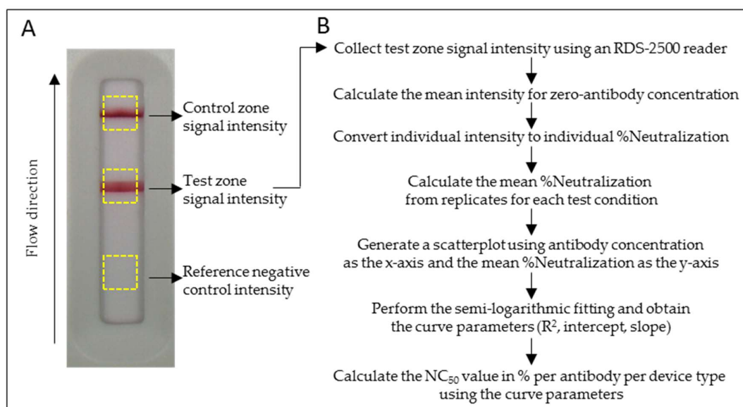
Figure 2. Collection of signal intensities and flowchart for the calculation of NC_{50} values from the test line signal intensity. (A) An example of test cassette image recorded by the RDS-2500 LFA reader with designated zones for collection of signal intensities. (B) Flowchart for the calculation of the NC_{50} value for each neutralization kinetic curve.
