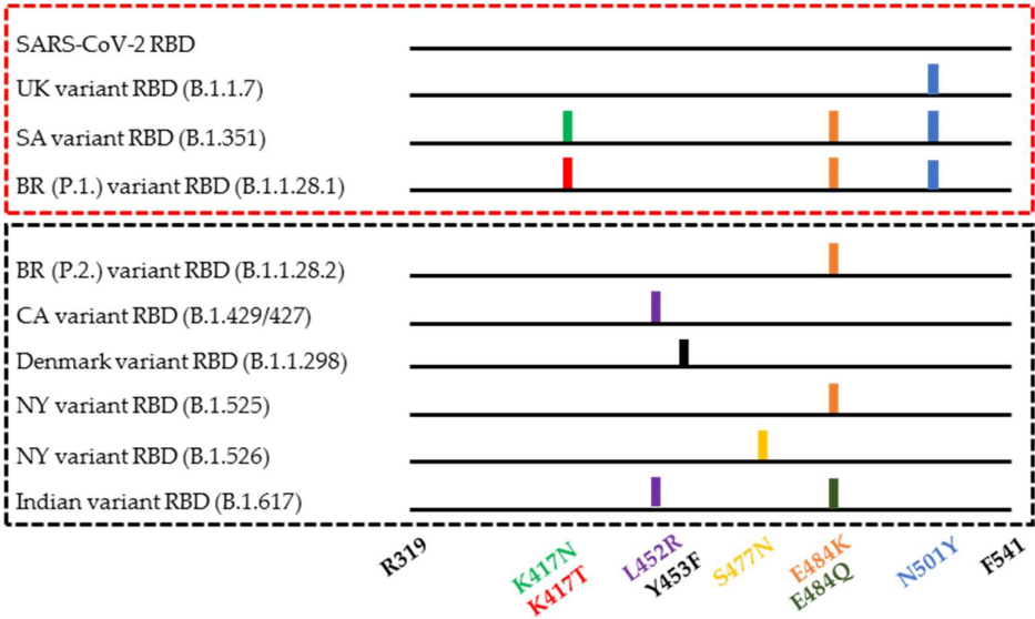
Figure 1. Mutations in the spike RBD protein of currently circulating SARS-CoV-2 variants [2-10]. (Top panel) Variants included in this study. (Bottom panel) Variants not addressed in this study.
