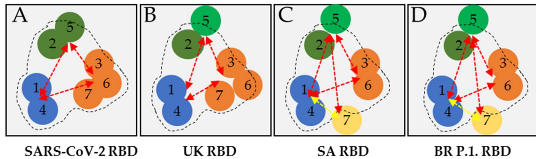
Figure 7. Functional arrangement map of the antibody pairing capability and neutralizing activity. ( Note 1 ) Blue circle – Epitope bin A antibodies (Ab1 and Ab4); Green circle - Epitope bin B antibodies (Ab2 and Ab5); Orange circle – Epitope bin C antibodies (Ab3, Ab6, and Ab7). ( Note 2 ) Red double-headed arrow indicates antibody pairing with strong detection capability; Yellow double-headed arrow indicates antibody pairing with weakened detection capability. ( Note 3 ) Black dotted line indicates the neutralization functionality – if inside the dotted line, strong neutralization activity; if on or outside the dotted line, weak or no neutralization activity.
