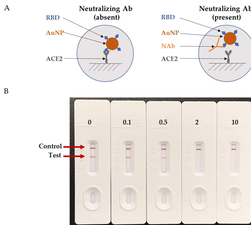
Figure 5. Neutralizing antibody test principle and images of representative test devices. (A) Lateral flow cassette neutralization assay principle. (B) Photographs of a representative set of lateral flow neutralization test devices. (Units = neutralizing antibody concentration in \mu\text{g/mL} ).
