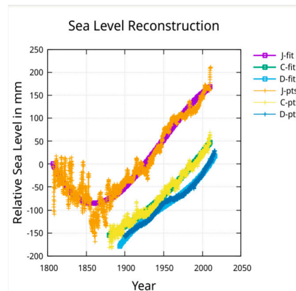
Figure 7. The fits to the reconstructions are shown here with the approximate 60-year period removed from the fit.
