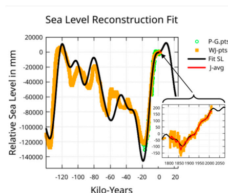
Figure 1. Here is shown the last 140,000 years of relative sea-level information, WJ-pts fit with a constant and functions associated with 11 periods related to planetary orbital cycles (Fit SL, black, negative years are BCE dates). The peak at 12.2 meters is in the year 9,726 or 7,700 years into the future. Note that the peak at -119,600 is at 10.75 meters. The inset plot (see Figure 13 for details) shows how the fit matches with the Jevrejeva et al. [12] reconstructed sea-level data, 1807 to 2010 relative to 1930. The J-avg curve (red) is a 10-year running average over these years. The P-G-pts are proxy sea-level information from Physical Geology [6] and not input to the fit – see Appendix.
